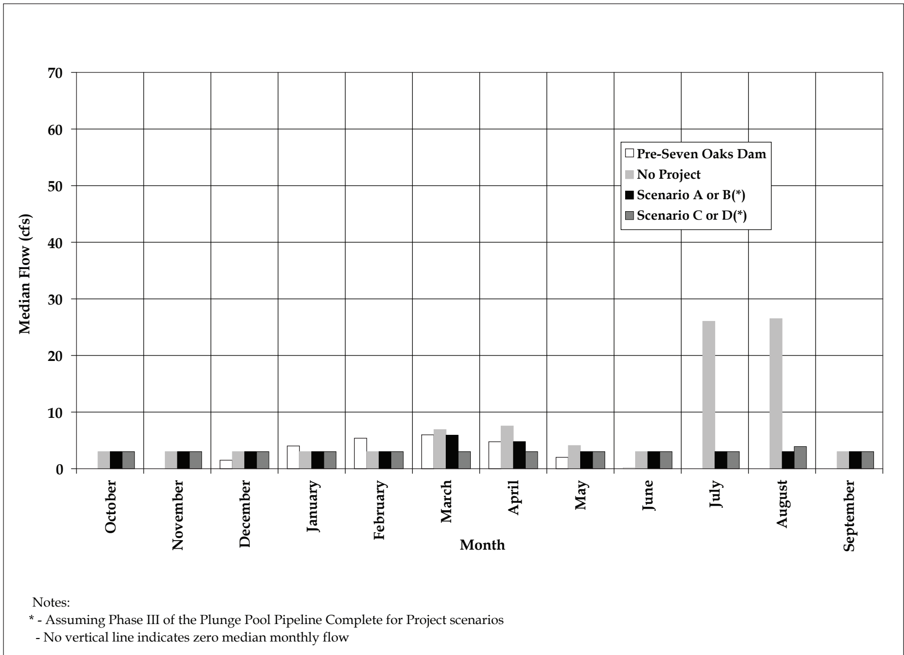
Figure 6.2-2. Median Monthly Flows (Non-Storm Days) for SAR Segment B, just above Cutter Weir, WY 1966-67 through WY 1999-2000
