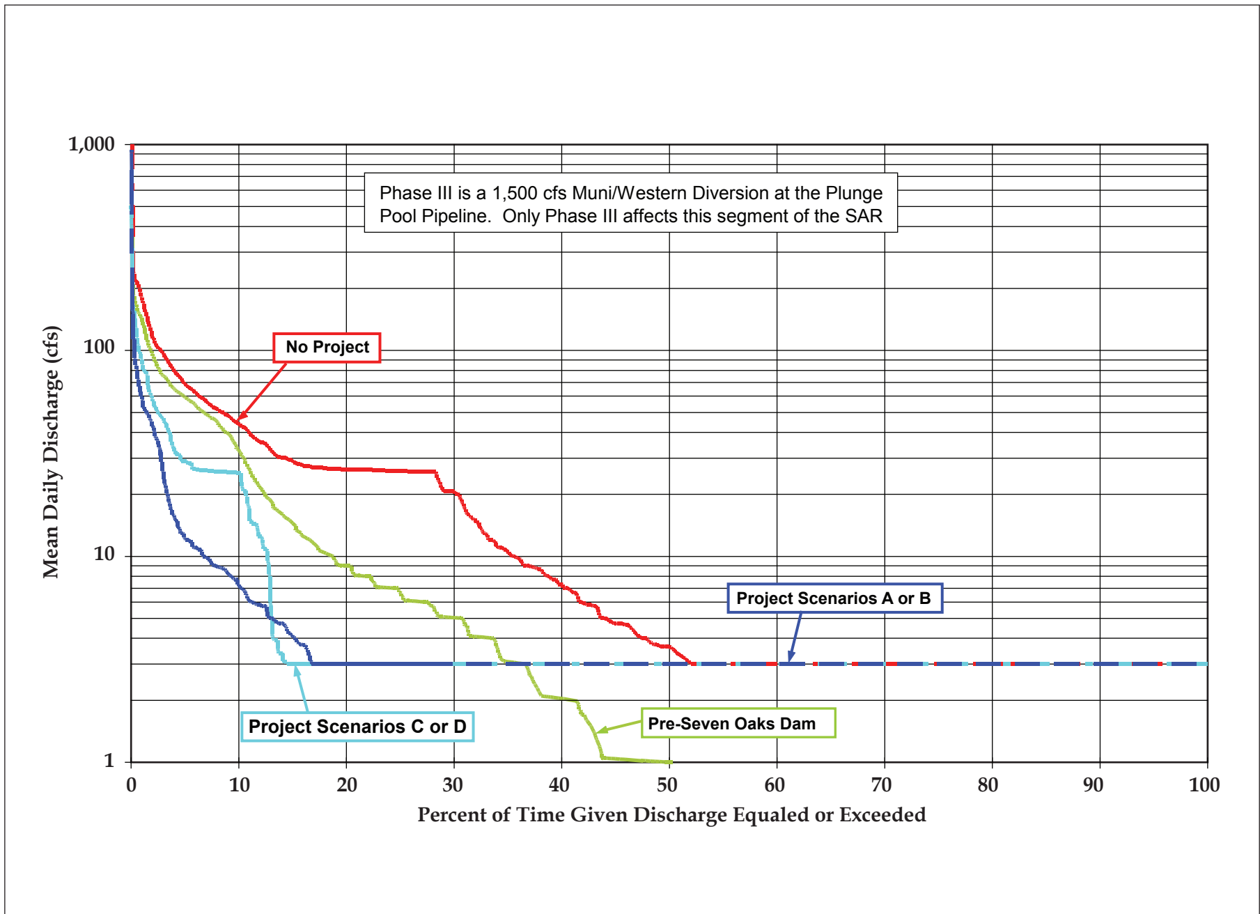
Figure 6.2-8. Probability of Daily Discharge (Non-Storm Days) for SAR Segment B, just above Cuttle Weir* WY 1966-67 through WY 1999-2000
