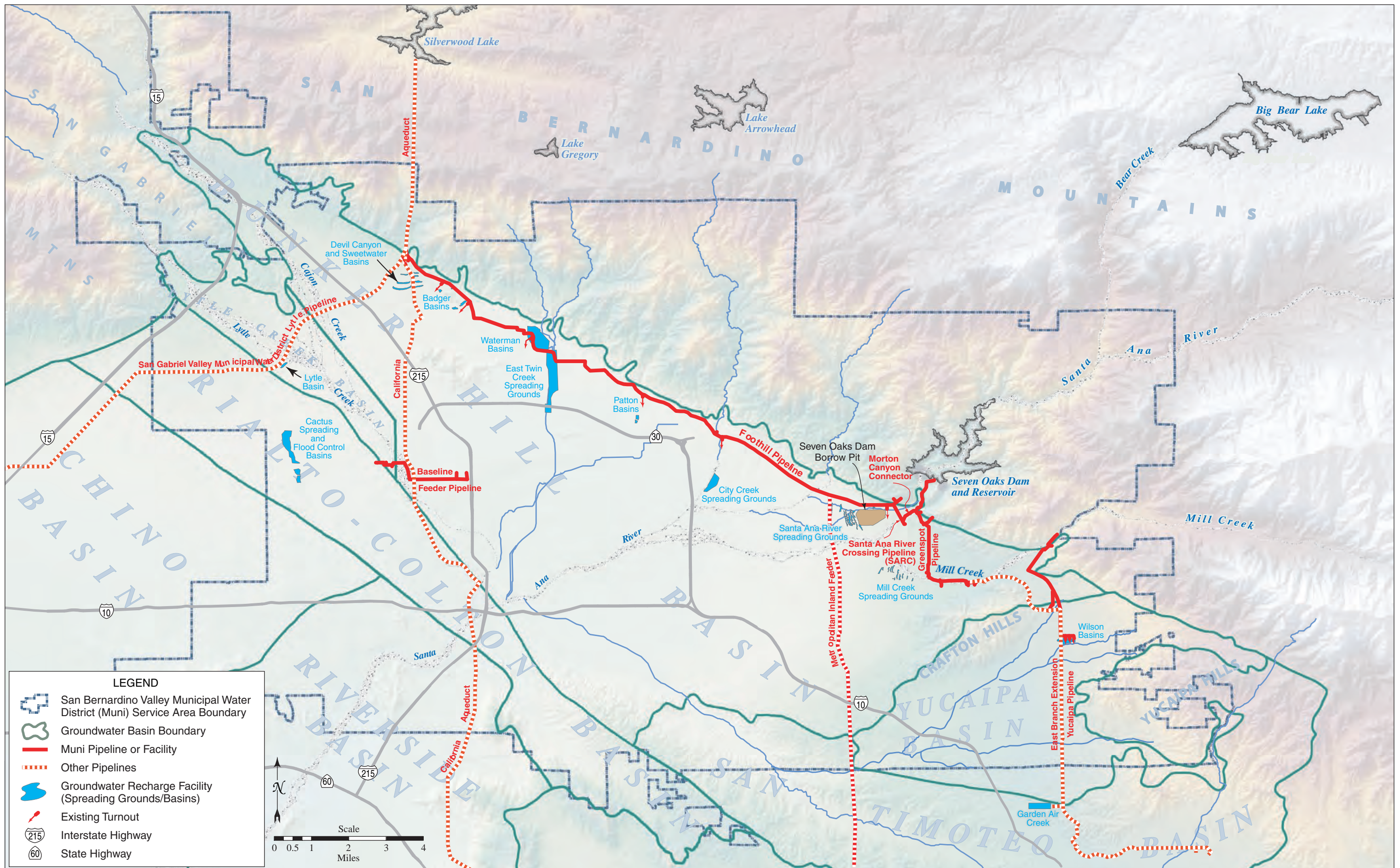
Figure 2-2. Groundwater Recharge Facilities and Underlying Groundwater Basins MUNI/WESTERN EXHIBIT 5-32
