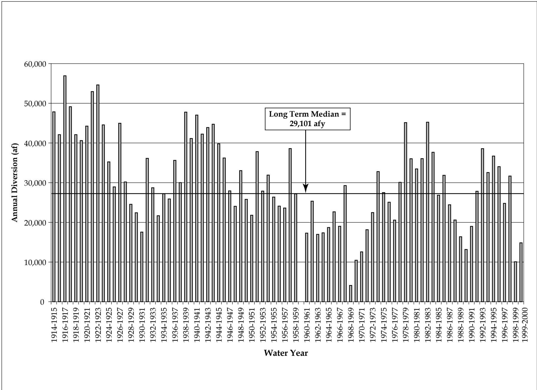
Figure 2.5-1. Southern California Edison Company Canal USGS Gaging Station 11049500, WY 1914-15 through 1999-00
