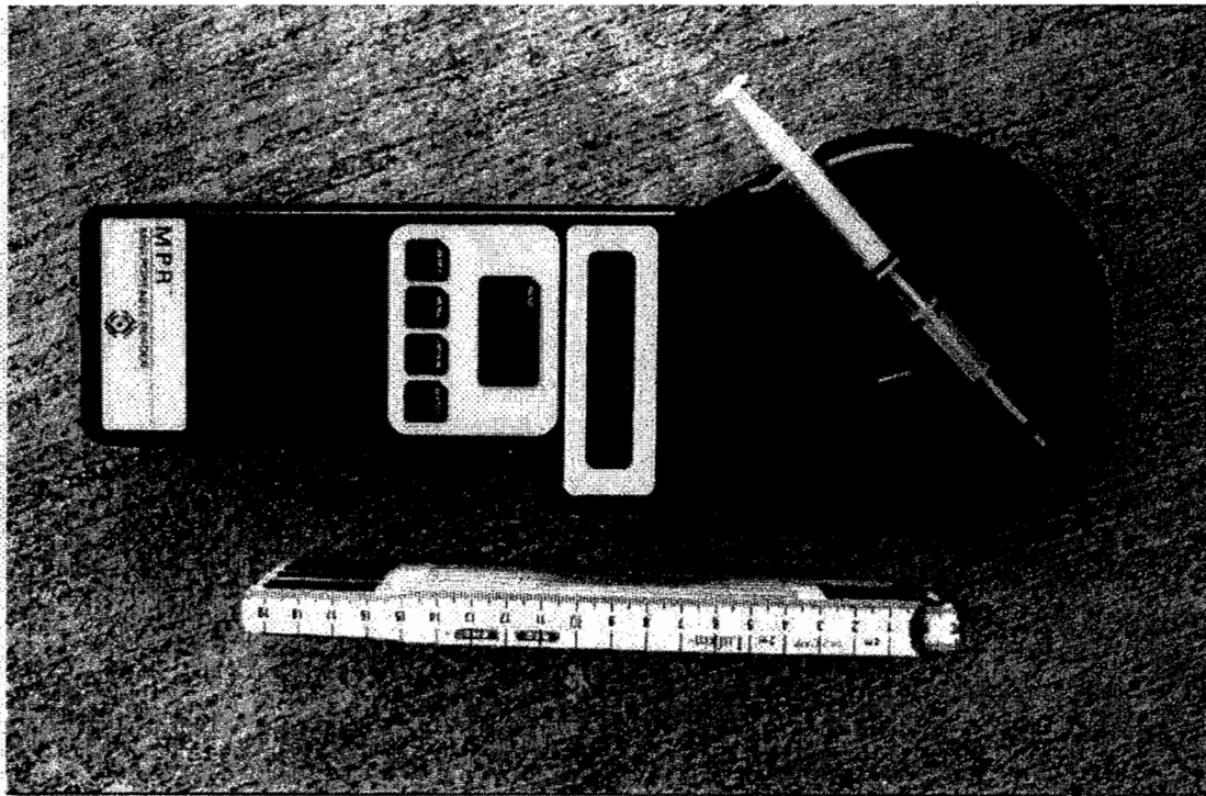
Photo 10. The PIT tagging equipment, including the reader, injector with needle and a PIT tag. A folding meter stick is provided for scale.
