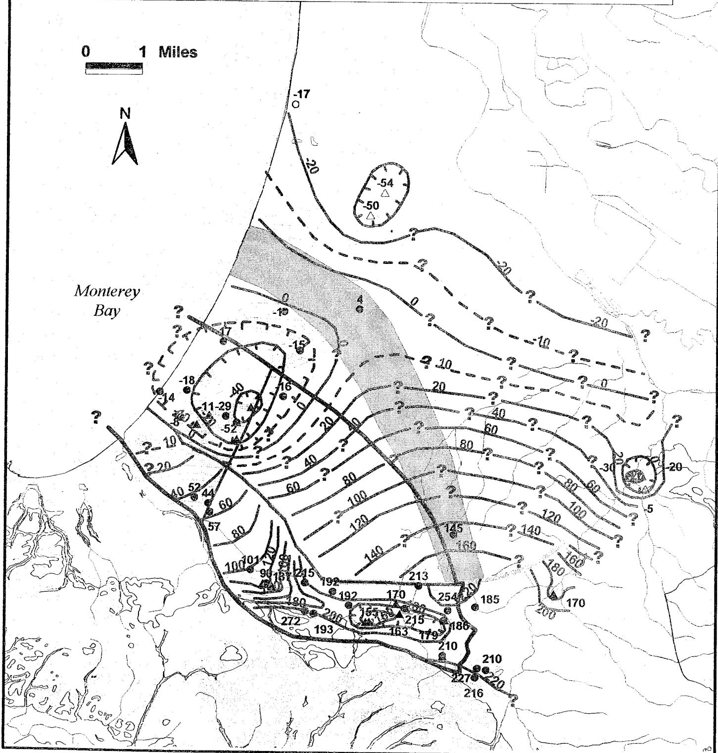
Figure 15. Contours of Groundwater Elevation in the Santa Margarita/Deep Aquifers, Fall 2002
