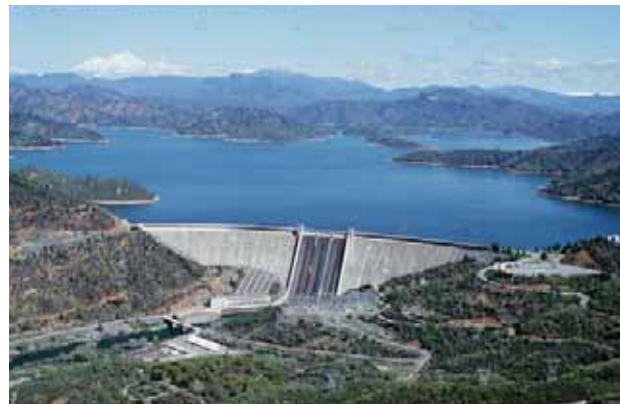
The 4.5 million acre-foot Shasta Reservoir on the Sacramento River near Redding is part of the federal Central Valley Project. Releases from this reservoir play a major role in controlling water quality in the Delta. Raising Shasta Dam and increasing storage in the reservoir are part of the CALFED Surface Storage Program.
