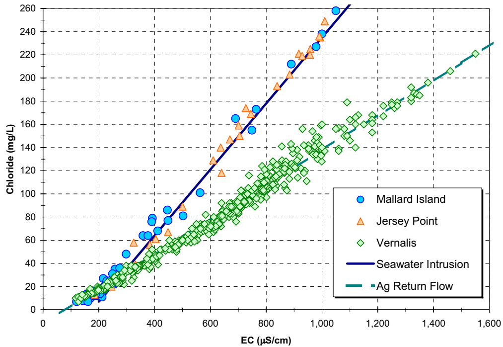
Figure 2C-9 Relationship between Chloride Concentration and Electrical Conductivity
