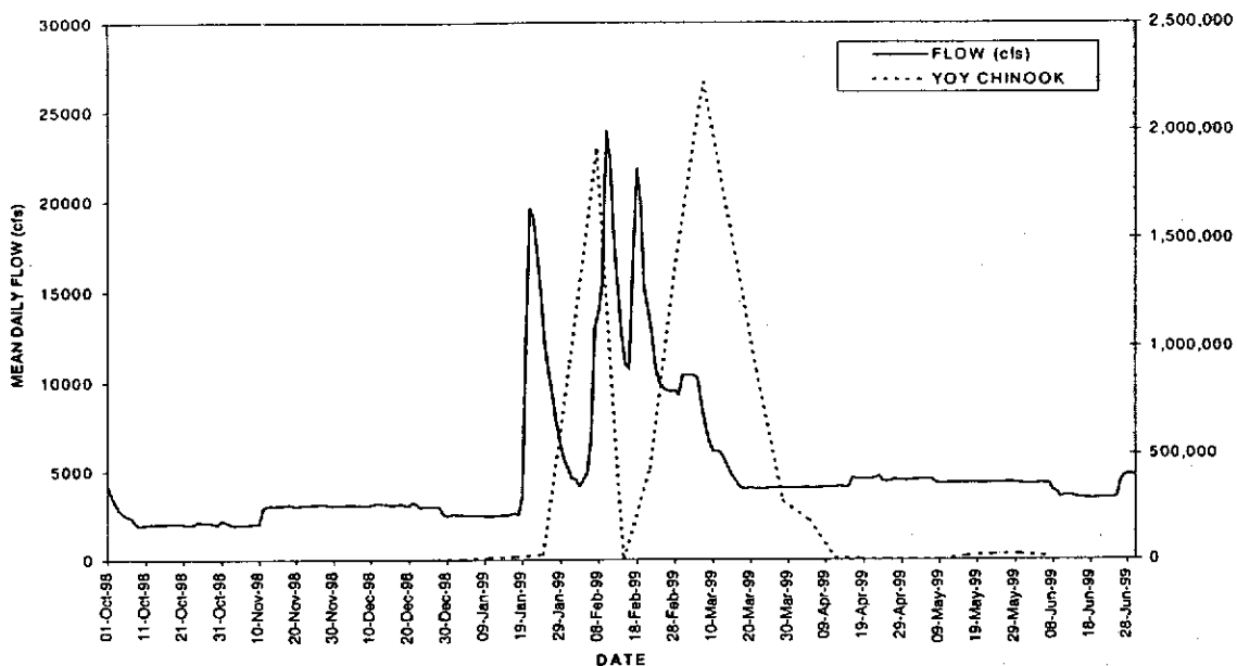
FIGURE B-2. Mean Daily Flow (cfs) at Fair Oaks, October 1998 Through June 1999 and Estimated Abundance of YOY Chinook Salmon Emigrating Weekly from the Lower American River During 1999.
