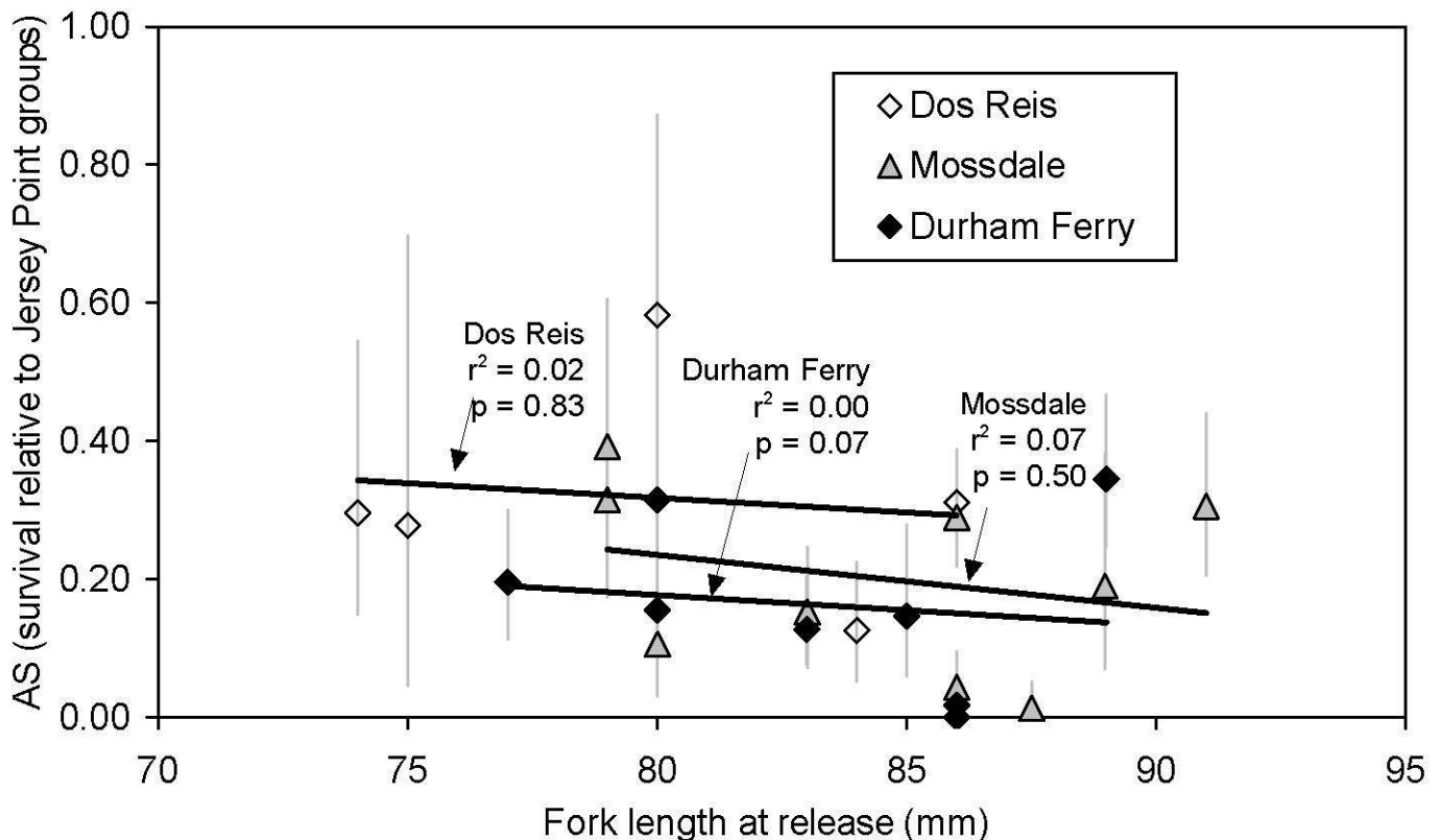
Figure 2. Survival vs size at release and Vernalis flow, for releases near the head of Old River from 1996 through 2003. Survivals are “AS” estimates, relative to recoveries from Jersey Point groups (SJRG 2004). Estimates were made by fitting inverse-Gaussian models to daily trawl effort and tag recovery data by maximum likelihood. The vertical lines are 95% confidence intervals using parametric bootstrap simulation: the BCa method was used for SI, and the percentile method for AS (Efron and Tibshirani 1993).
