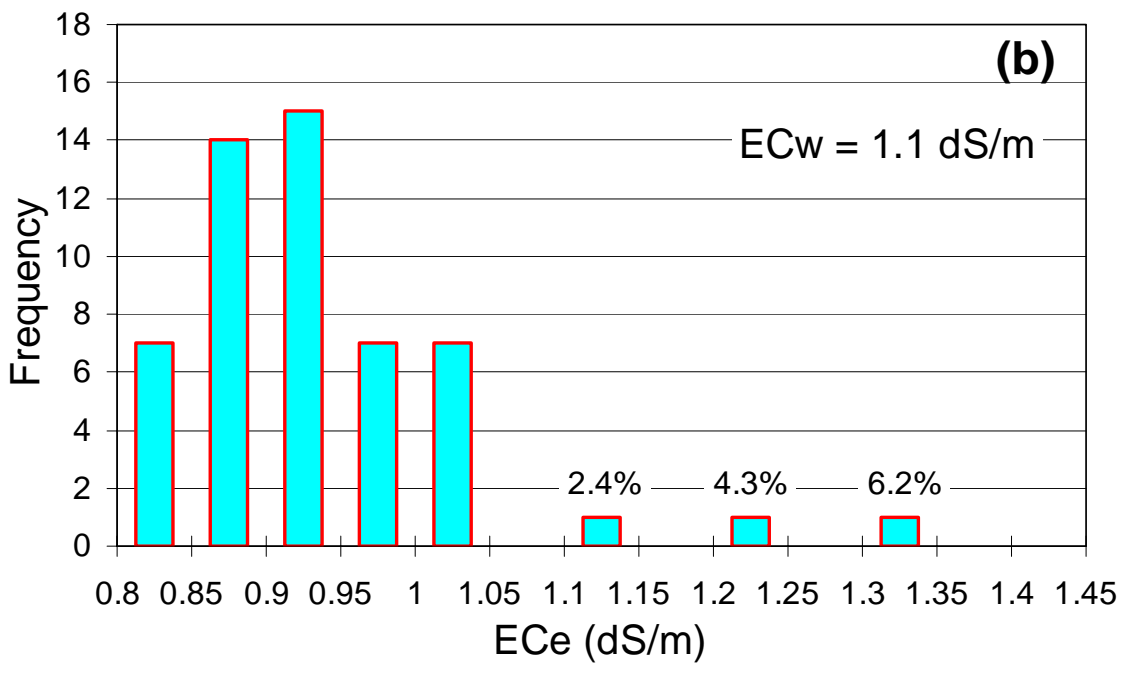
Figure 3.3. Frequency distribution of the seasonal mean ECe obtained by the simulation of the 53 year series assuming the ECw is 1.2 dS/m (a) and ECw is 1.1 dS/m (b). The numbers on top of the bars indicate the predicted yield reduction for that ECe, for yield reductions higher than 2%.
