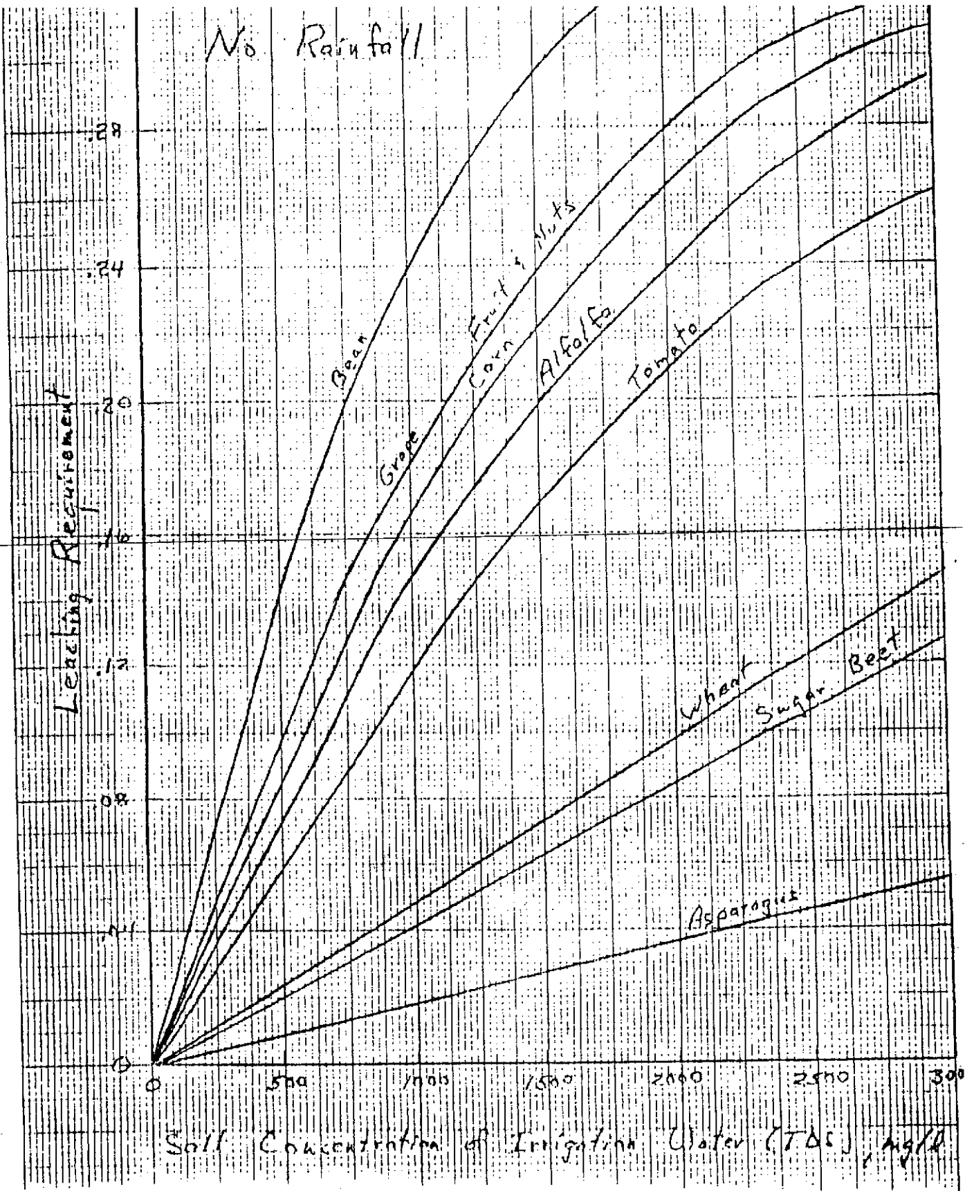
Fig. 1. Leaching requirement of the prominent crops in the South Delta as a function of the salinity of the irrigation water without rainfall.
