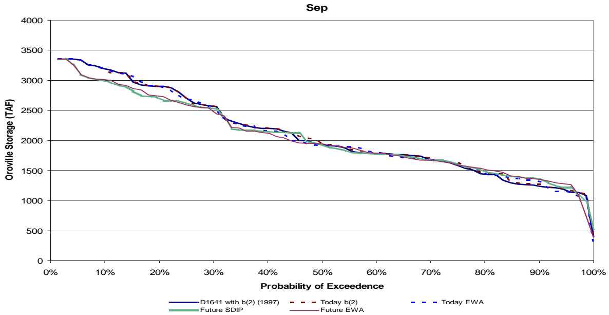
Figure 11-12 Oroville Reservoir End of September Exceedance
