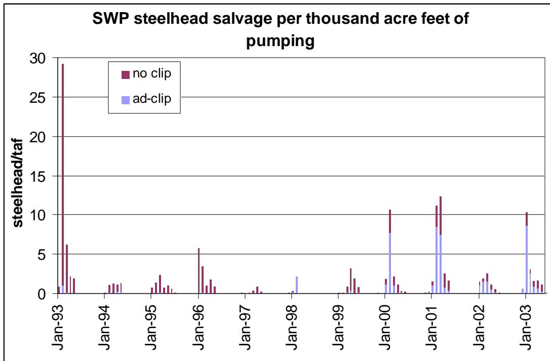
Figure 10–2 SWP steelhead salvage density, 1993-2003.
