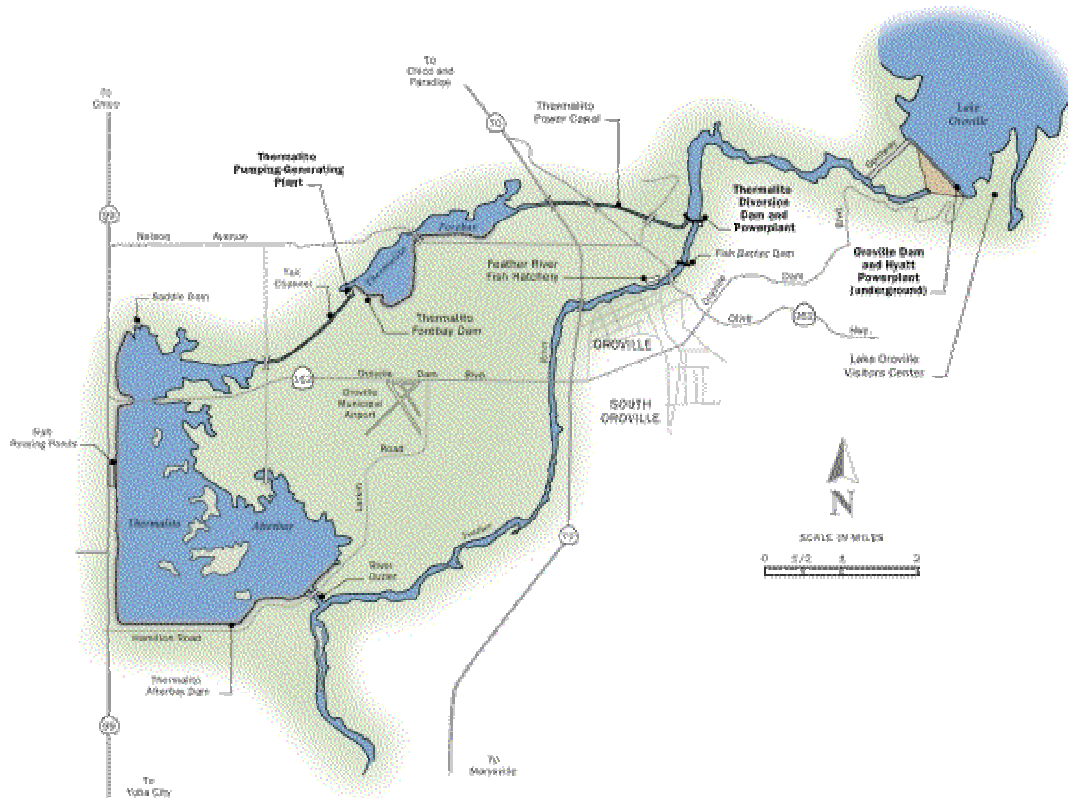
Figure 2-7 Oroville Facilities on the Feather River
