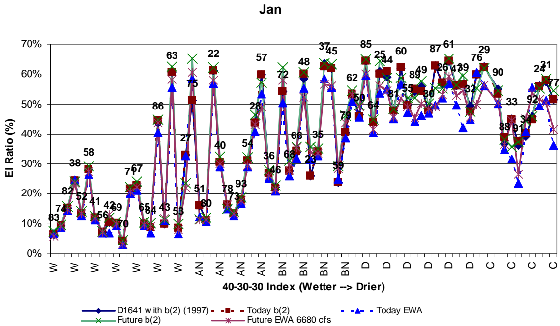
Figure 10–36 January export-to-inflow ratio sorted by 40-30-30 Index
