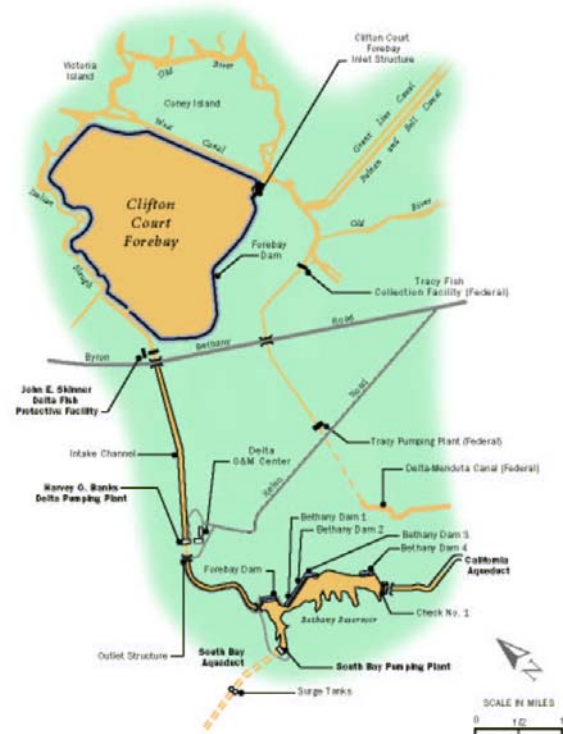
CLIFTON COURT FOREBAY AND FOREBAY GENERAL PLAN
