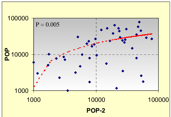
Figure 52. Log of salmon escapement versus log of escapement two years earlier.
