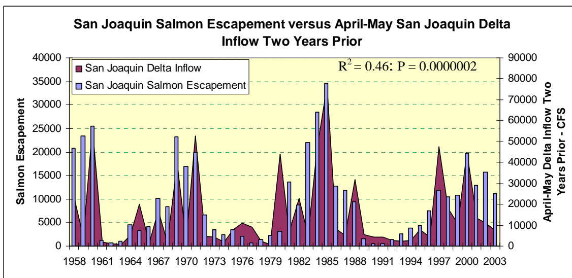
Figure 50. San Joaquin tributary spawner escapement from 1958-2003 and April-May Delta inflow two-years prior (the flow when three year old salmon would have been migrating a young through the Delta to the ocean).
