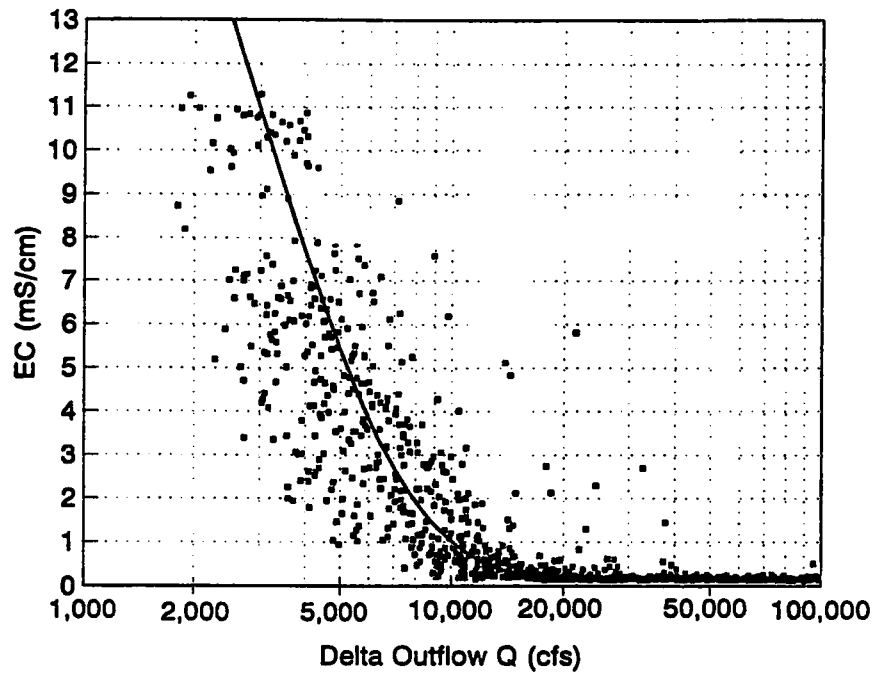
Figure 4.1(a). 14-day average salinity at Collinsville as a function of 14-day average net Delta outflow (Q). The data shown are for water years 1968 through 1986.
