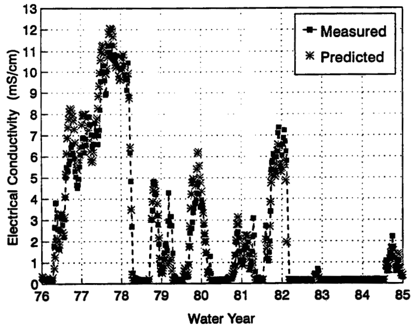
Figure 4.4. Measured and predicted 14-day average salinity at Collinsville for the period, 1976-1985. The stars represent predictions using Denton's antecedent flow model. The squares joined by dashed lines represent field-measured salinities.
