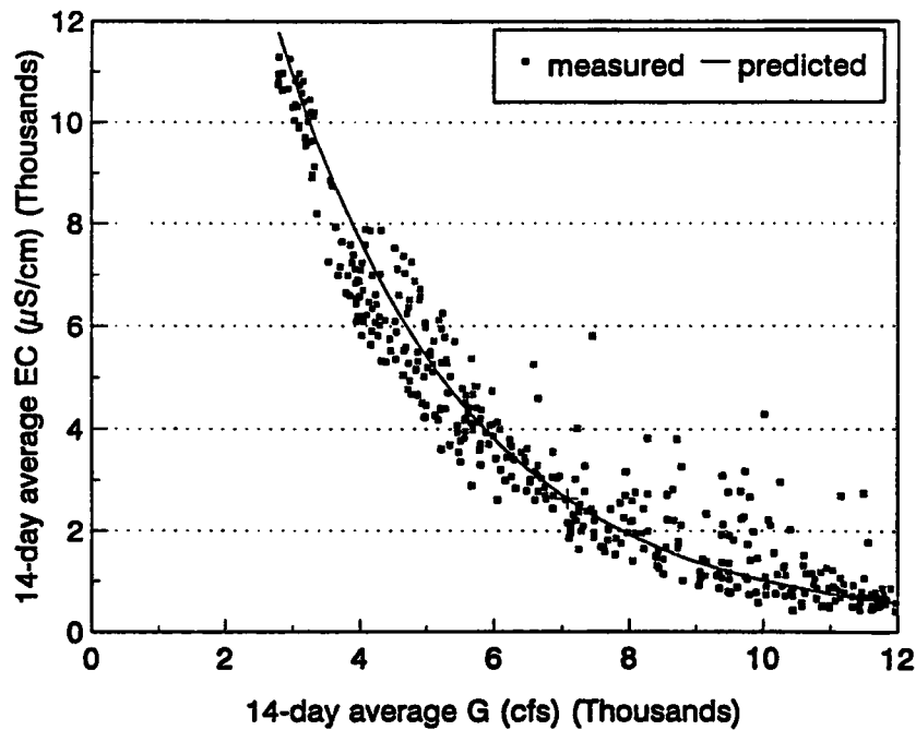
Figure 4.1(b). Predicted and measured 14-day average salinity at Collinsville. The solid line is the salinity predicted using Denton's antecedent flow relations and overall "best-fit" parameters from table 4.1 (below). The cross indicates the model prediction at EC=2640 μS/cm using locally "best-fit" parameters in the vicinity of EC=2640 μS/cm.
