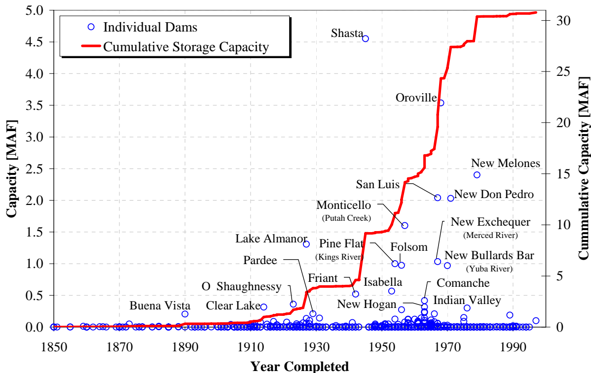
Figure A-6 – Surface Reservoir Capacity
