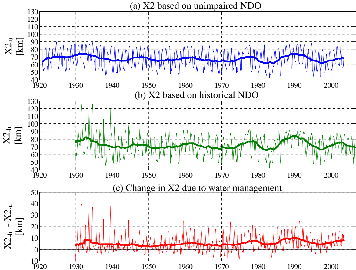
Figure 3-11 – Location of X2 under unimpaired and historical conditions
