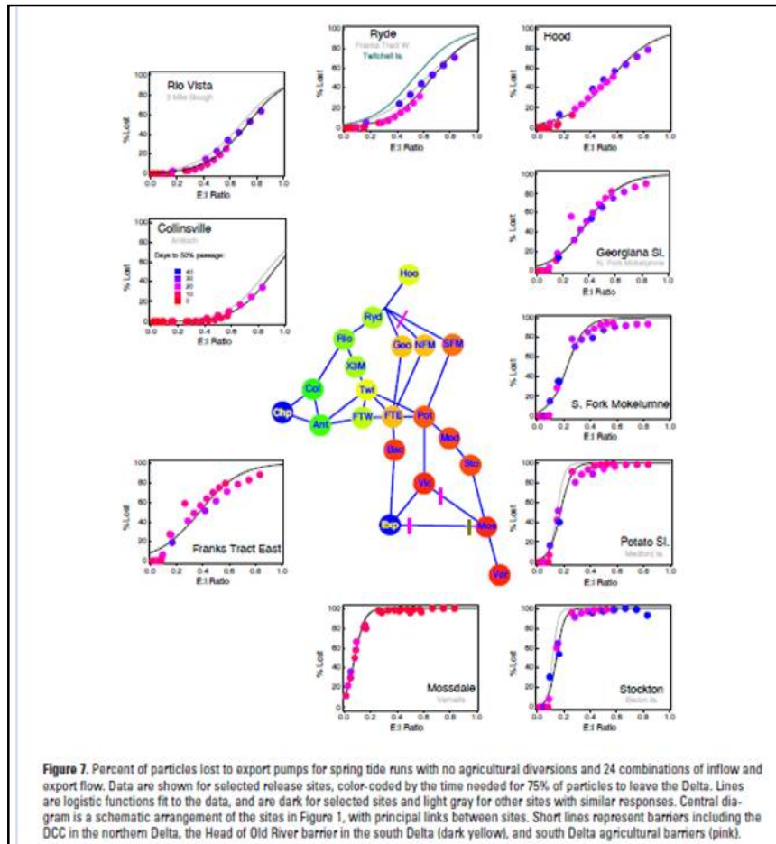
Figure 16 Results of particle tracking model simulations showing the percentage of particle released at different locations within the Delta entrained into the CVP or SWP export facilities at different E:I ratio conditions. For particles released in the southern Delta, most or all of the particles were entrained by the CVP or SWP pumps within a few weeks at E:I ratio >0.2. From: Nobriga and Kimmerer 2008.
