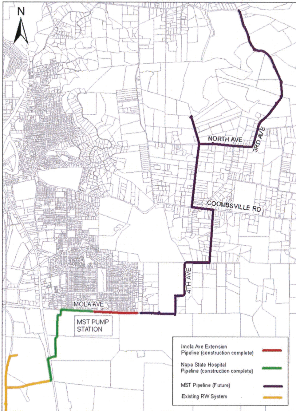
Figure 1: Pump Station Location and Pipeline Alignment
