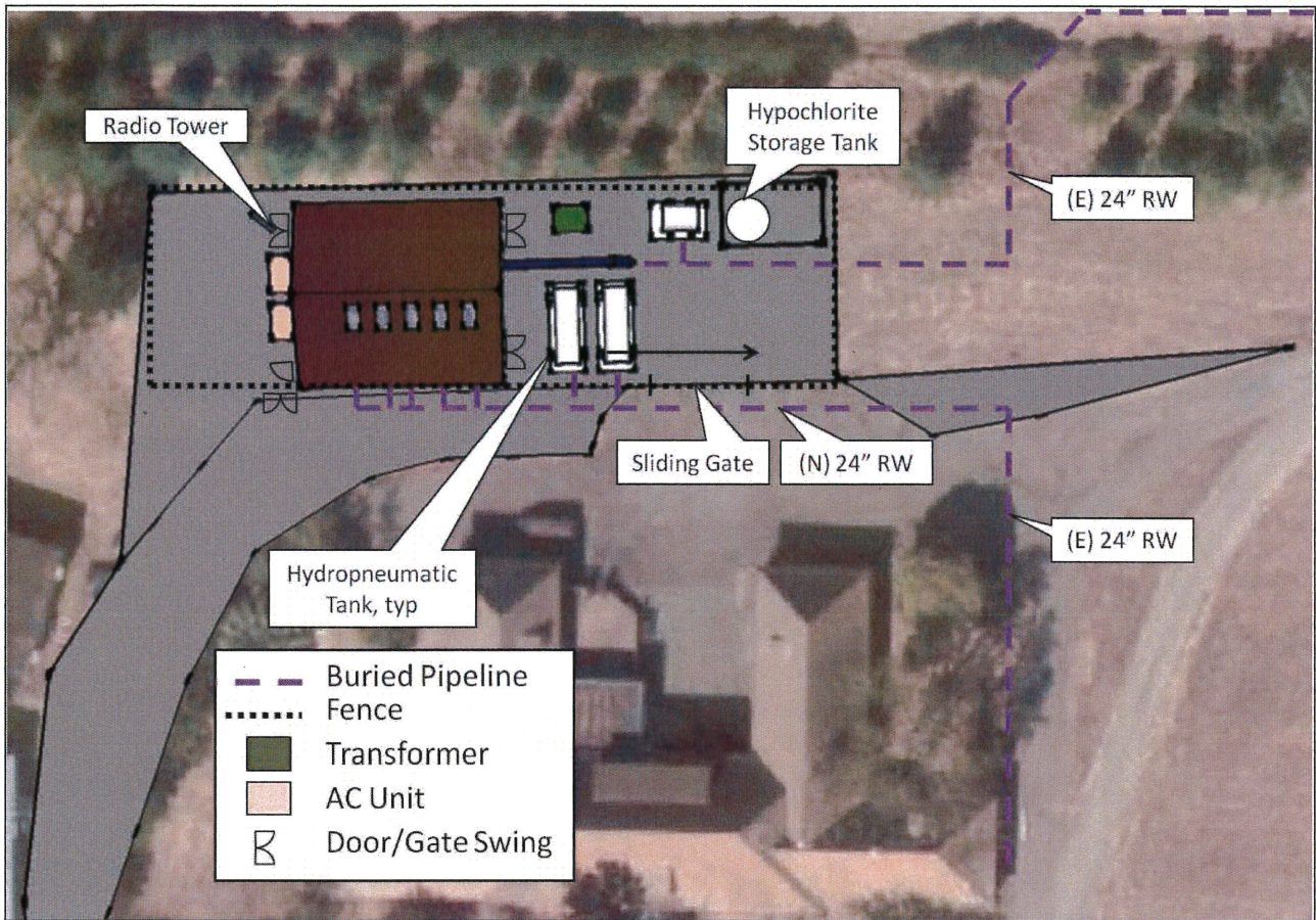
Figure 2: Pump Station Conceptual Site Plan
