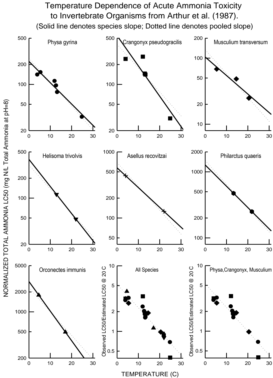
Figure M.6. Temperature Dependence of Acute Ammonia Toxicity to Invertebrate Organisms from Arthur et al. (1987).
