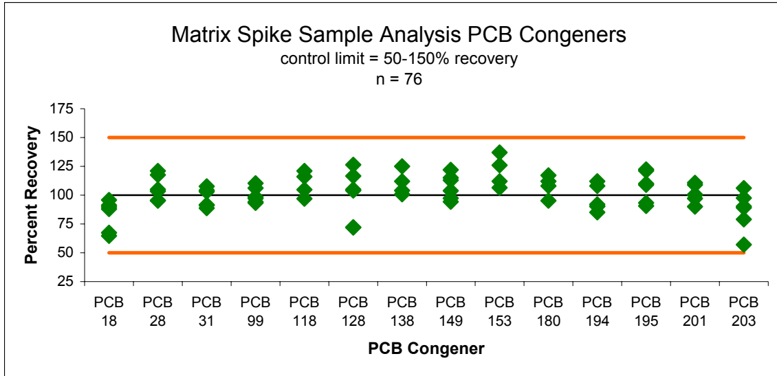
Figure A1-4. Control chart for MS/MSD sample analysis for PCB.
