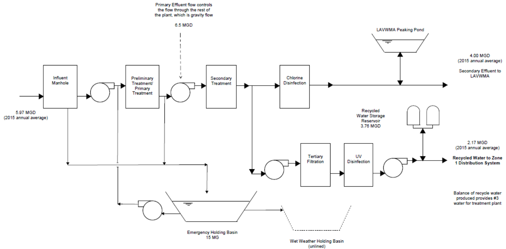
Livermore Water Reclamation Plant Wastewater and Recycled Water Treatment Facilities
