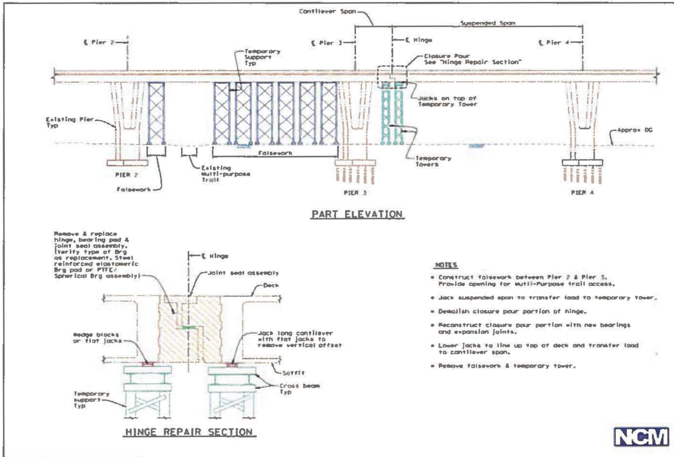
Figure 5 Temporary Falsework and Support Structures
