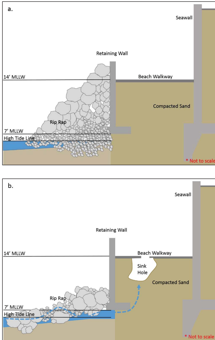
Figure 1. Cross sections of the originally designed riprap ( panel a. ) and the existing conditions ( panel b. ), in which the riprap has subsided, allowing intrusion of seawater during high tide wave and/or large swell events. Seawater has eroded through the engineered compacted sand, causing sink holes beneath the walkway.
