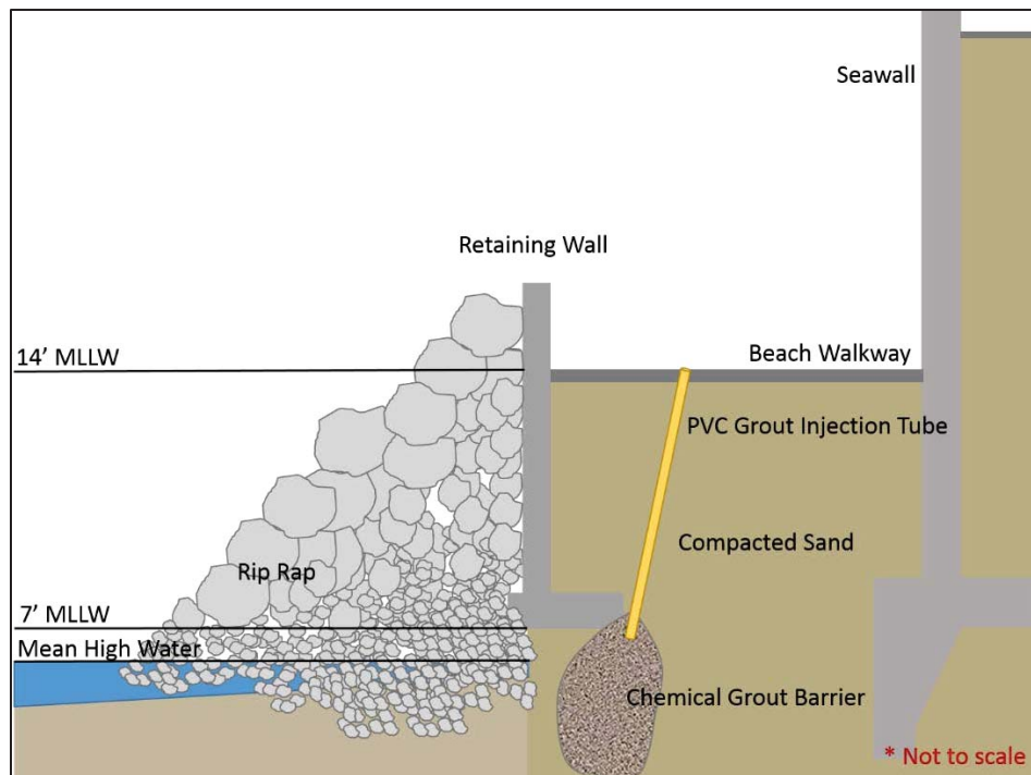
Figure 4. Grout injection process. Preset polyvinyl chloride (PVC) pipes in the beach walkway will be injected with a site-specific formula of chemical grout, commonly used in shoreline applications. The chemical grout barrier will provide a barrier from future erosion and seawater intrusion that would otherwise compromise the compacted sand beneath the walkway.
