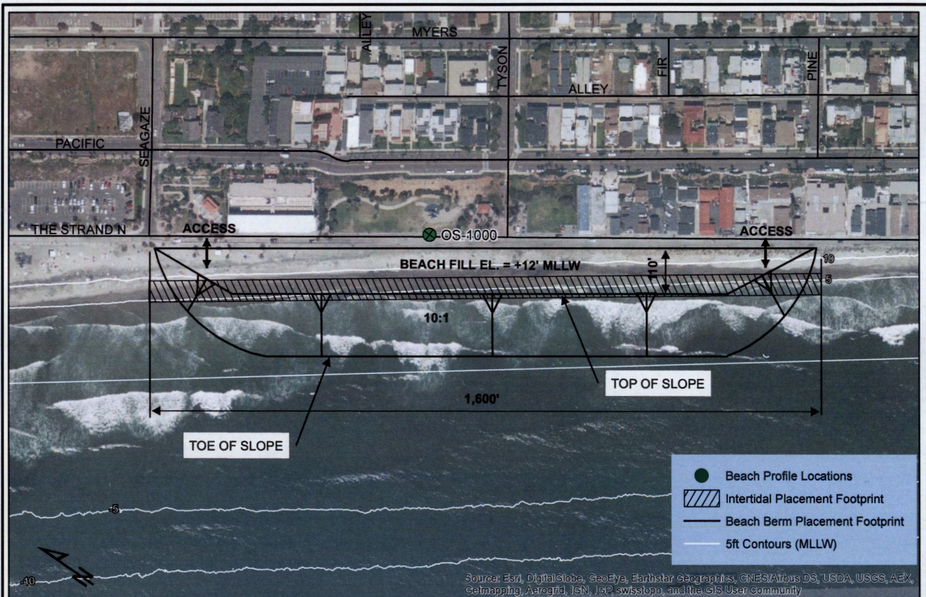
Northern Placement Site - Plan View
