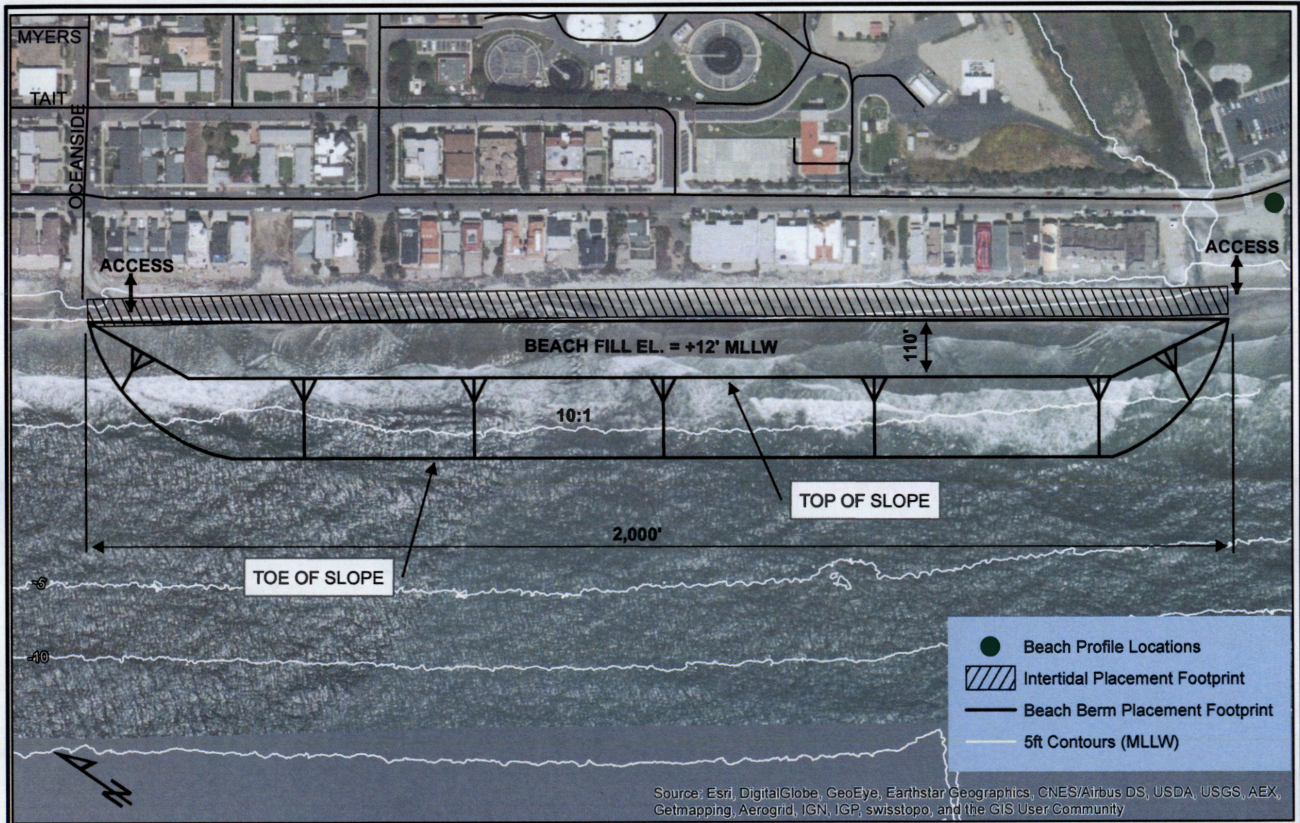
Southern Placement Site - Plan View
