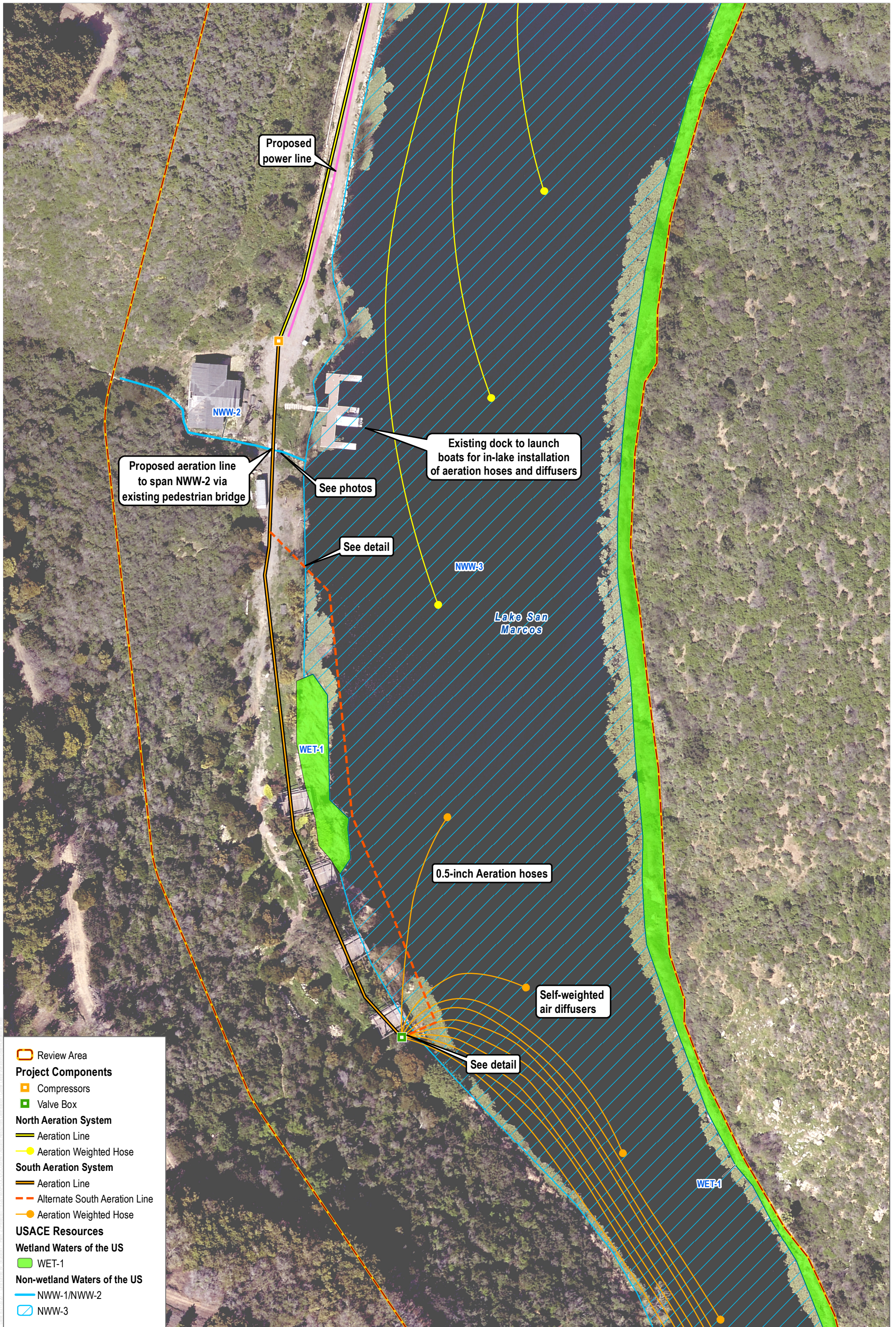
Figure 3: Lake aeration system project overview and detailed maps
