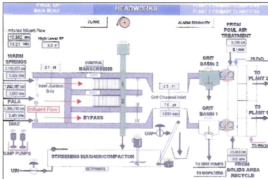
Figure 4. SCADA Graphical Interface
