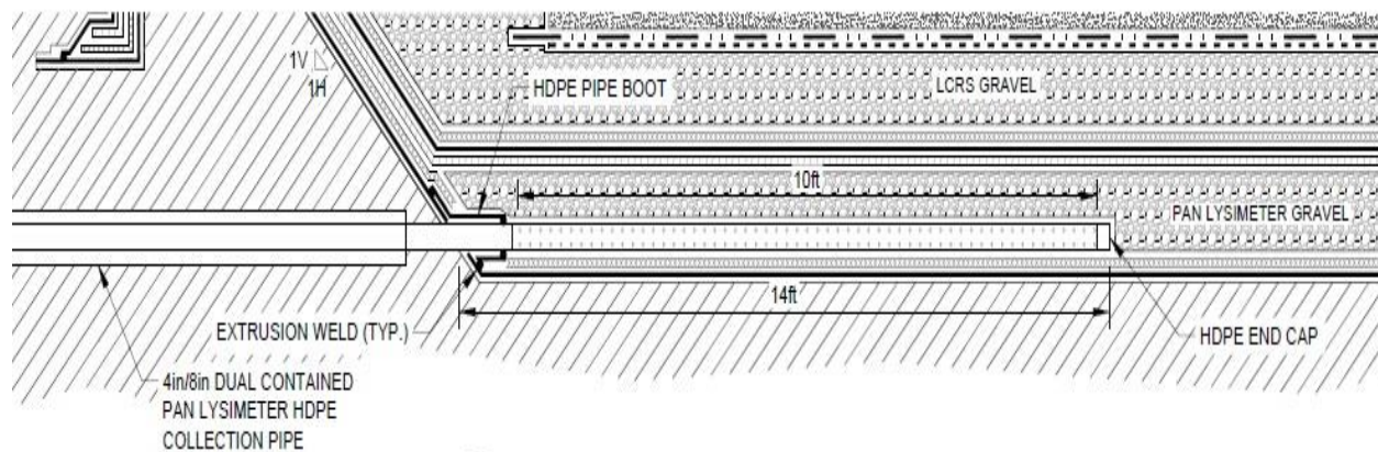
SCALE N.T.S. 2 PAN LYSIMETER DRAINAGE PIPE TYPICAL SECTION 3
