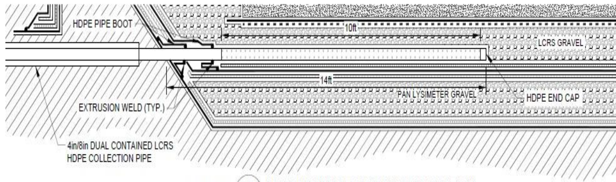
SCALE N.T.S. 1 LCRS DRAINAGE PIPE TYPICAL SECTION 3
