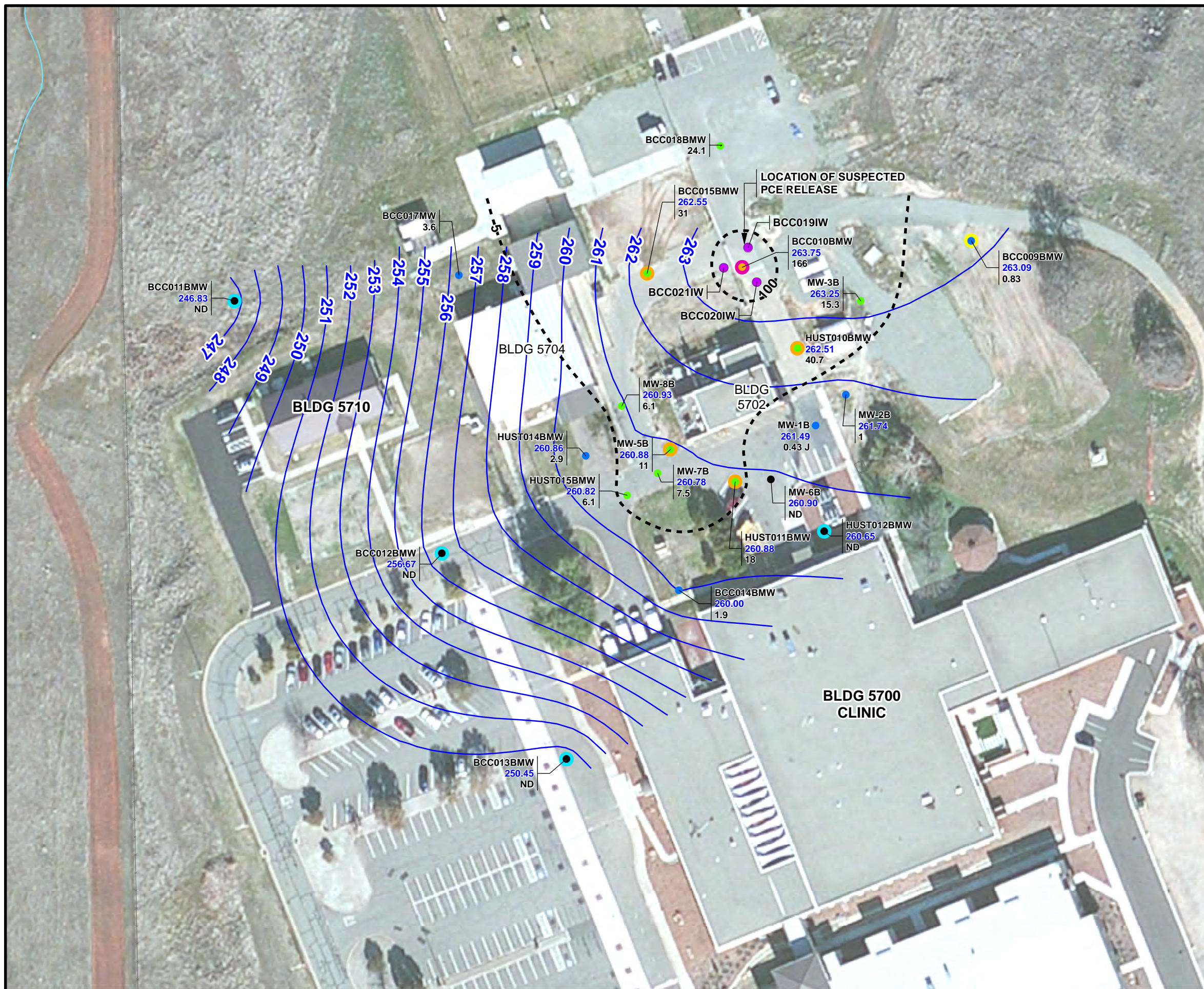
FIGURE 4-1 CG041-517 PCE CONCENTRATIONS IN GROUNDWATER AND PROPOSED INJECTION WELL LOCATIONS SITE CG517 AND CG041-517 STATEMENT OF BASIS/ CORRECTIVE MEASURES IMPLEMENTATION WORK PLAN BEALE AIR FORCE BASE, CALIFORNIA
