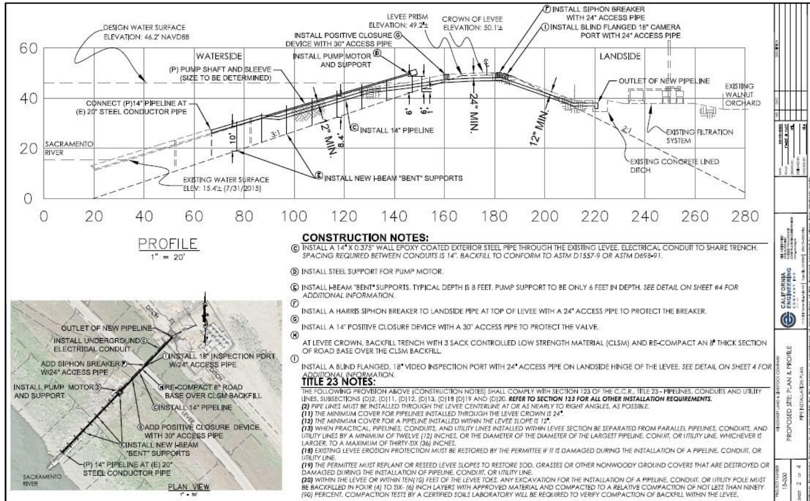
Figure 2: Project Site Plan and Profile
