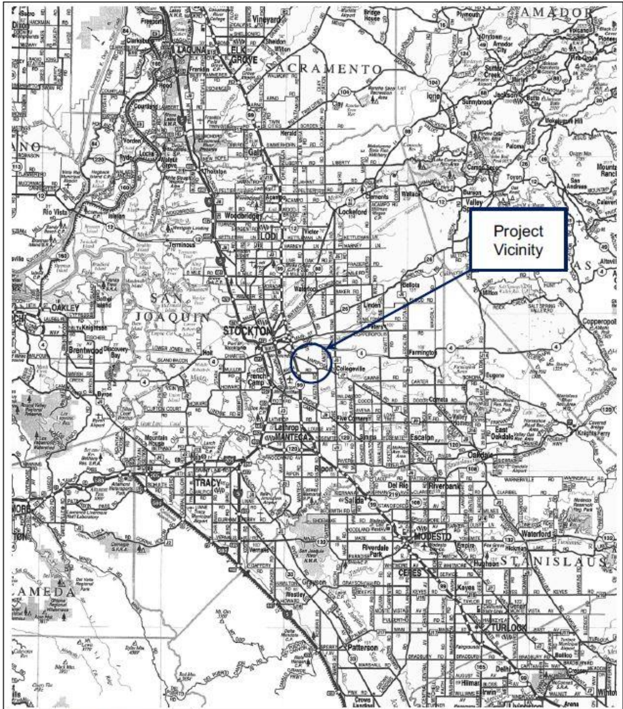
FIGURE 1 PROJECT VICINITY
