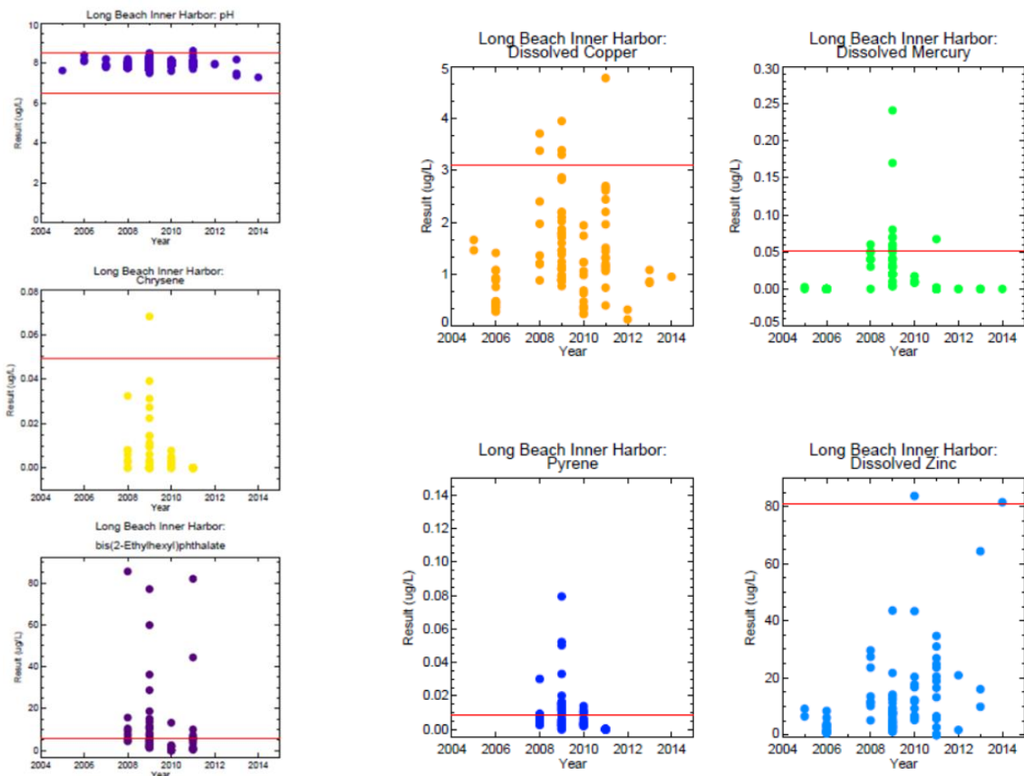
Figure 2-1: Pollutants in water exceeding water quality assessment thresholds
