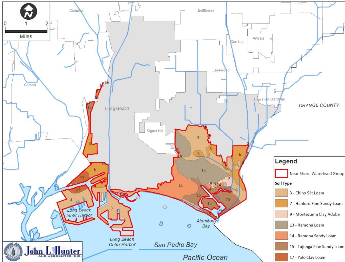
Figure 1-6: Soil Types 17
