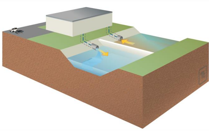
Figure 3-15: Low flow diversion schematic
