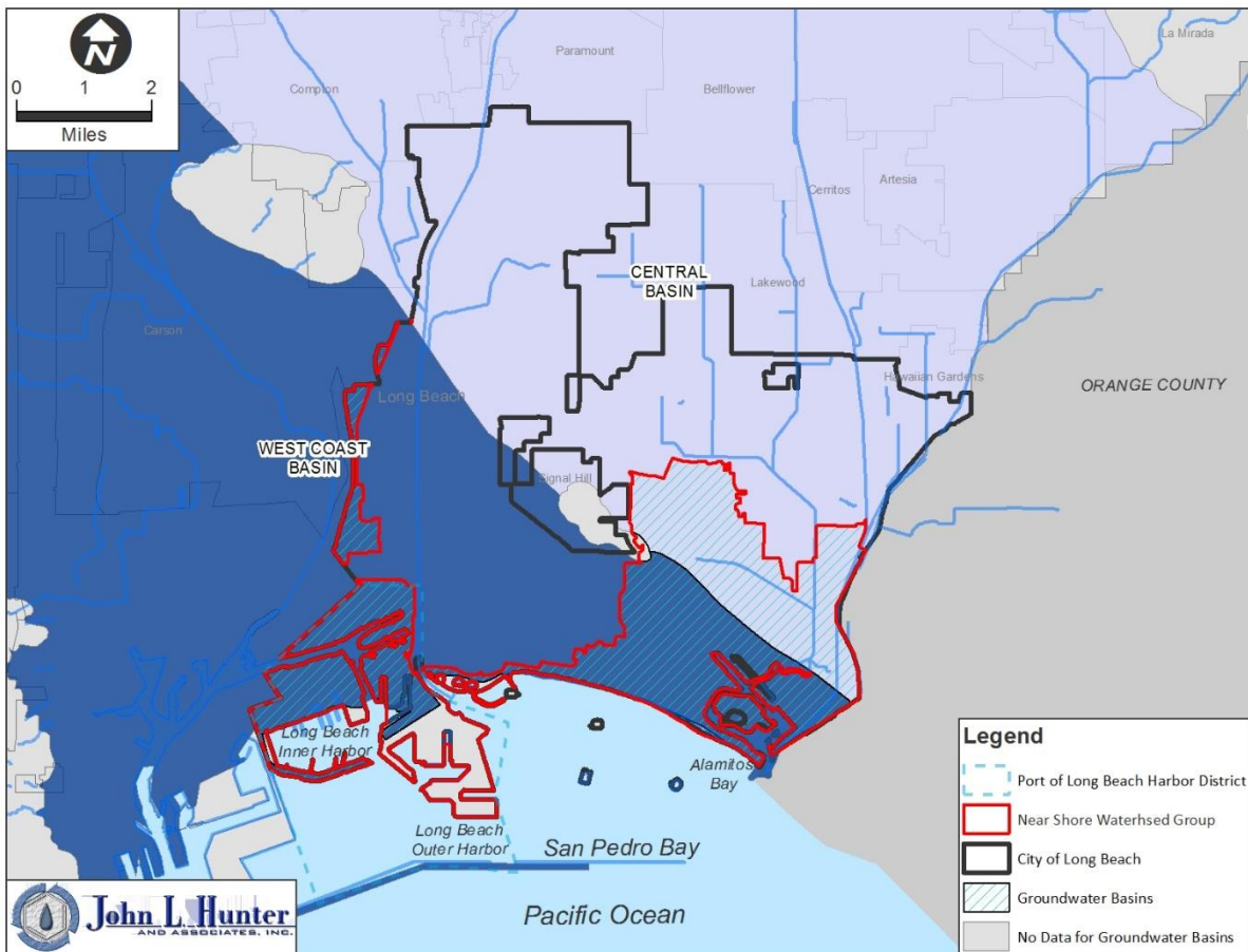
Figure 1-7: Groundwater Basins
