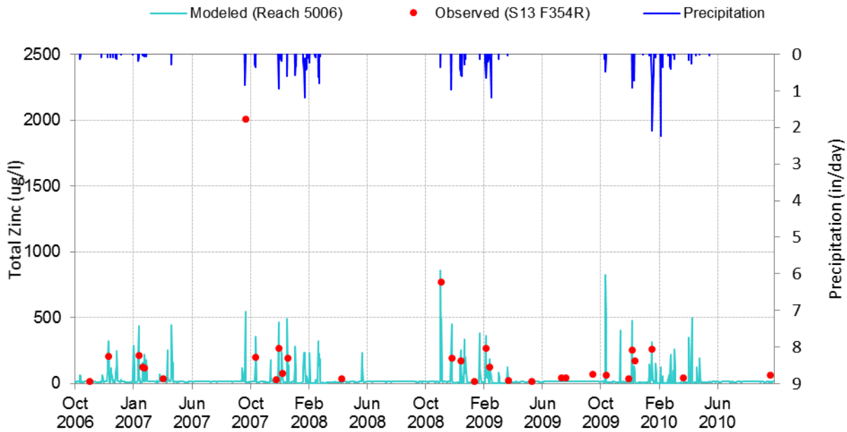
Figure E-13. Simulated vs. observed timeseries plots for Total Zinc (10/1/2006 through 9/30/2010) at Coyote Creek below Spring Street (S13).
