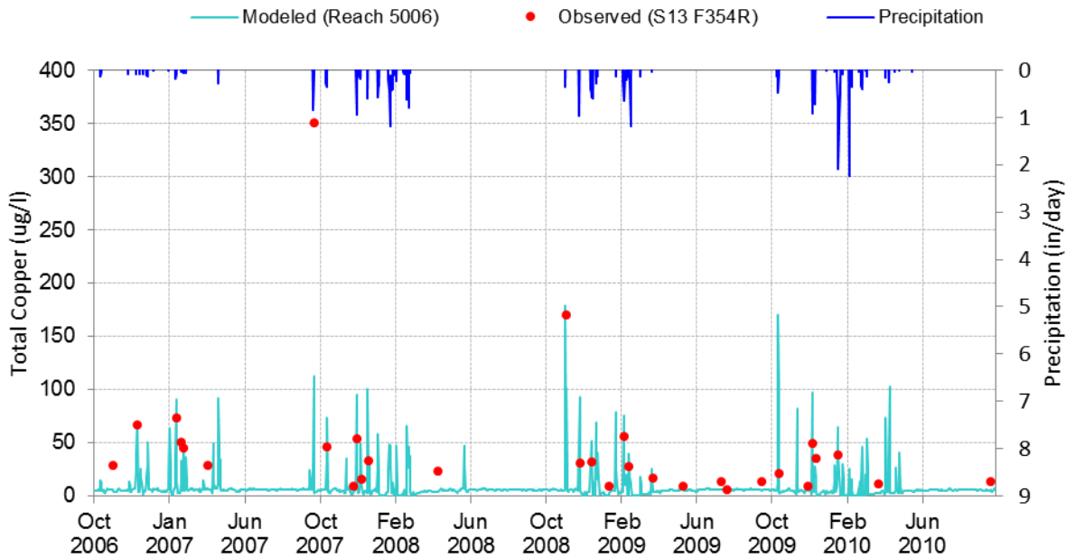
Figure E-15. Simulated vs. observed timeseries plots for Total Copper (10/1/2006 through 9/30/2010) at Coyote Creek below Spring Street (S13).
