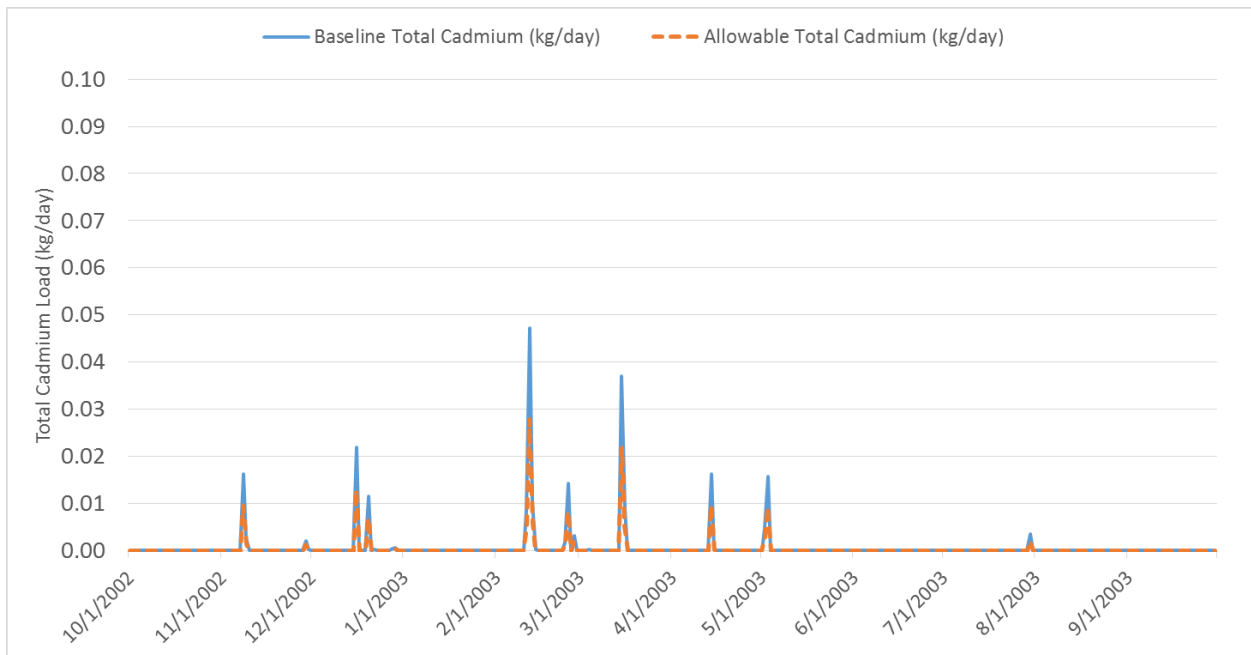
Figure 4. Baseline (WY 2003) and allowable total cadmium load for Dominguez Toxics assessment zone.
