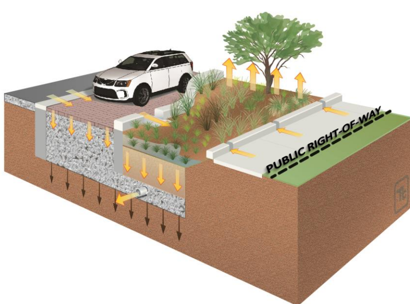
Figure 1. Conceptual schematic of ROW BMPs with an underdrain (arrows indicate water pathways).
