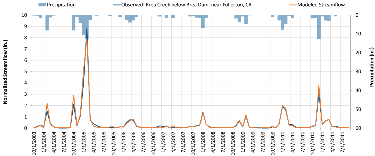
Figure E-2. Monthly flow at Brea Creek below Brea Dam, near Fullerton, CA (Station ID: 11088500).
