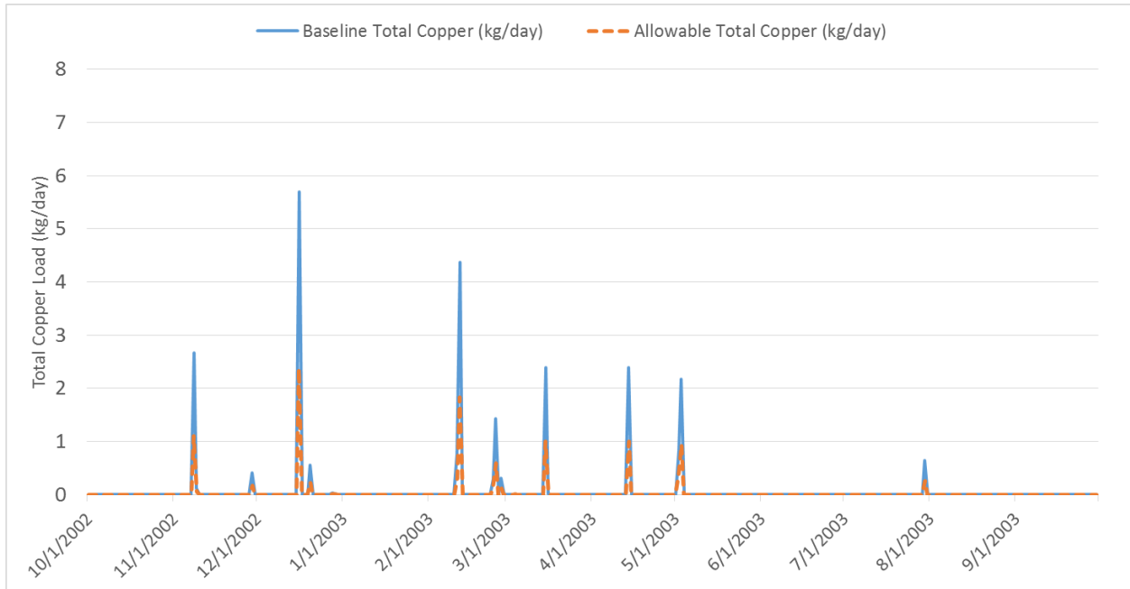
Figure 2. Baseline (WY 2003) and allowable total copper load for Dominguez Toxics assessment zone.
