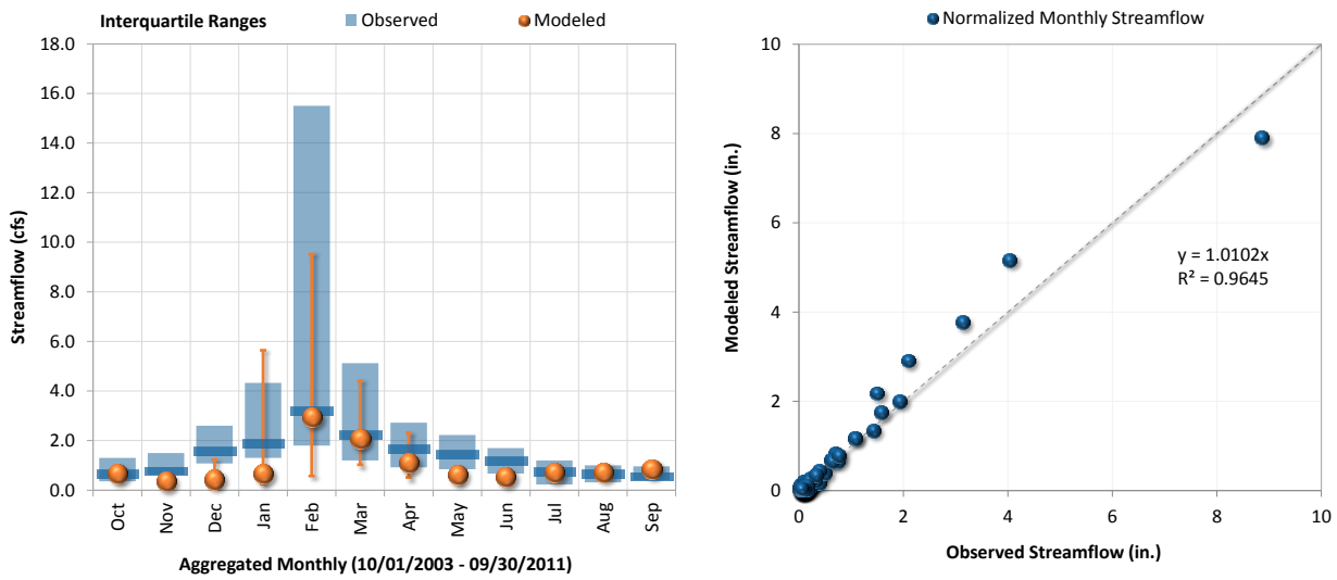
Figure E-4. Monthly flow interquartiles at Brea Creek below Brea Dam, near Fullerton, CA (Station ID: 11088500).
