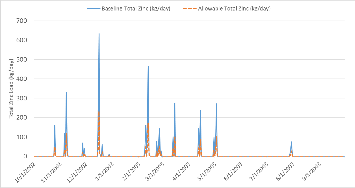
Figure 9. Baseline (WY 2003) and allowable total zinc load for Harbor Toxics assessment zone.
