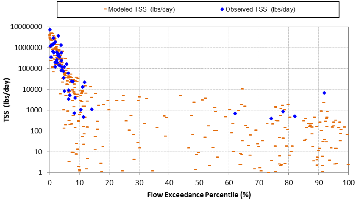
Figure E-10. Simulated vs. observed load duration plots for Total Sediment (10/1/2006 through 9/30/2011) at Coyote Creek below Spring Street (S13).
