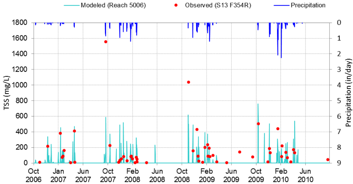
Figure E-11. Simulated vs. observed timeseries plots for Total Sediment (10/1/2006 through 9/30/2010) at Coyote Creek below Spring Street (S13).
