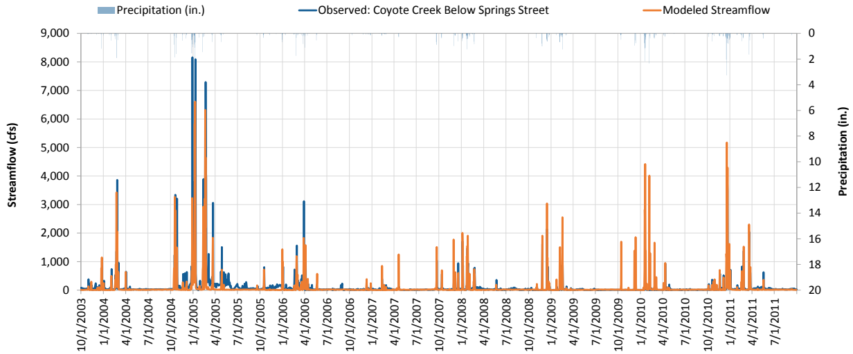
Figure E-5. Daily flow at Coyote Creek Below Springs Street (Station ID: F354).
