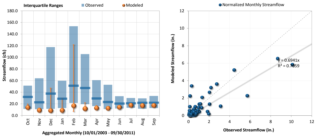
Figure E-8. Monthly flow interquartiles at Coyote Creek Below Springs Street (Station ID: F354).
