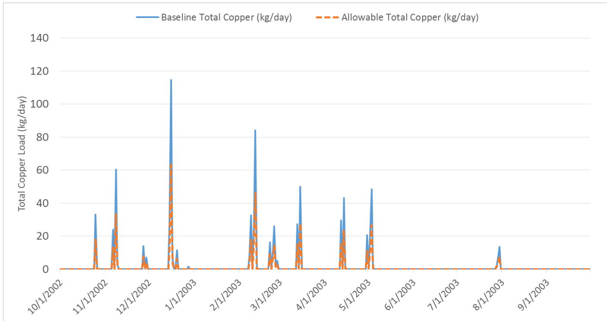
Figure 7. Baseline (WY 2003) and allowable total copper load for Harbor Toxics assessment zone.
