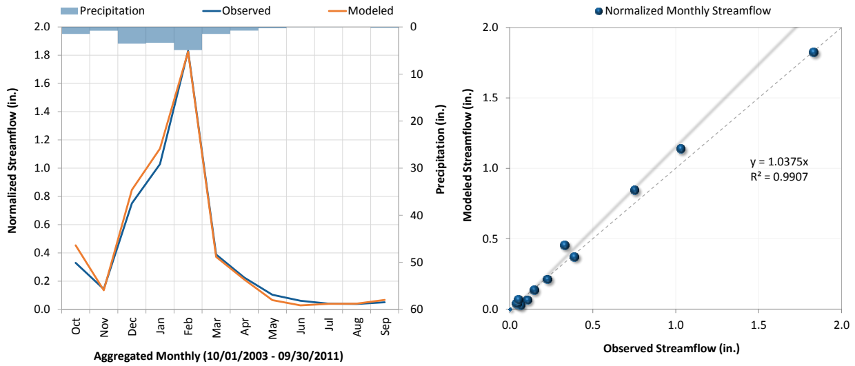
Figure E-3. Average monthly flow at Brea Creek below Brea Dam, near Fullerton, CA (Station ID: 11088500).
