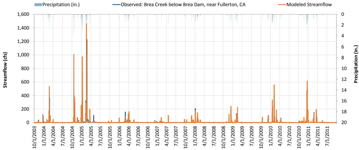
Figure E-1. Daily flow at Brea Creek below Brea Dam, near Fullerton, CA (Station ID: 11088500).
