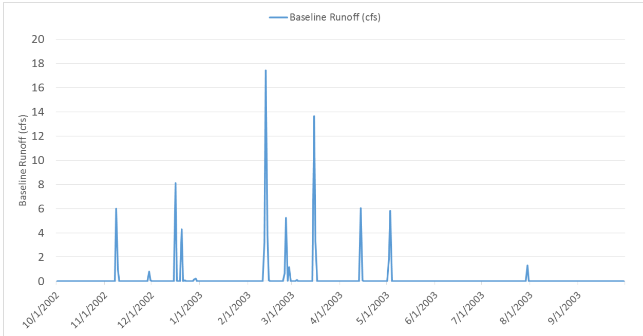
Figure 1. Baseline (WY 2003) runoff for Dominguez Toxics assessment zone.
