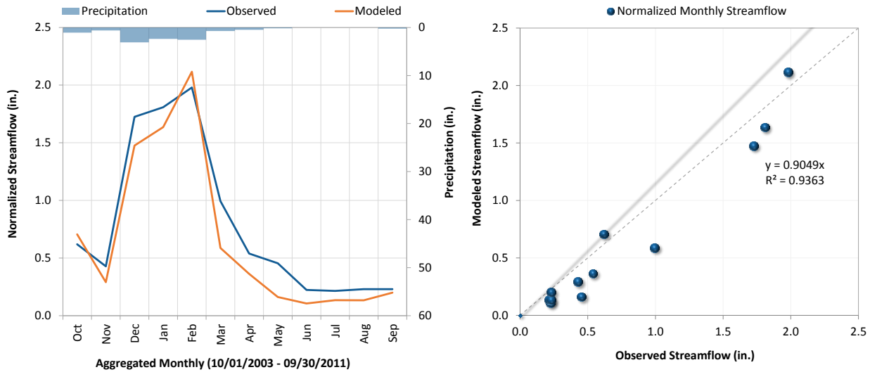
Figure E-7. Average monthly flow at Coyote Creek Below Springs Street (Station ID: F354).
