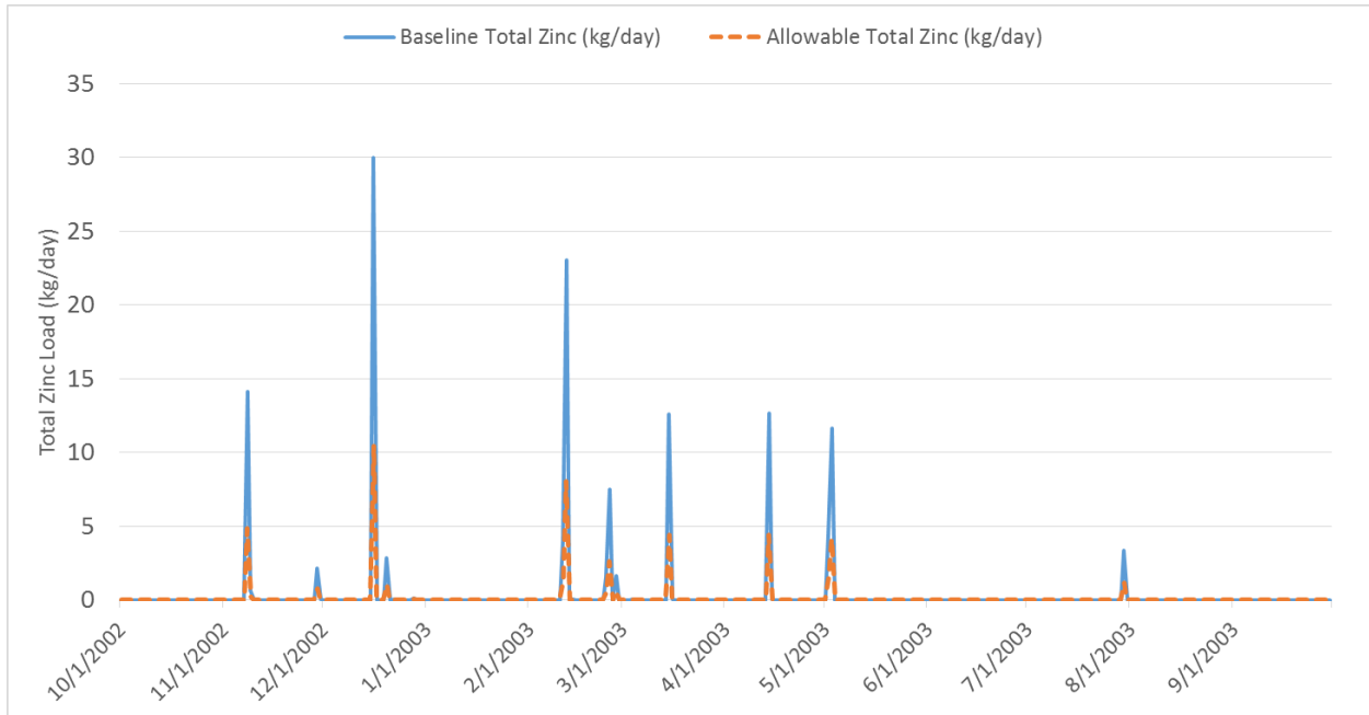
Figure 3. Baseline (WY 2003) and allowable total zinc load for Dominguez Toxics assessment zone.
