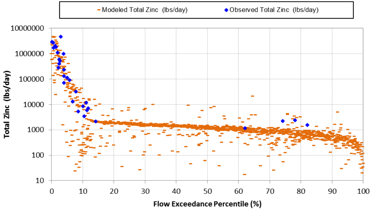
Figure E-12. Simulated vs. observed load duration plots for Total Zinc (10/1/2006 through 9/30/2010) at Coyote Creek below Spring Street (S13).
