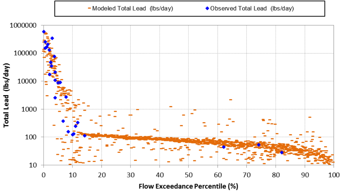
Figure E-16 Simulated vs. observed load duration plots for Total Lead (10/1/2006 through 9/30/2010) at Coyote Creek below Spring Street (S13).
