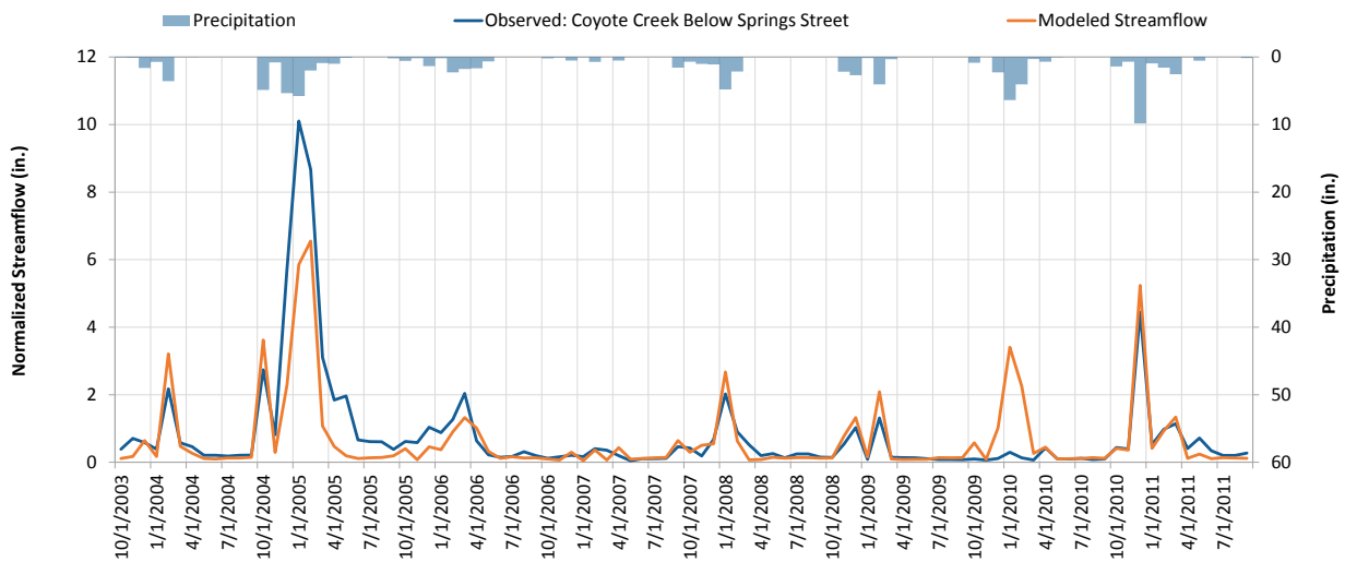
Figure E-6. Monthly flow at Coyote Creek Below Springs Street (Station ID: F354).
