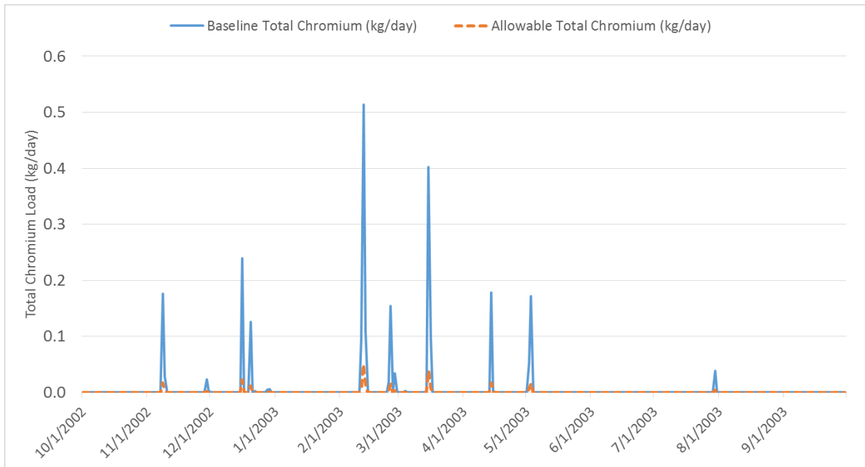
Figure 5. Baseline (WY 2003) and allowable total chromium load for Dominguez Toxics assessment zone.
