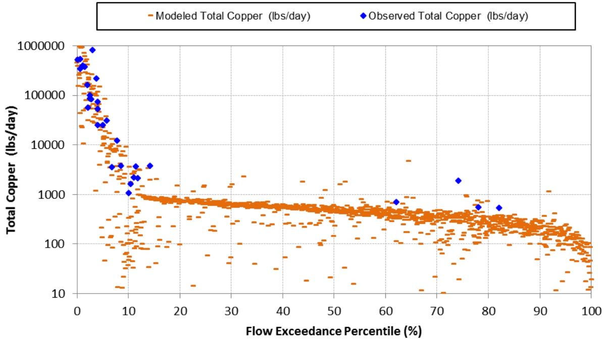
Figure E-14. Simulated vs. observed load duration plots for Total Copper (10/1/2006 through 9/30/2010) at Coyote Creek below Spring Street (S13).
