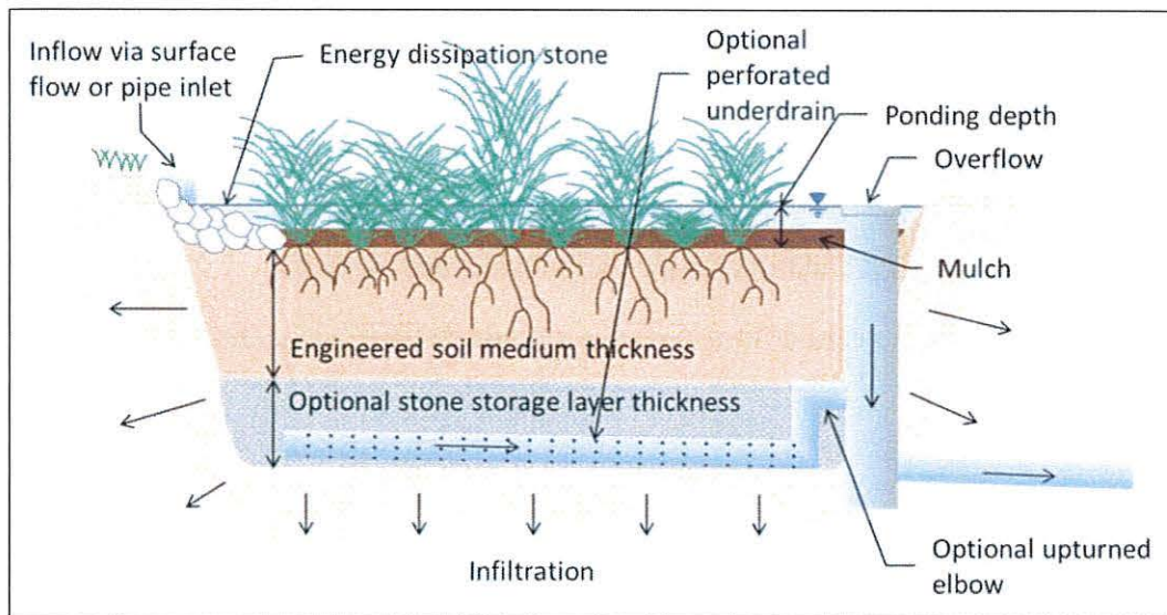
Figure 1. Cross sections of typical biofiltration system
