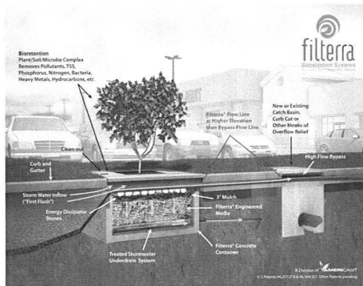
Figure 2. Diagram of the Filtterra system (Contech, 2015 via web).
