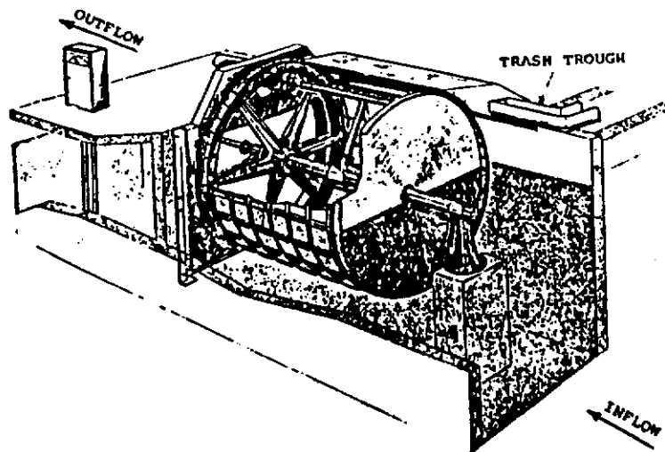
Outside-to-Inside-Flow Drum Screen (Richards, 1988)
