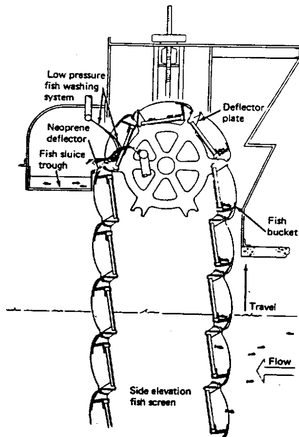
Modified Vertical Traveling Screens (White et al., 1976)
