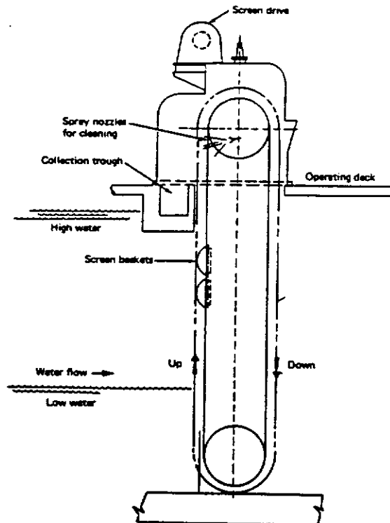
Conventional Traveling Screen (EPA, 1976)
