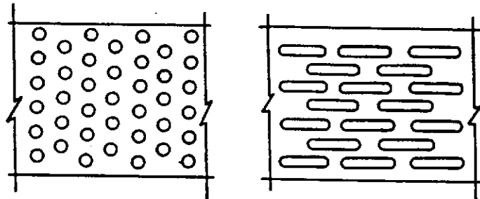
Perforations and Slots in Perforated Pipe (ASCE, 1982)
