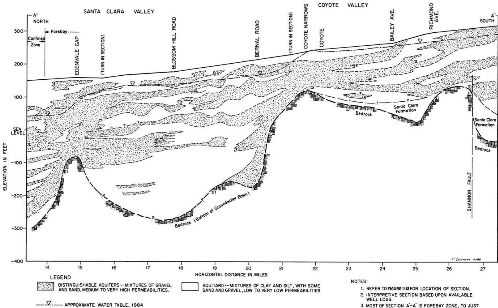
Figure 8b: Geologic Cross-section of the Santa Clara and Coyote Valleys
