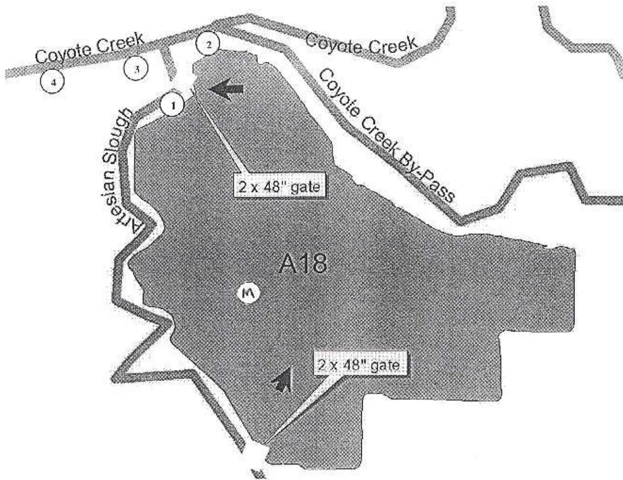
Figure 2 – Pond A18 Monitoring for North Discharge
