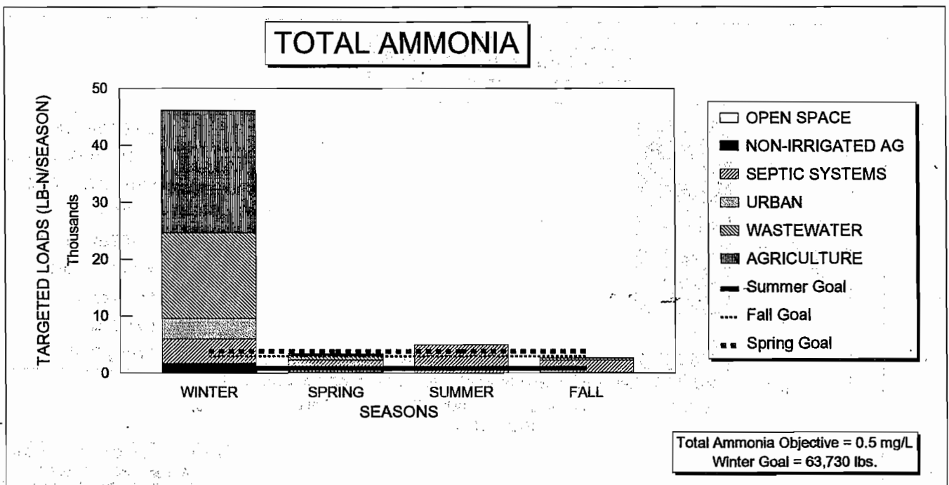
Figure 8. Reduced total nitrogen and total ammonia loads for the selected scenario in the Laguna at Occidental Road.
