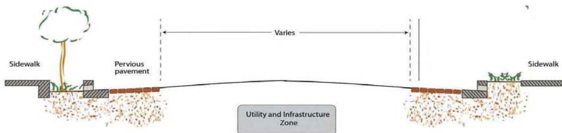
Figure 5: Possible pervious pavement design layout ( Model for Living Streets Design Manual, 2011 ).
