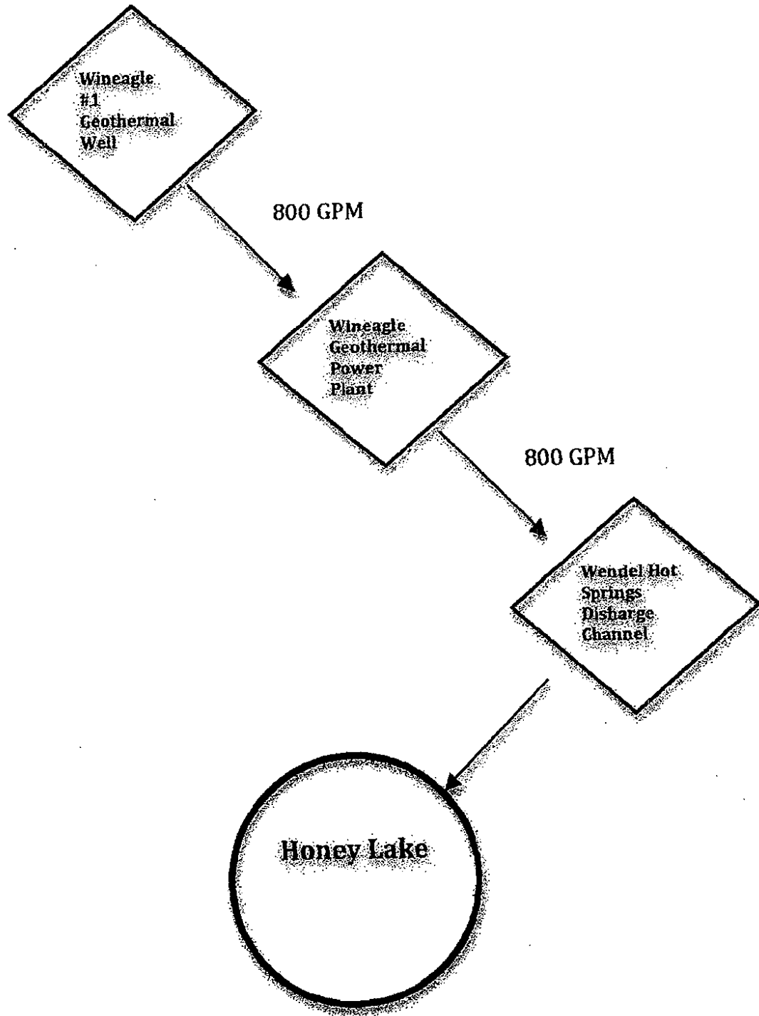
Figure C-1. Wineagle Geothermal Power Plant Flow Schematic
