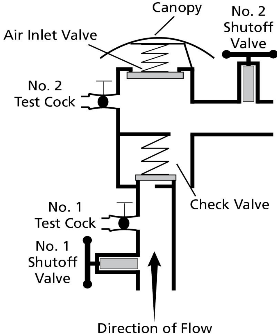
Pressure vacuum breaker backsiphonage prevention assembly 4
