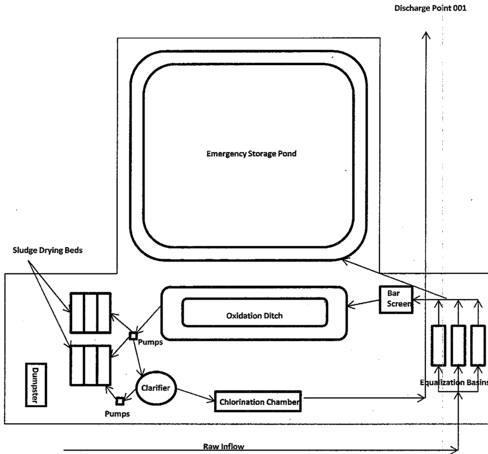
Naval Air Facility El Centro Waste Water Flow Process Schematic
