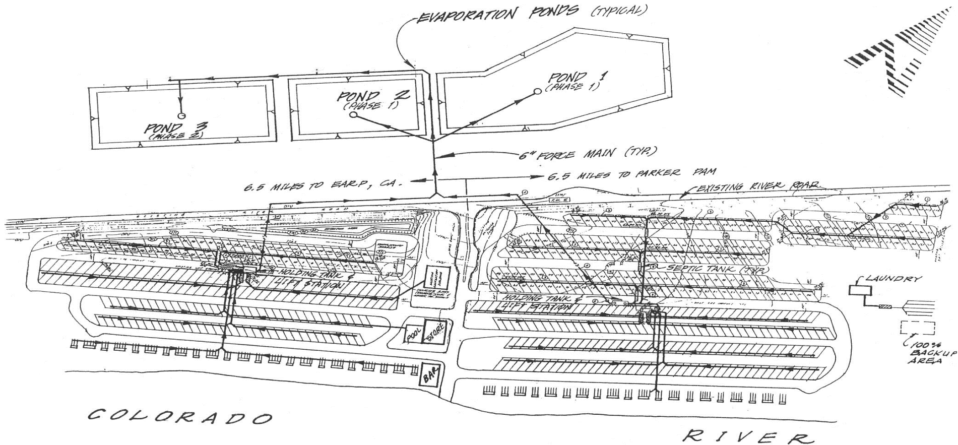
SITE MAP EMERALD COVE RESORT, L.L.C., OWNER/OPERATOR EMERALD COVE RESORT SEPTIC TANK/EVAPORATION BASIN DISPOSAL FACILITIES Northeast of Earp - San Bernardino County
