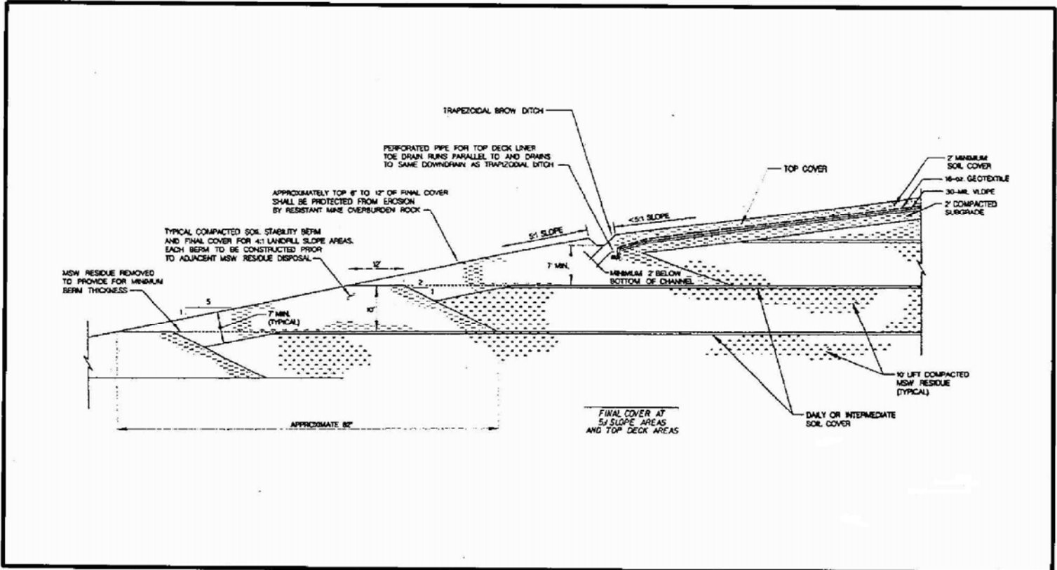
MESQUITE REGIONAL LANDFILL Permitted Final Cover System on Deck and Slope Areas Attachment 7
