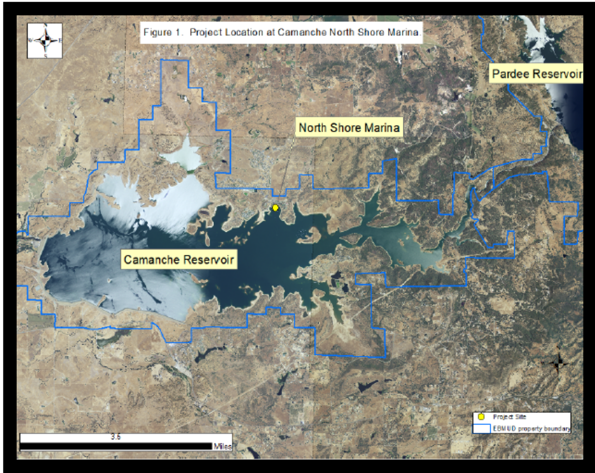
Figure 1: Vicinity Map
