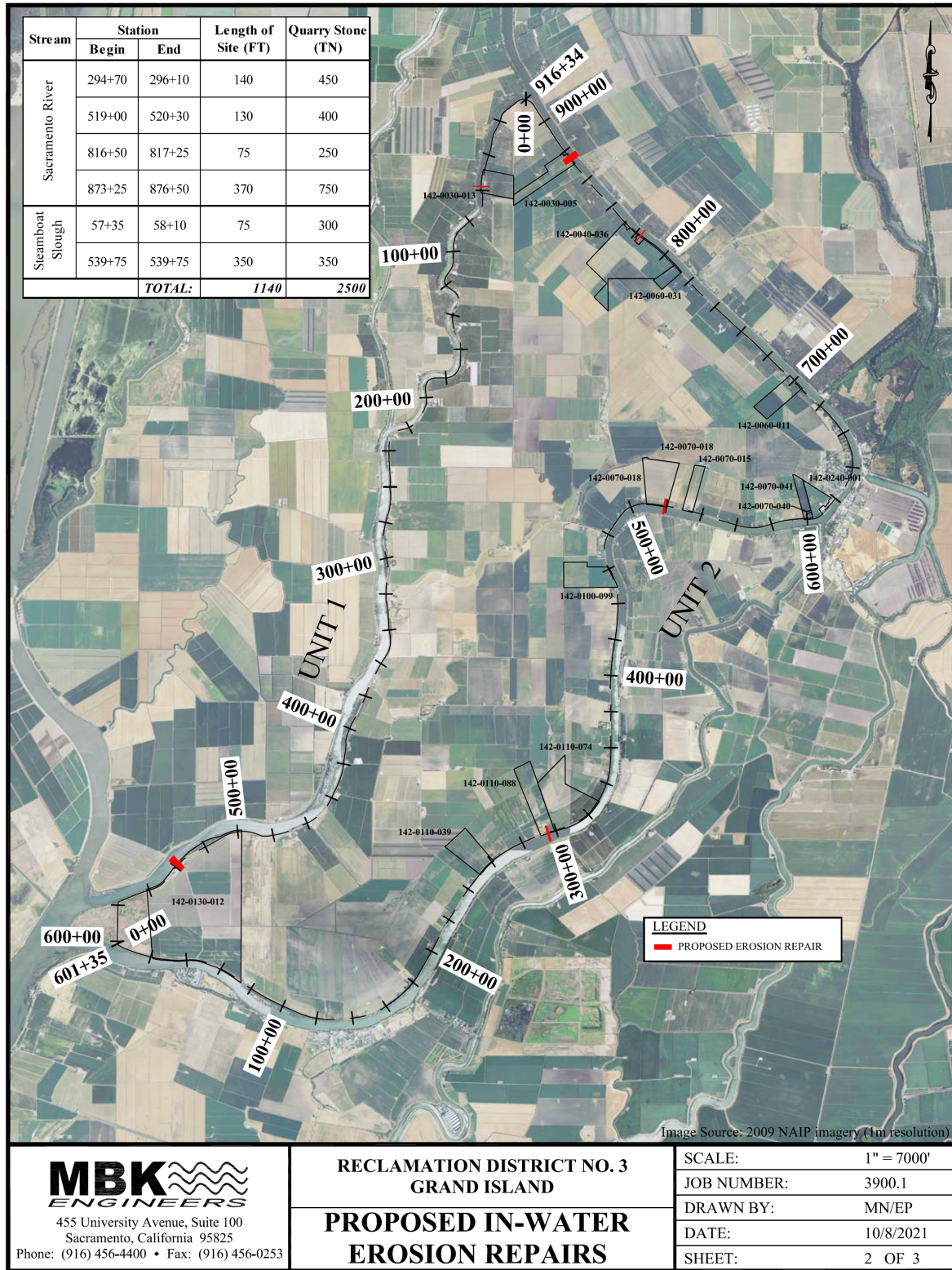
Figure 2 – Proposed In-Water Erosion Repairs
