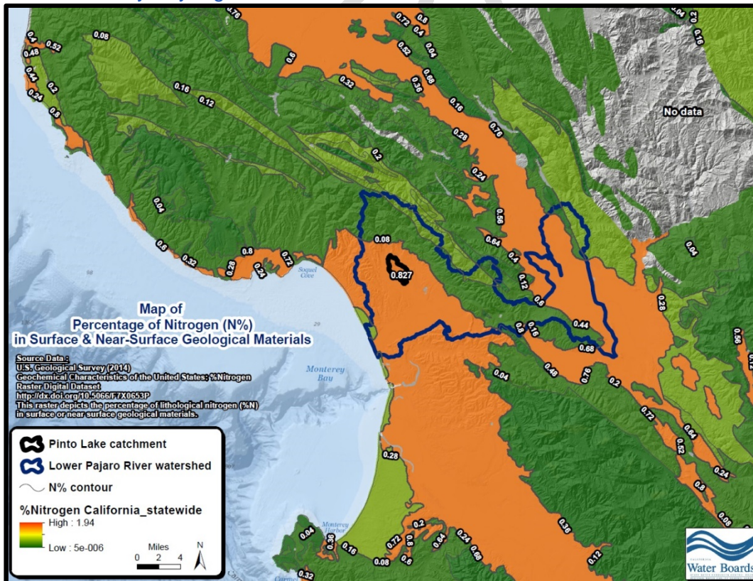
Figure 2-35. Map of estimated percentage of nitrogen (N) in surface and near-surface geologic materials of the Monterey Bay region.
