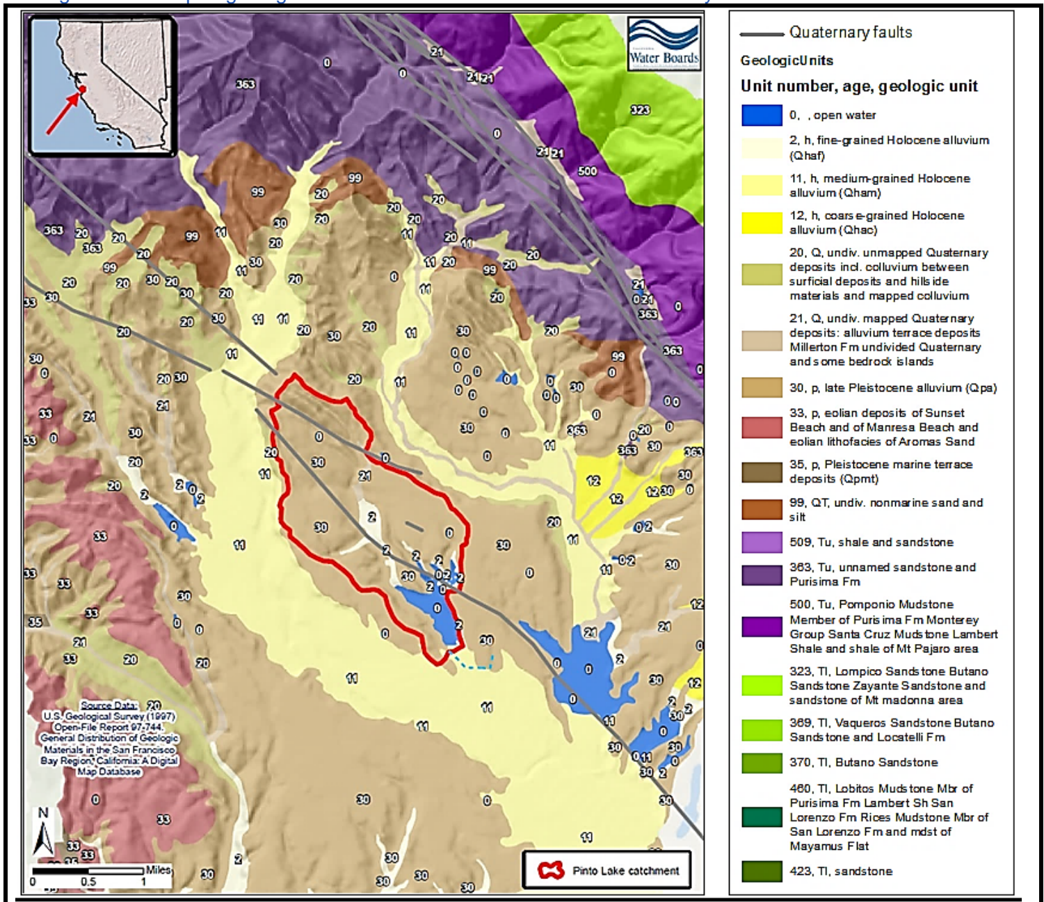
Figure 2-32. Map of geologic units in the Pinto Lake catchment and vicinity.
