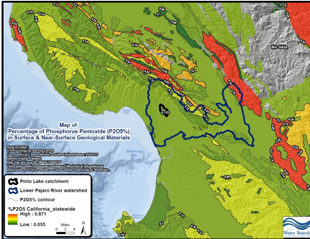
Figure 2-34. Map of percentage of phosphorus pentoxide (P 2 O 5 ) in surface and near-surface geologic materials of the Monterey Bay region.
