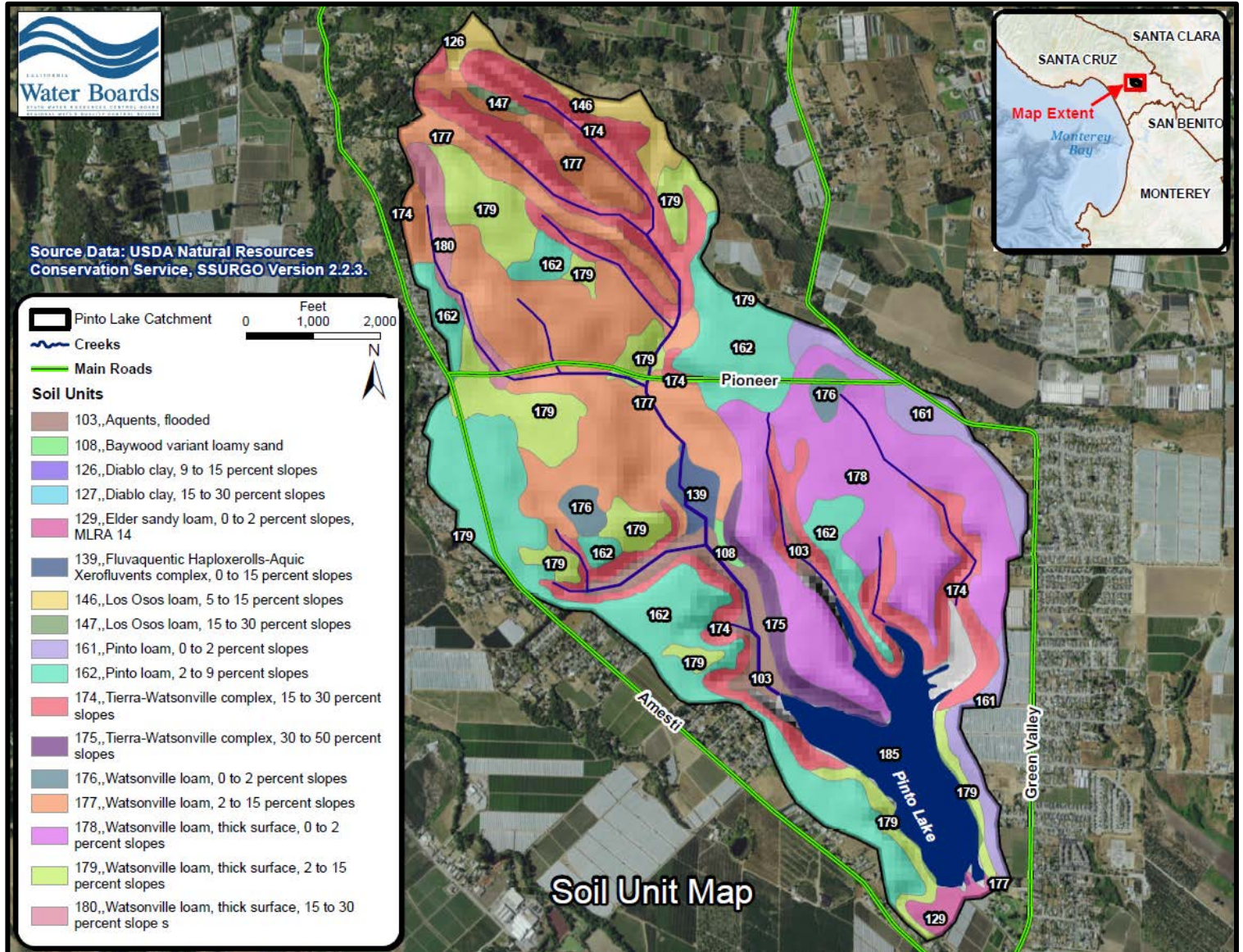
Figure 2-39. Map of soil units in the Pinto Lake catchment.
