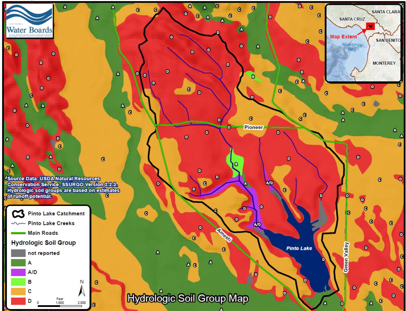
Figure 2-41. Hydrologic soils groups (HSGs) in Pinto Lake catchment and vicinity, with tabular description of HSGs.
