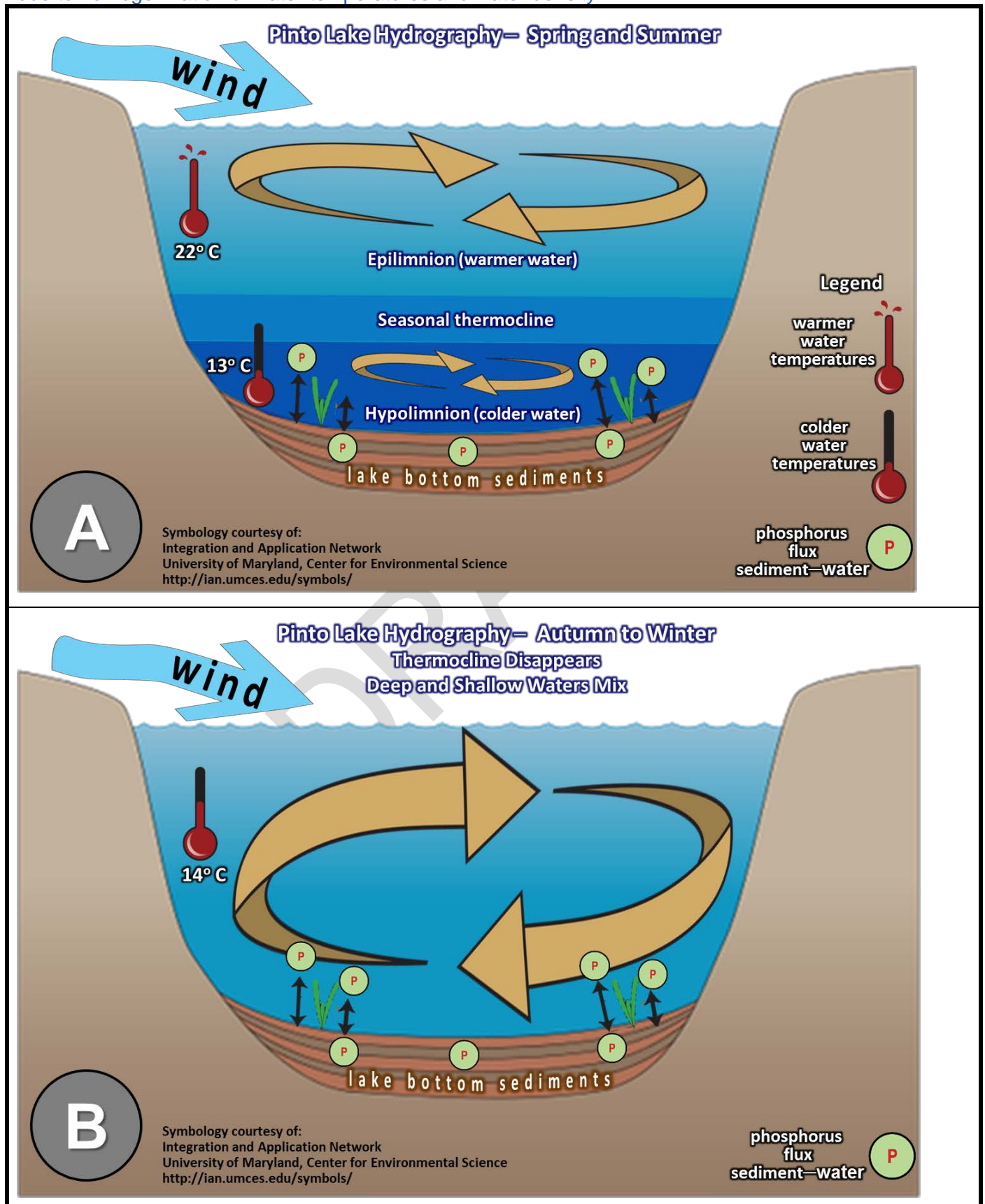
Figure 2-6. Conceptual illustration of Pinto Lake hydrography: (A) lake waters are stratified by thermal and density contrasts in the spring and summer; and (B) lake waters are mixed in the autumn and winter due to homogenization of water temperatures and water density.
