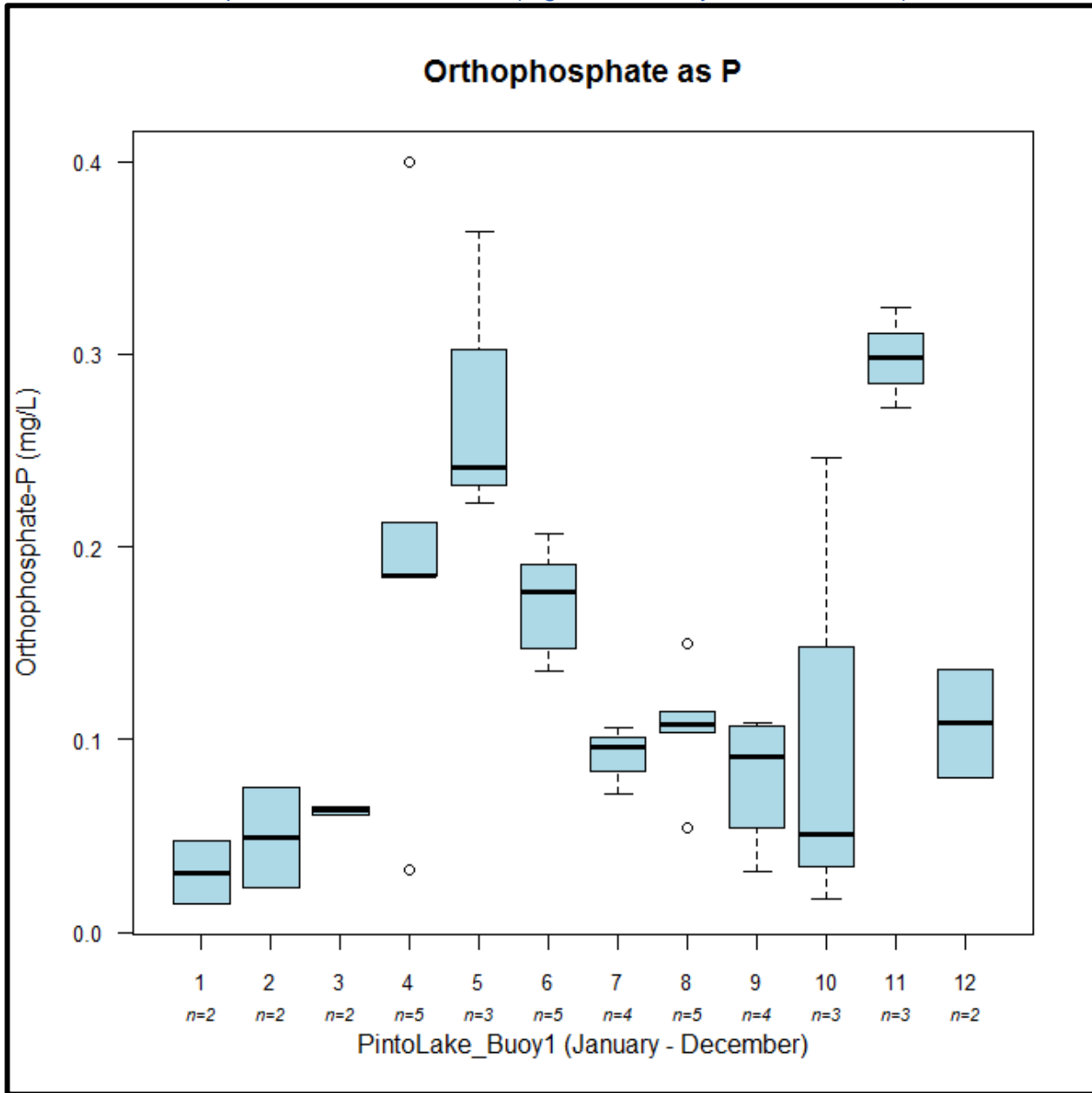
Figure 4-36. Box and whisker plot of orthophosphate as P (mg/L) values from Pinto Lake catchment site, PintoLake_Buoy1. Values plotted per month to show seasonal difference in phosphate values. Numbers on the x-axis correspond to calendar months (e.g., 1 = January, 12 = December).
