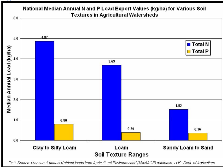
Figure 2-36. Median annual Total N and Total P export for various soil textures.
