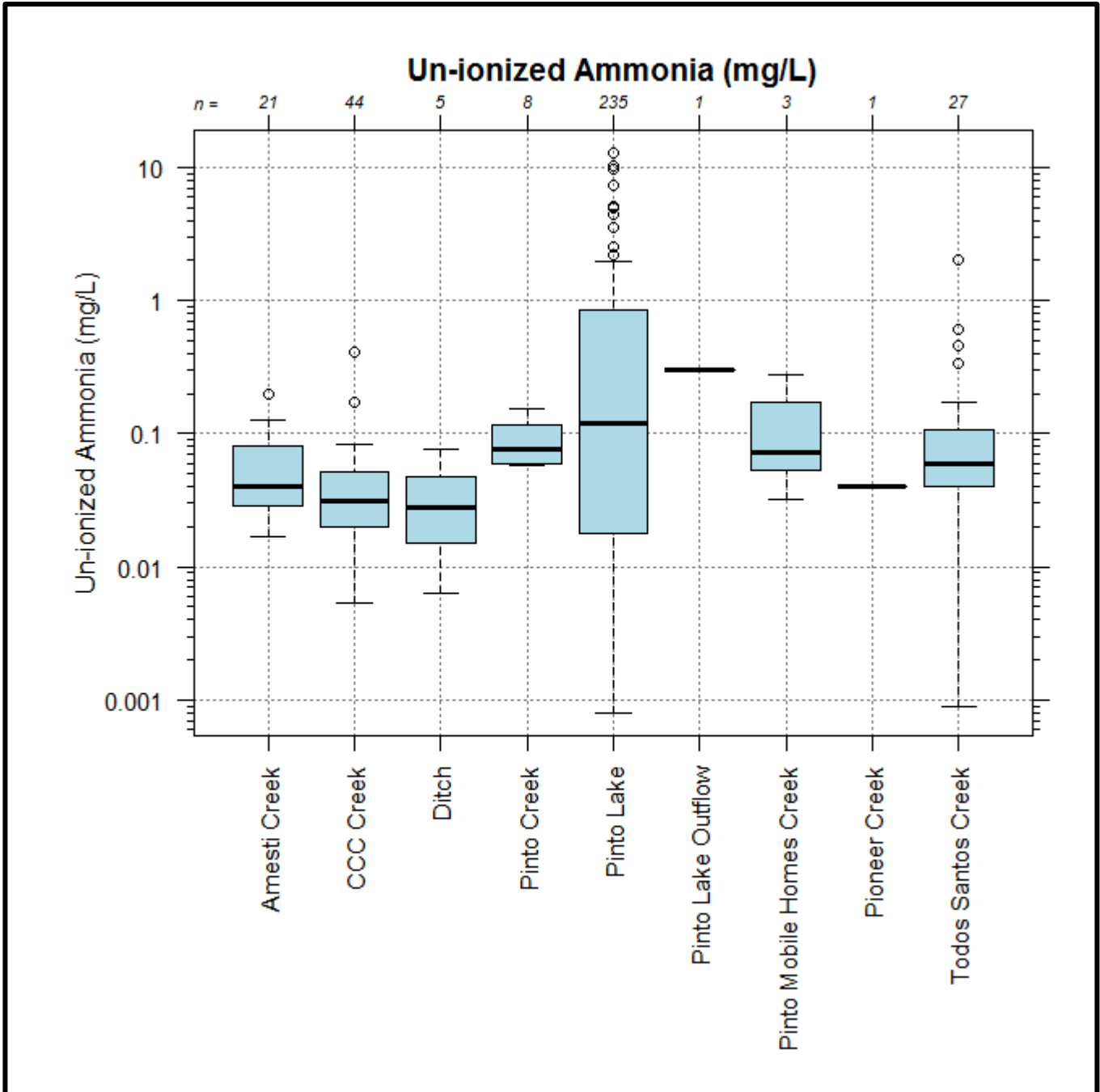
Figure 4-16. Box and whiskers plot, un-ionized ammonia water quality data, for each waterbody/surface water type (creeks, lake, drainages, etc.) sampled.
