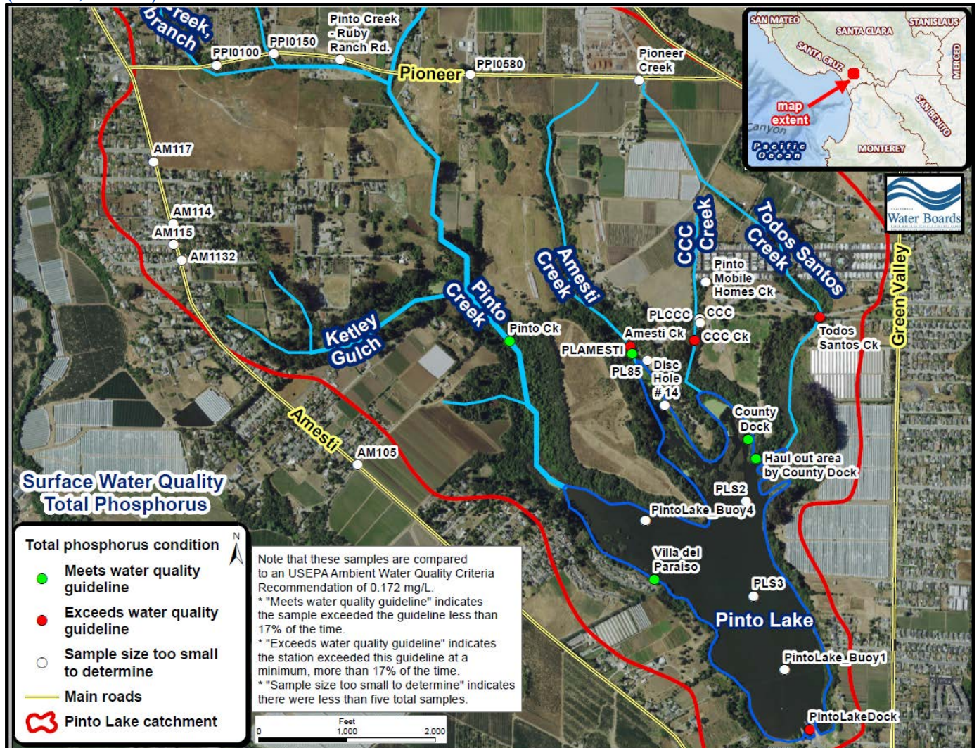
Figure 4-34. Total Phosphorus water quality standards attainment assessment of the aquatic habitat (WARM, SPWN) beneficial uses.
