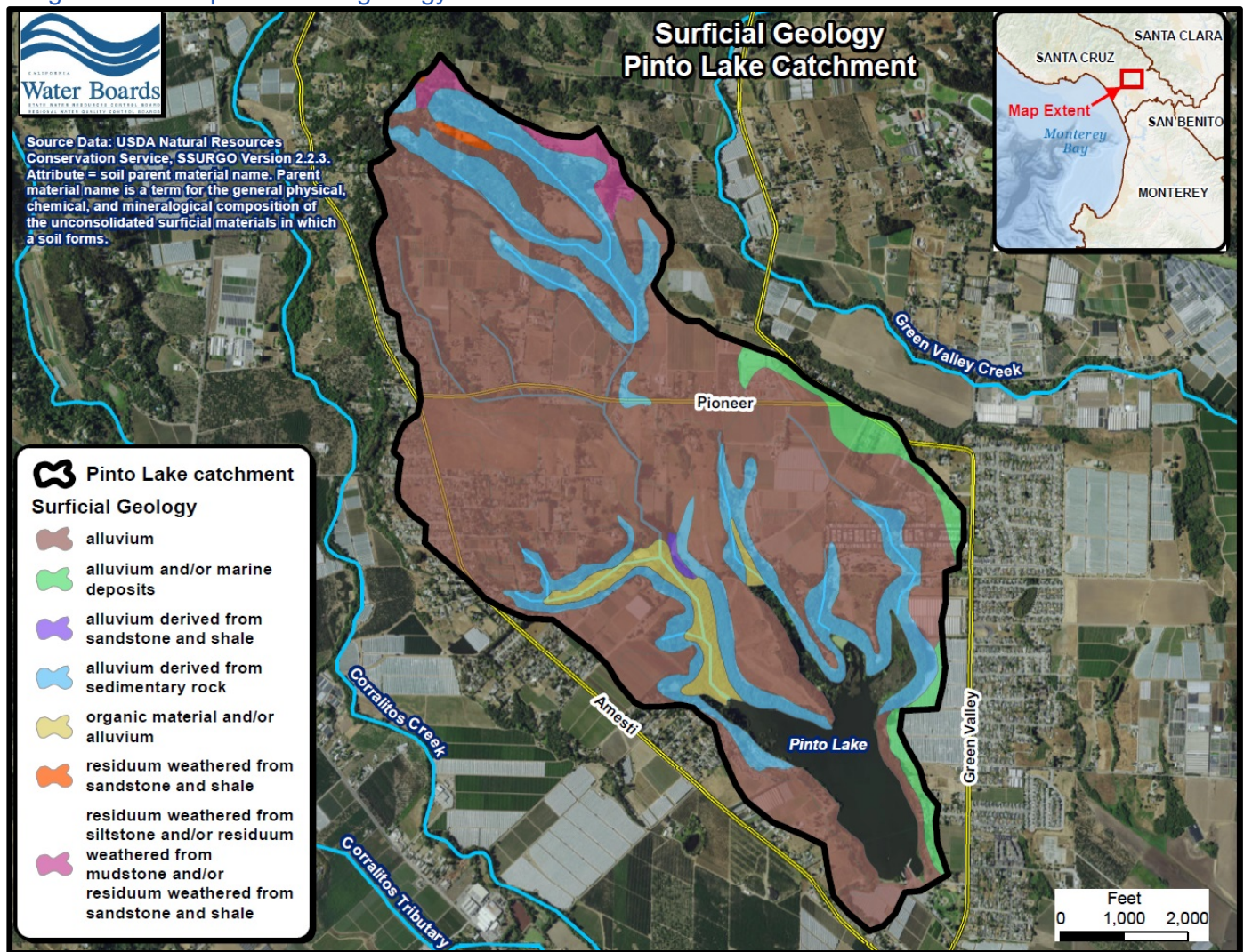
Figure 2-33. Map of surficial geology in the Pinto Lake catchment.
