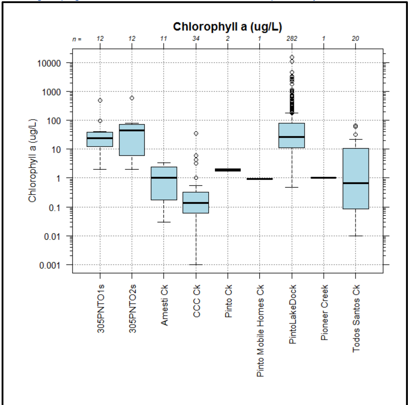
Figure 4-19. Box and whiskers plot, chlorophyll a water quality data for all surface water quality monitoring sampling sites within the Pinto Lake catchment, ordered alphabetically.
