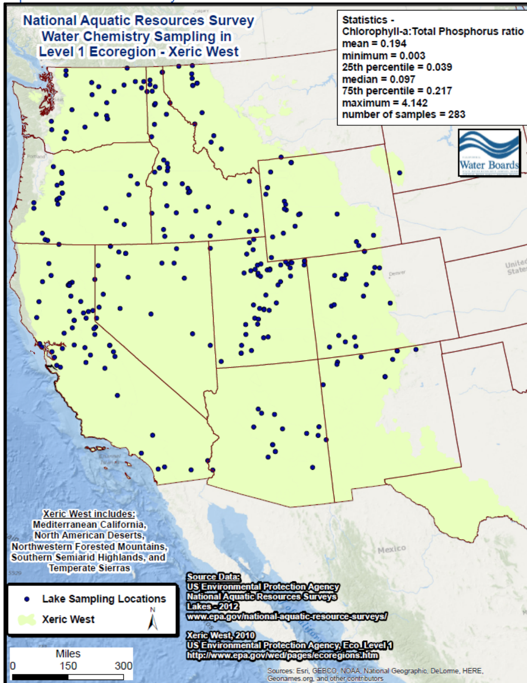
Figure 4-26. Map of USEPA Nutrient Ecoregion level 1, (Xeric West) and lakes sampled by the National Aquatic Resources Survey in 2012.
