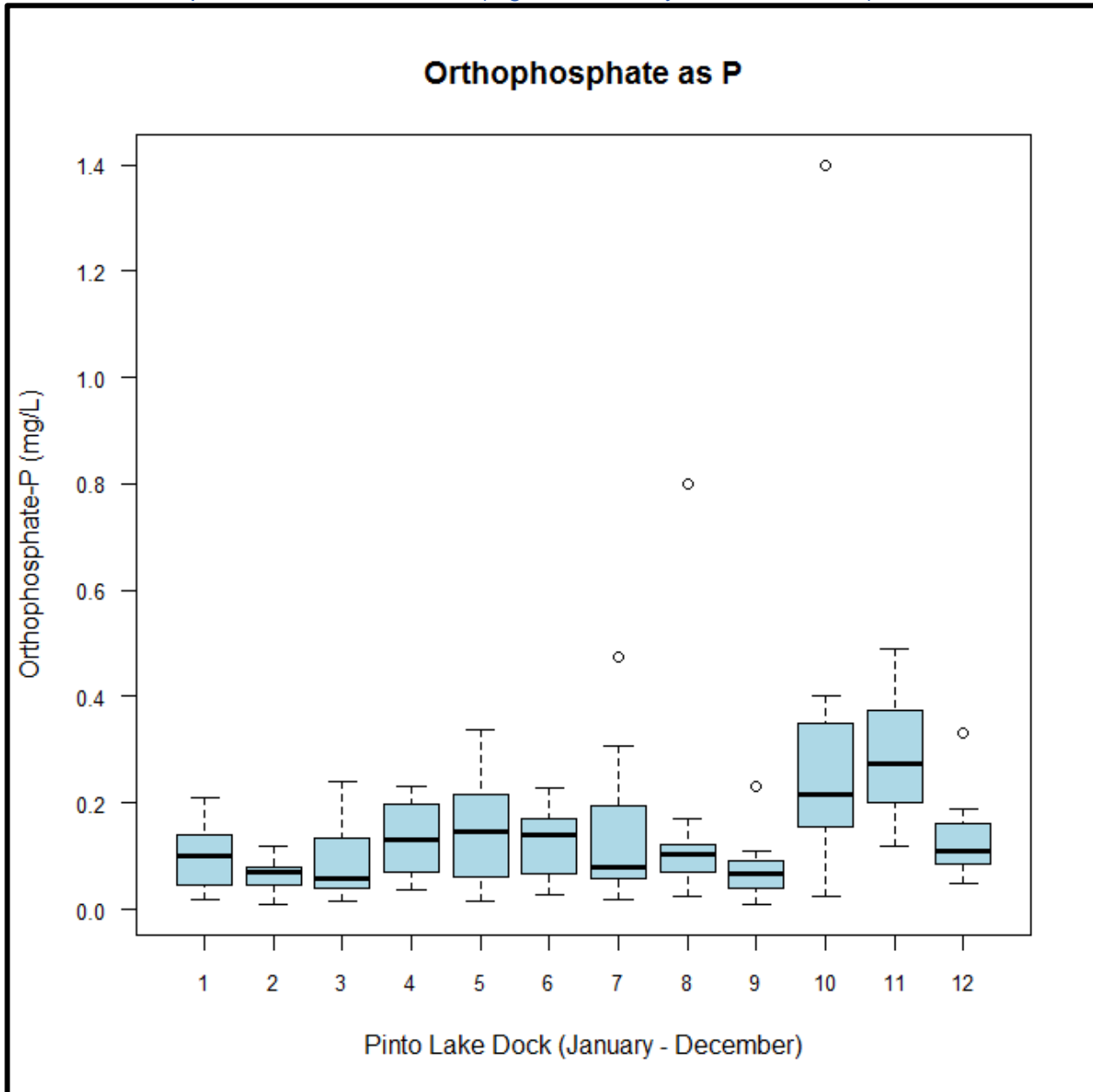
Figure 4-42. Box and whisker plot of orthophosphate as P (mg/L) values from Pinto Lake catchment site, PintoLakeDock. Values plotted per month to show seasonal difference in phosphate values. Numbers on the x-axis correspond to calendar months (e.g., 1 = January, 12 = December).
