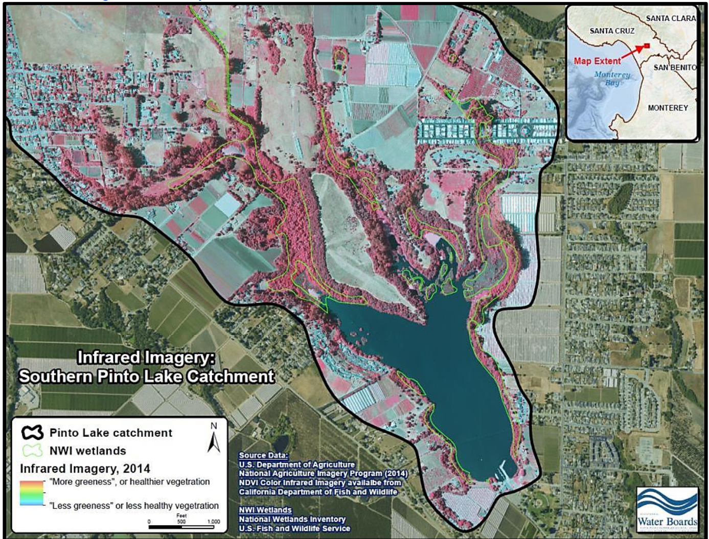
Figure 2-14. Infrared spectral image (year 2014) of the southern Pinto Lake catchment, illustrating variations in vegetative density.
