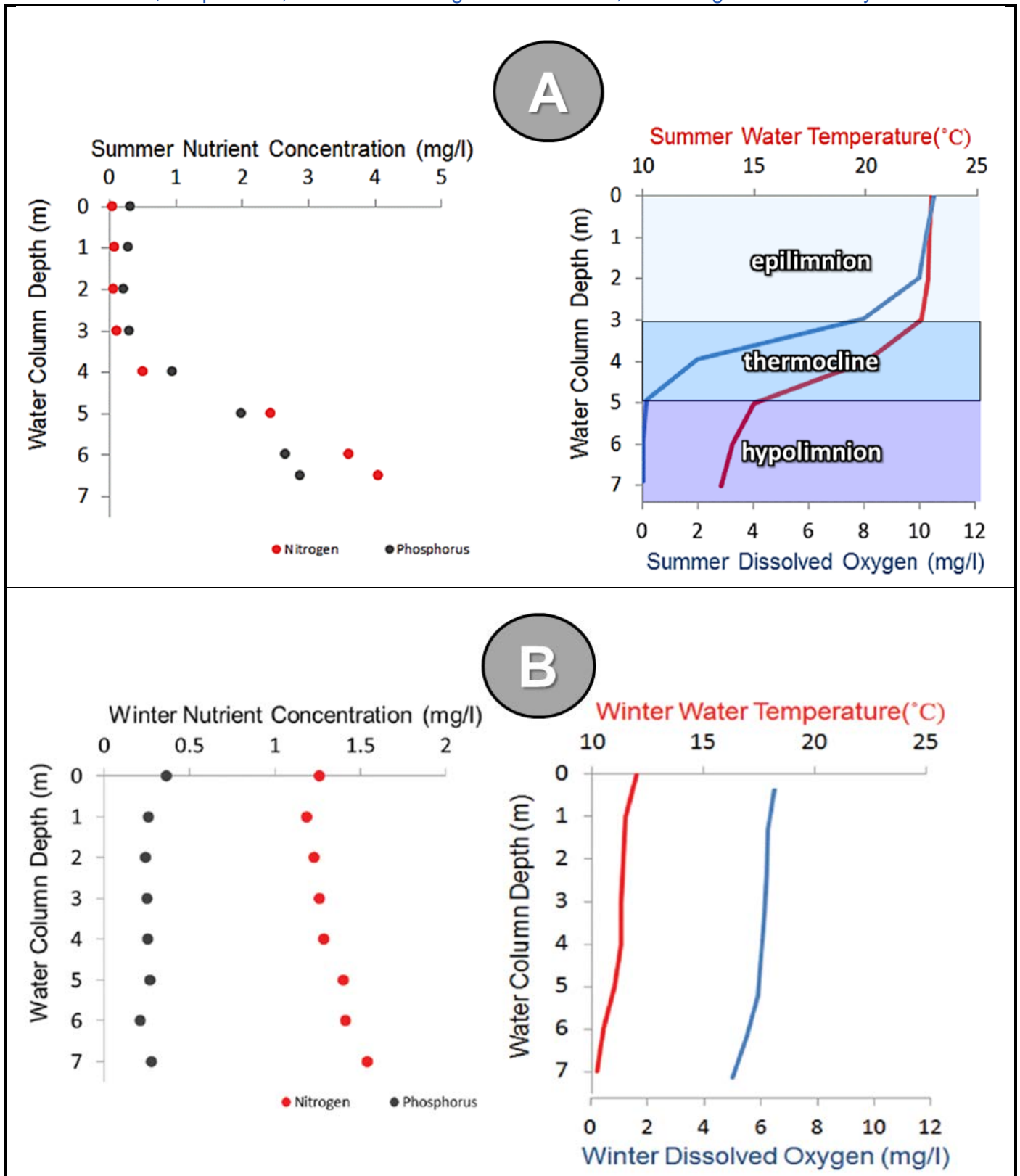
Figure 2-7. Figure from CSUMB and Resource Conservation District of Santa Cruz County, 2013. (A) Summer nutrient concentrations, temperature, and dissolved oxygen illustrating thermal stratification of lake waters and nutrient-enrichment of deep waters (hypolimnion); and (B) Winter nutrient concentrations, temperature, and dissolved oxygen in Pinto Lake, illustrating a well mixed system.
