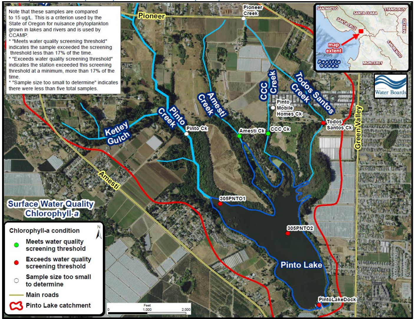
Figure 4-37. Chlorophyll-a water quality standards attainment assessment of the aquatic habitat (WARM, SPWN), recreational (REC-1) and wildlife habitat (WILD) beneficial uses.
