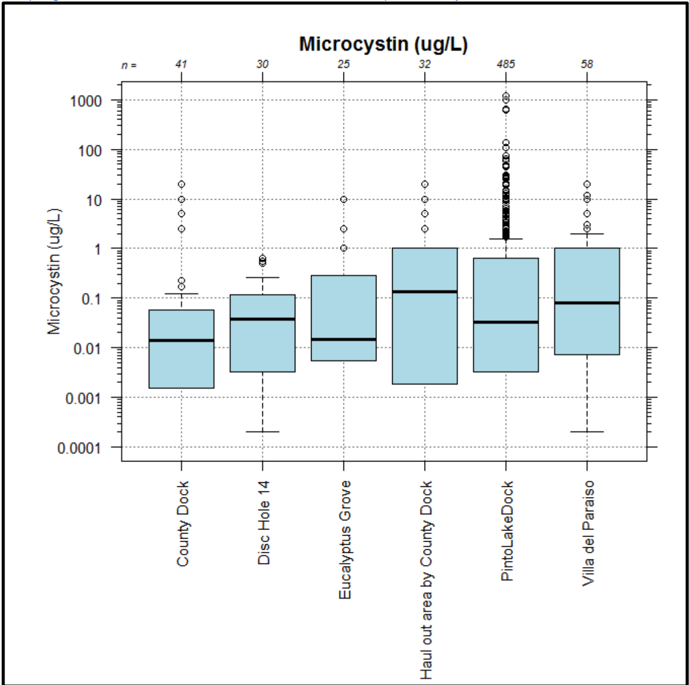
Figure 4-21. Box and whiskers plot, microcystin water quality data for all surface water quality monitoring sampling sites within the Pinto Lake catchment, ordered alphabetically.
