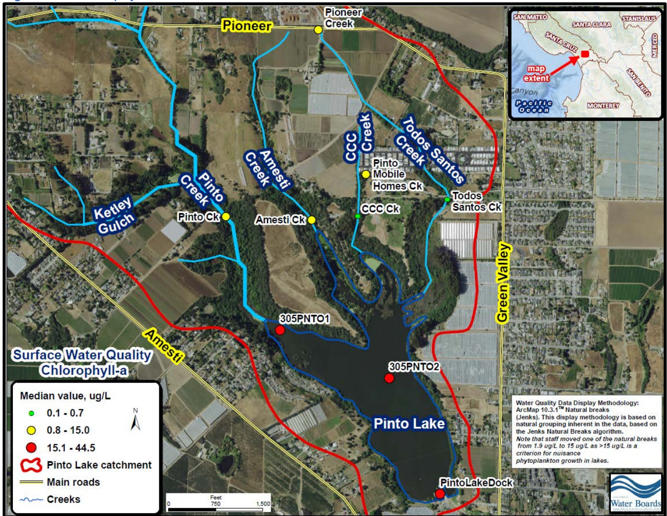
Figure 4-8. Chlorophyll-a concentrations in the Pinto Lake catchment.
