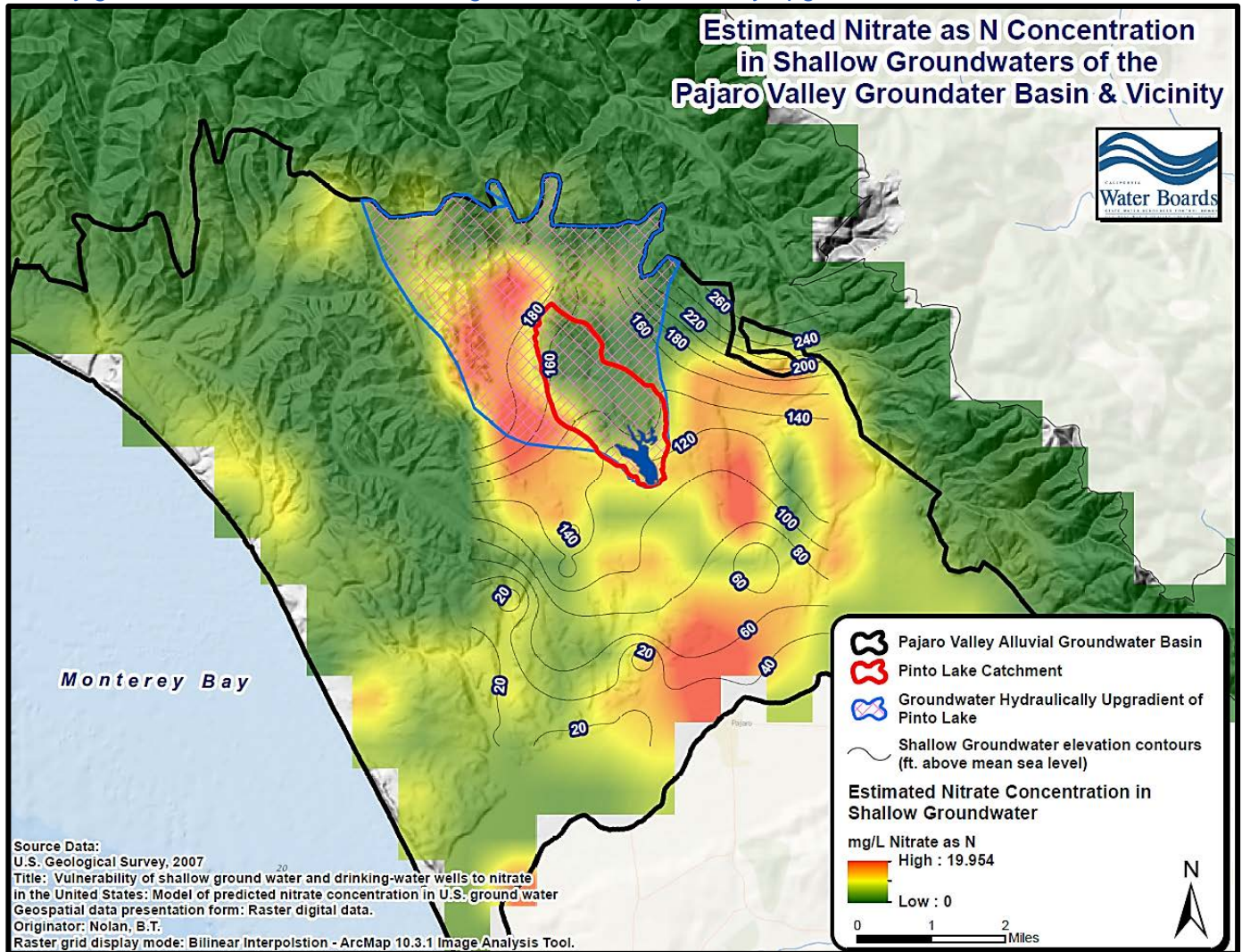
Figure 2-31. Map illustrating estimated nitrate as N concentrations in shallow groundwater of the Pajaro Valley groundwater basin, and shallow groundwater hydraulically upgradient from Pinto Lake.
