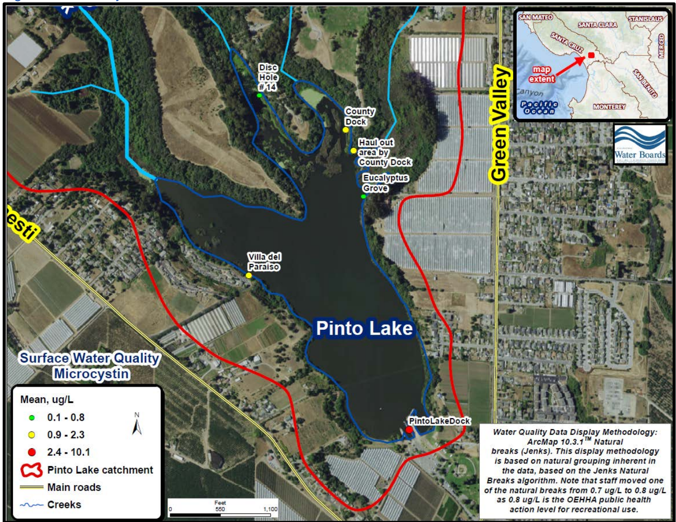
Figure 4-9. Microcystin concentrations in the Pinto Lake catchment.
