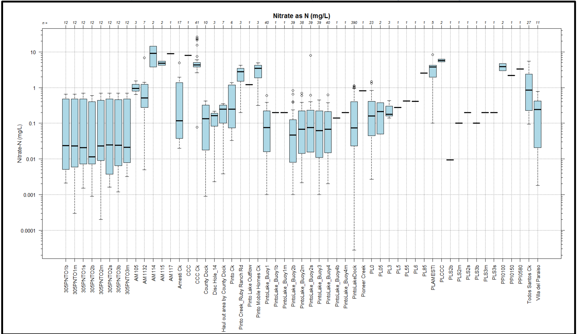
Figure 4-13. Box and whiskers plot, nitrate as N water quality data for all surface water quality monitoring sampling sites within the Pinto Lake catchment, ordered alphabetically. For reference, the nitrate as N water quality standard for drinking water is 10 mg/L.
