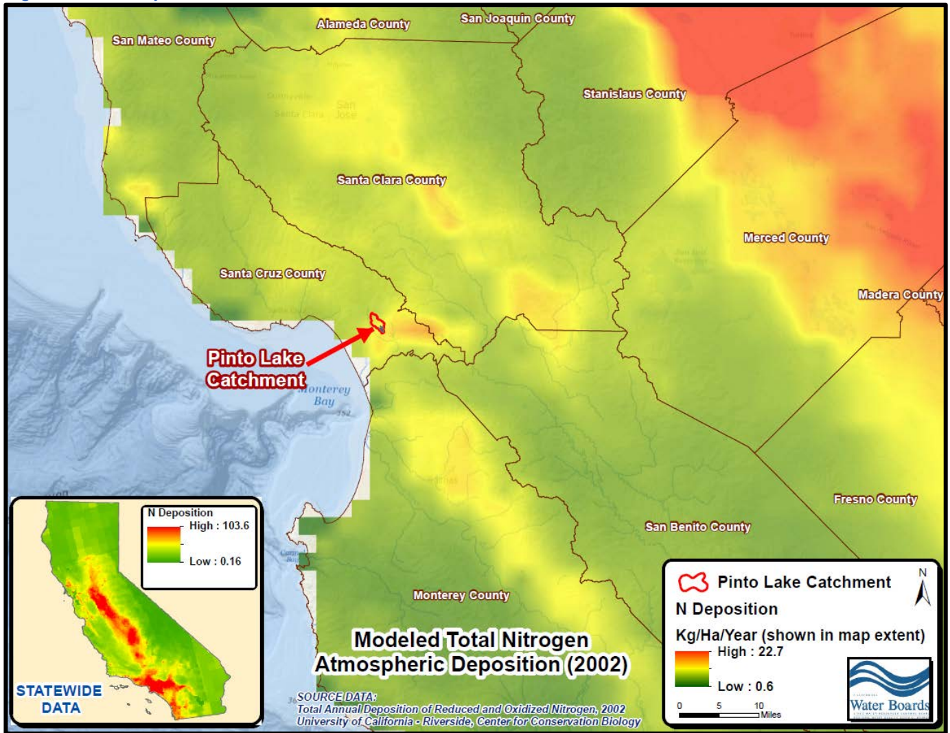
Figure 2-27. Estimated atmospheric deposition of nitrogen as N (units=kg/Ha/year) in the Monterey Bay region and vicinity.
