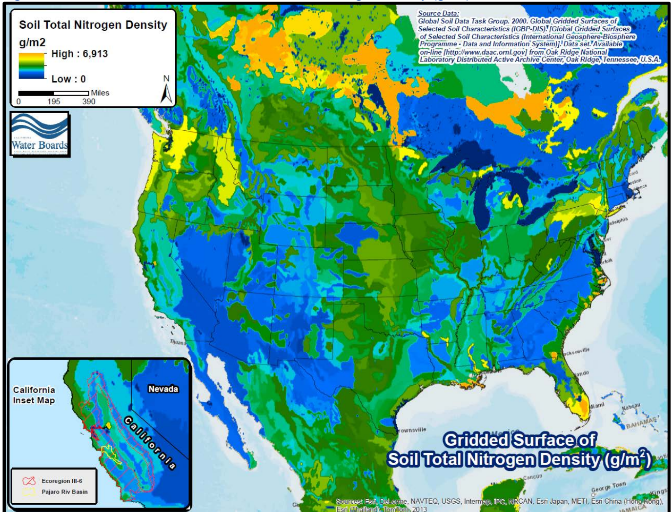
Figure 2-46. Gridded surface of estimated soil total nitrogen density ( \text{g/m}^2 ), from the IGBP-DIS dataset.
