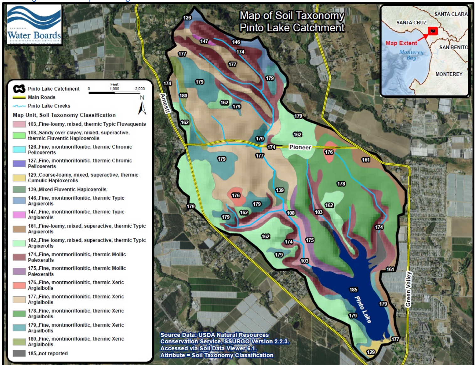
Figure 2-42. Map showing soil taxonomic classifications in the Pinto Lake catchment.
