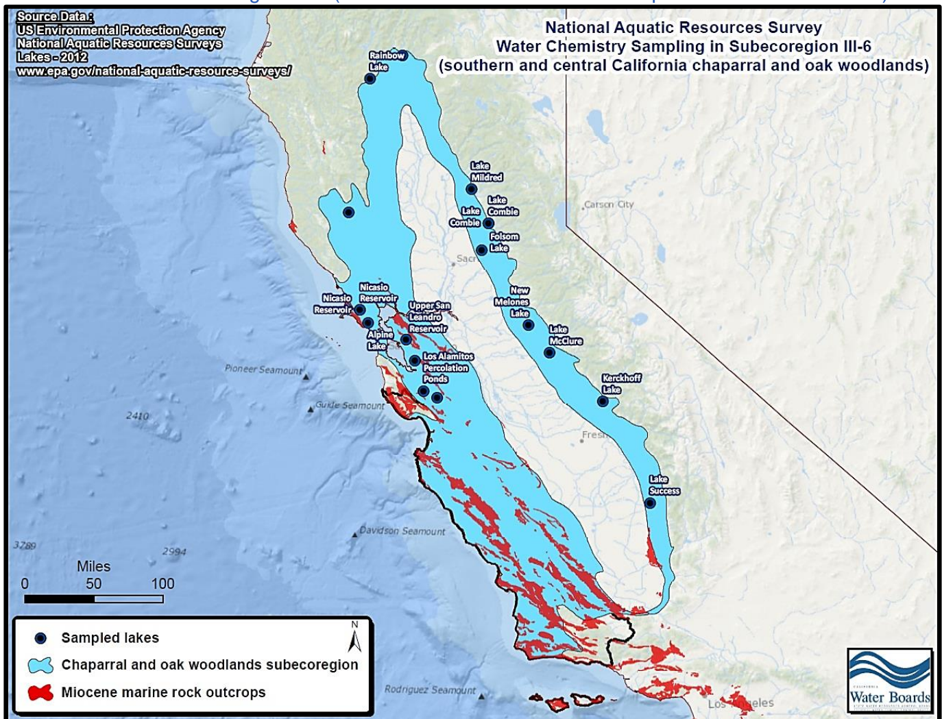
Figure 2-25. Map showing lake sample locations for USEPA National Lake Assessment (2012), for lakes located in nutrient subecoregion III-6 (southern and central California chaparral and oak woodlands).
