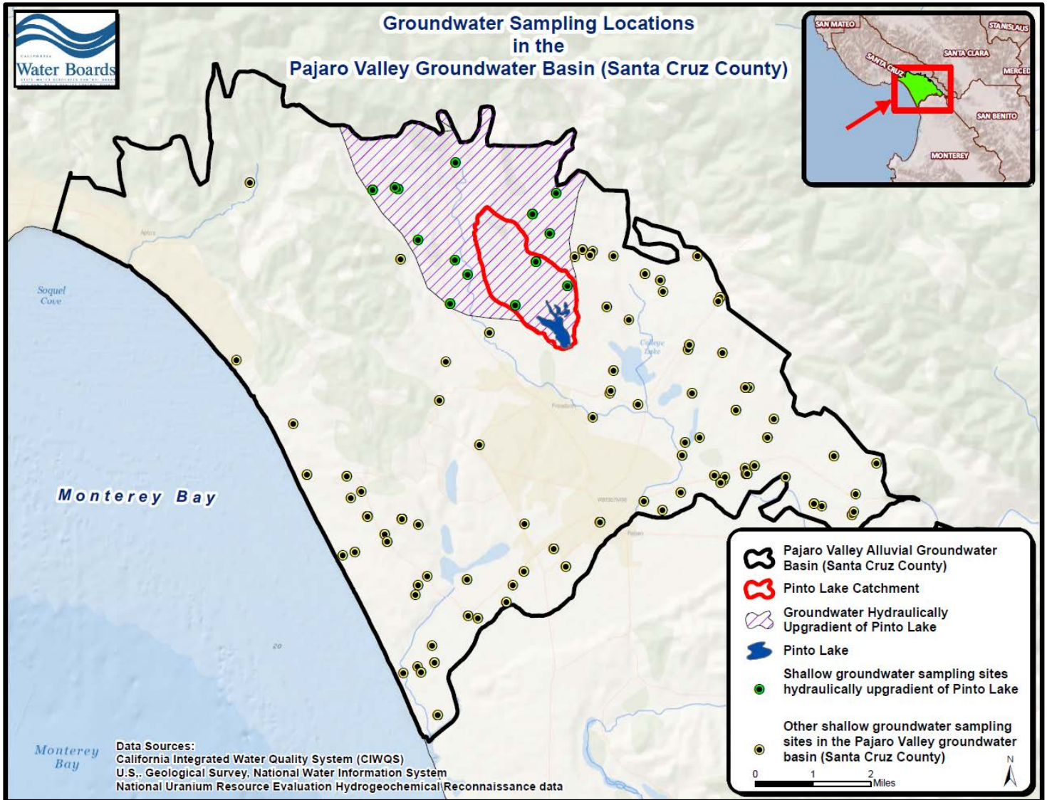
Figure 4-28. Higher resolution map view of sampling sites in the Pajaro Valley groundwater basin used for statistical summaries of nutrient water quality in groundwaters. Statistical summaries are presented in Table 4-19 and Table 4-20.
