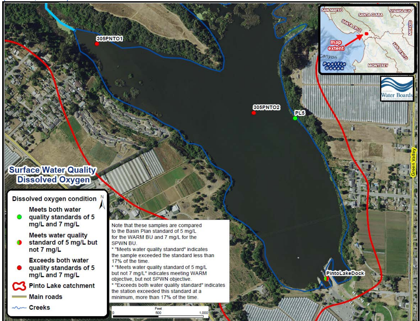
Figure 4-36. Dissolved oxygen water quality standards attainment assessment of the aquatic habitat (WARM, SPWN) beneficial uses.
