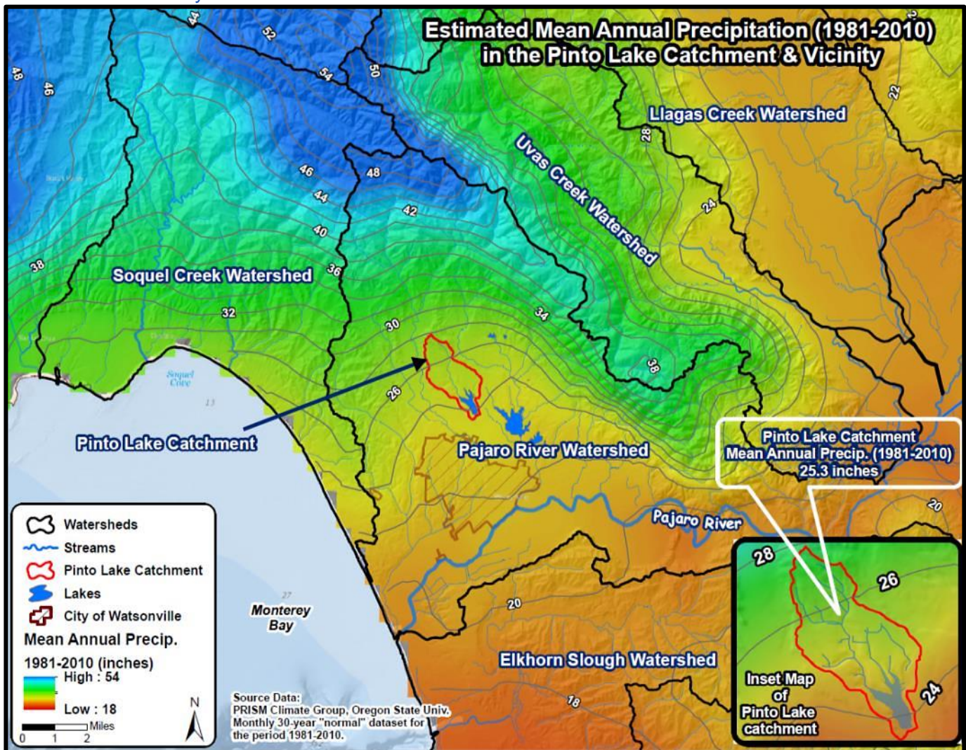
Figure 2-26 . Estimated mean annual precipitation for the 30 year period of 1981-2010 in the Pinto Lake catchment and vicinity.
