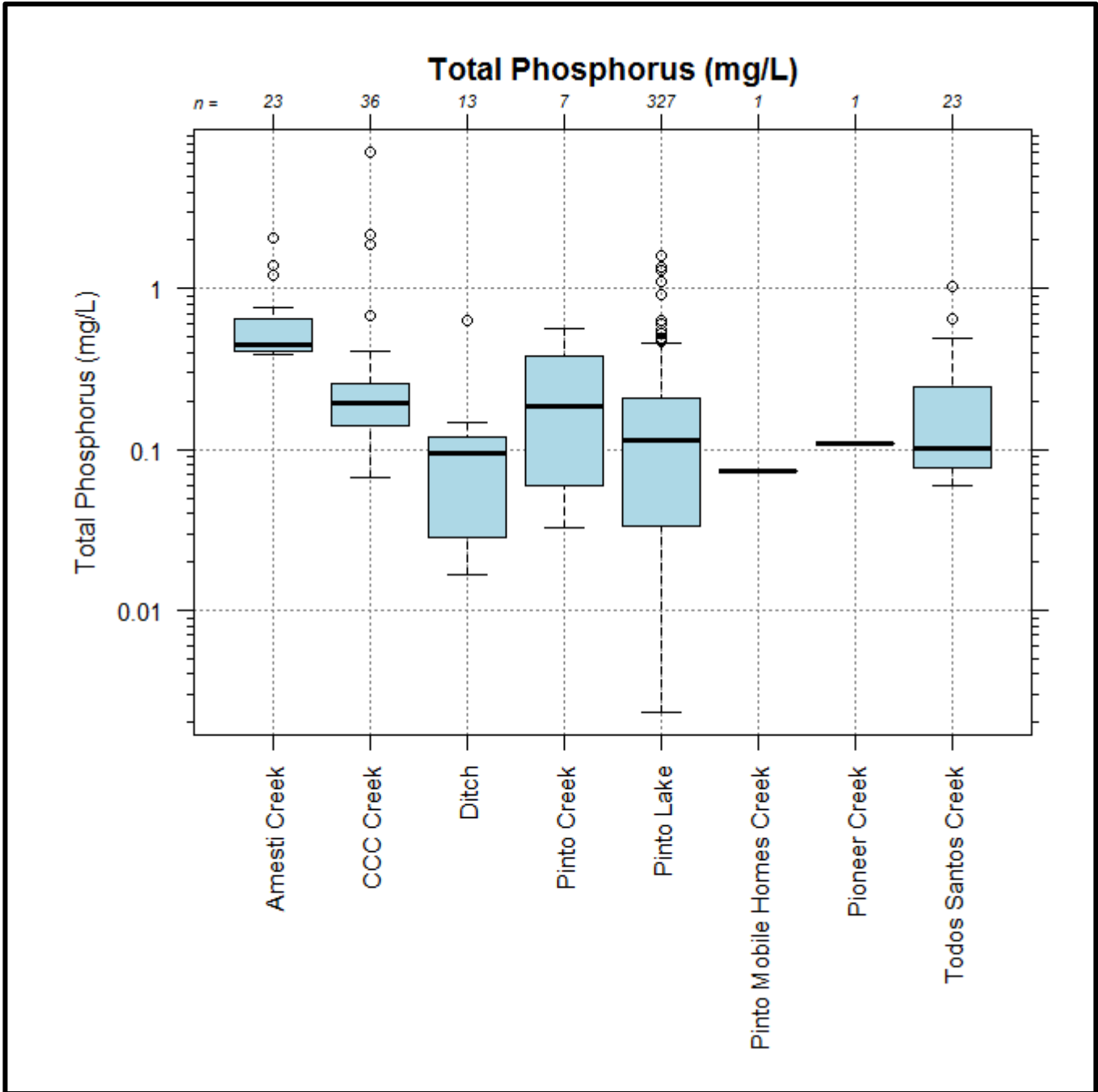
Figure 4-11. Box and whiskers plots, total phosphorus water quality data, for each waterbody/surface water type (creeks, lake, drainages, etc.) sampled. Tributaries Amesti Creek, CCC Creek and Pinto Creek had the highest average (and median) total phosphorous concentrations of all waterbody/surface water types sampled.
