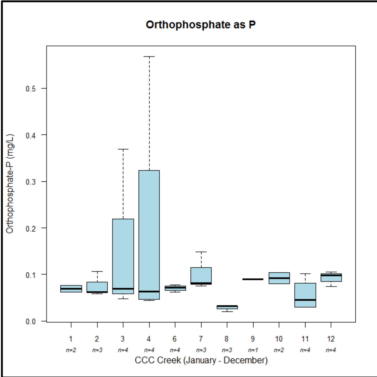
Figure 4-35. Box and whisker plot of orthophosphate as P (mg/L) values from Pinto Lake catchment site, CCC Creek. Values plotted per month to show seasonal difference in phosphate values. Numbers on the x-axis correspond to calendar months (e.g., 1 = January, 12 = December).
