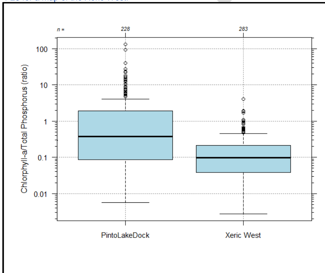
Figure 4-24. Boxplot showing values of chlorophyll-a to total phosphorus (Chl:TP) ratios in Pinto Lake at the sampling station PintoLakeDock and a grouping of values from the Ecoregion Xeric West. See Figure 4-26 for a map of the Xeric West.
