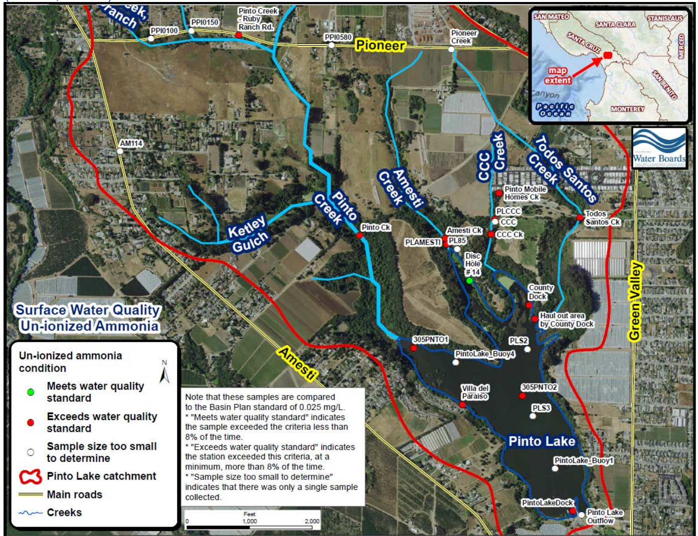
Figure 4-33. Un-ionized ammonia, water quality standards attainment assessment of the aquatic habitat (WARM, SPWN) beneficial uses.
