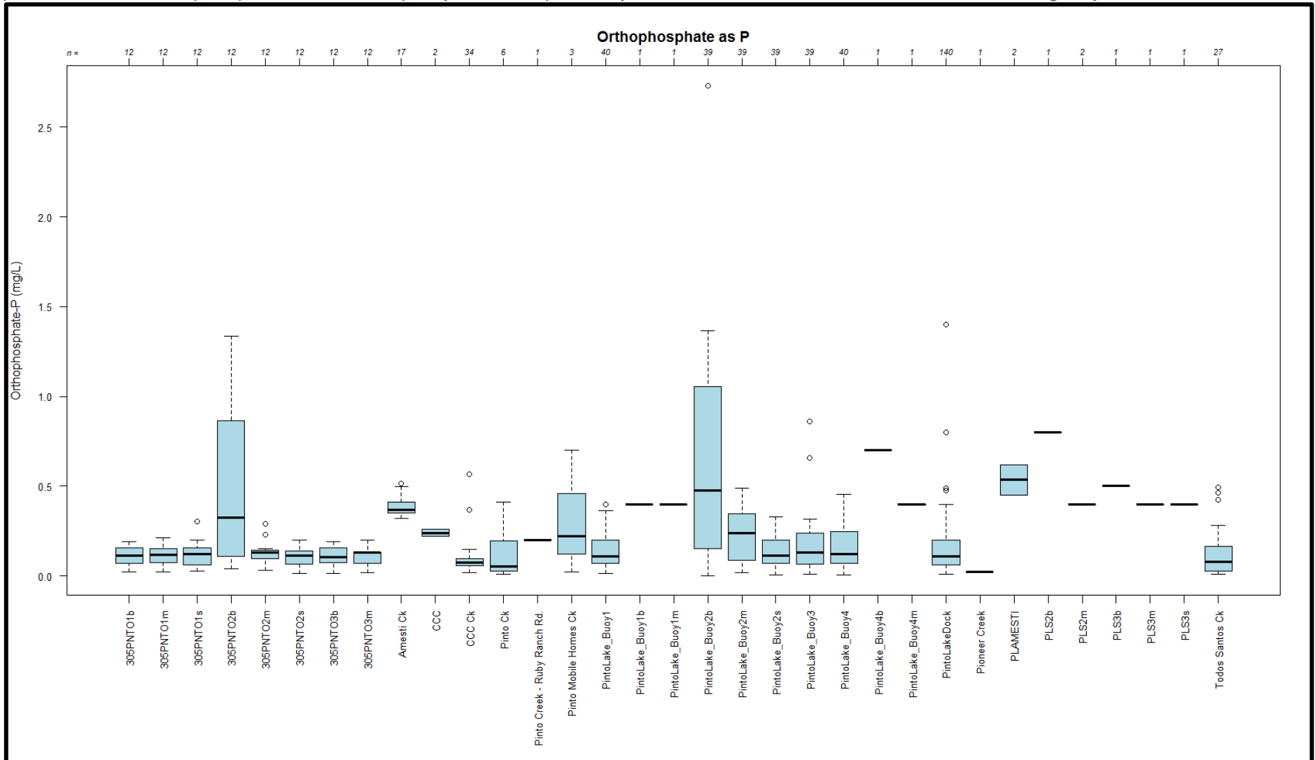
Figure 4-17. Box and whiskers plot, orthophosphate as P water quality data for all surface water quality monitoring sampling sites within the Pinto Lake catchment, ordered alphabetically. For reference, the orthophosphate as P guideline concentration of 0.06 mg/L represents the 75% percentile of all orthophosphate lake water quality criteria reported by states to the U.S. Environmental Protection Agency.
