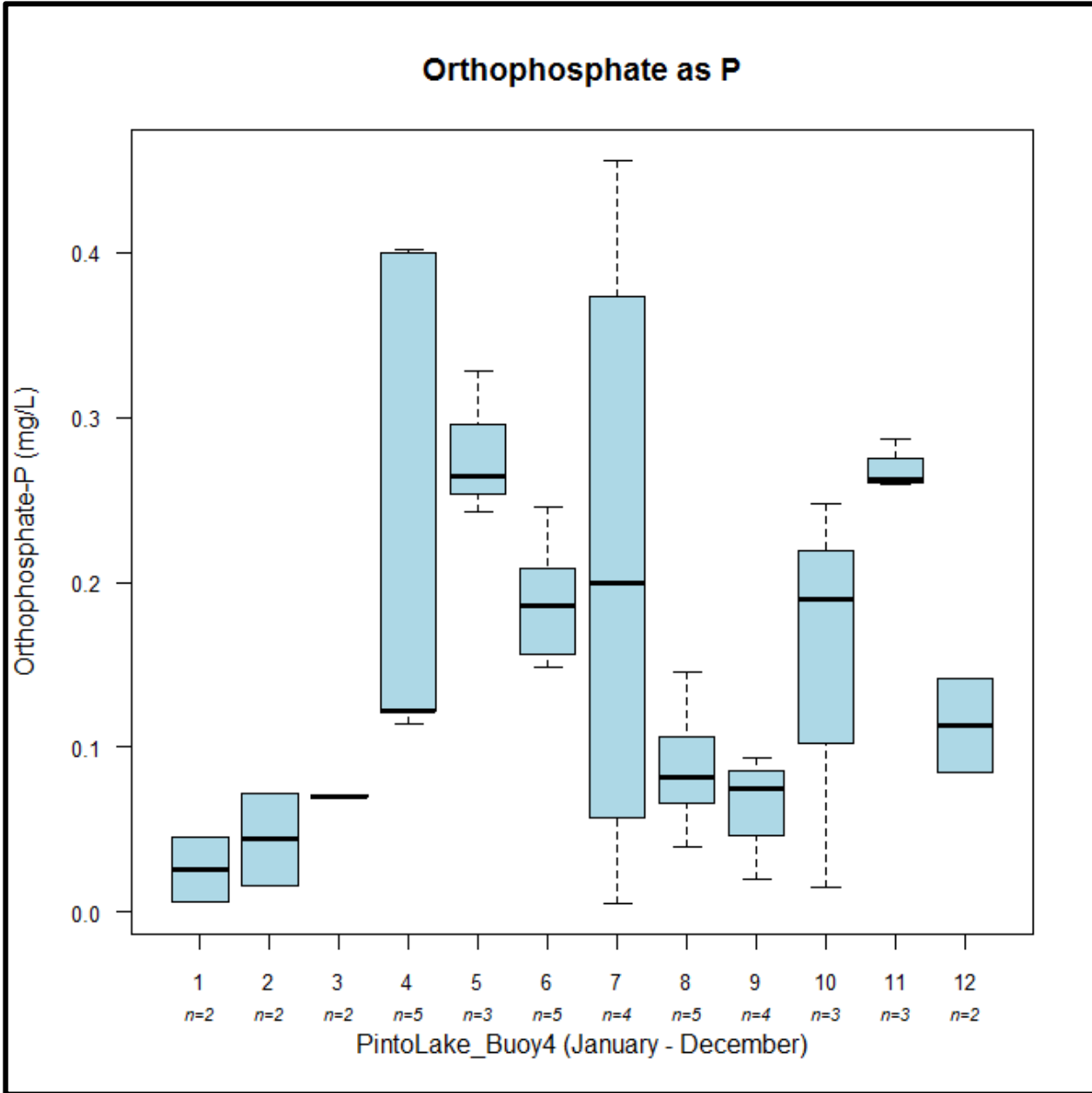
Figure 4-41. Box and whisker plot of orthophosphate as P (mg/L) values from Pinto Lake catchment site, PintoLake_Buoy4. Values plotted per month to show seasonal difference in phosphate values. Numbers on the x-axis correspond to calendar months (e.g., 1 = January, 12 = December).
