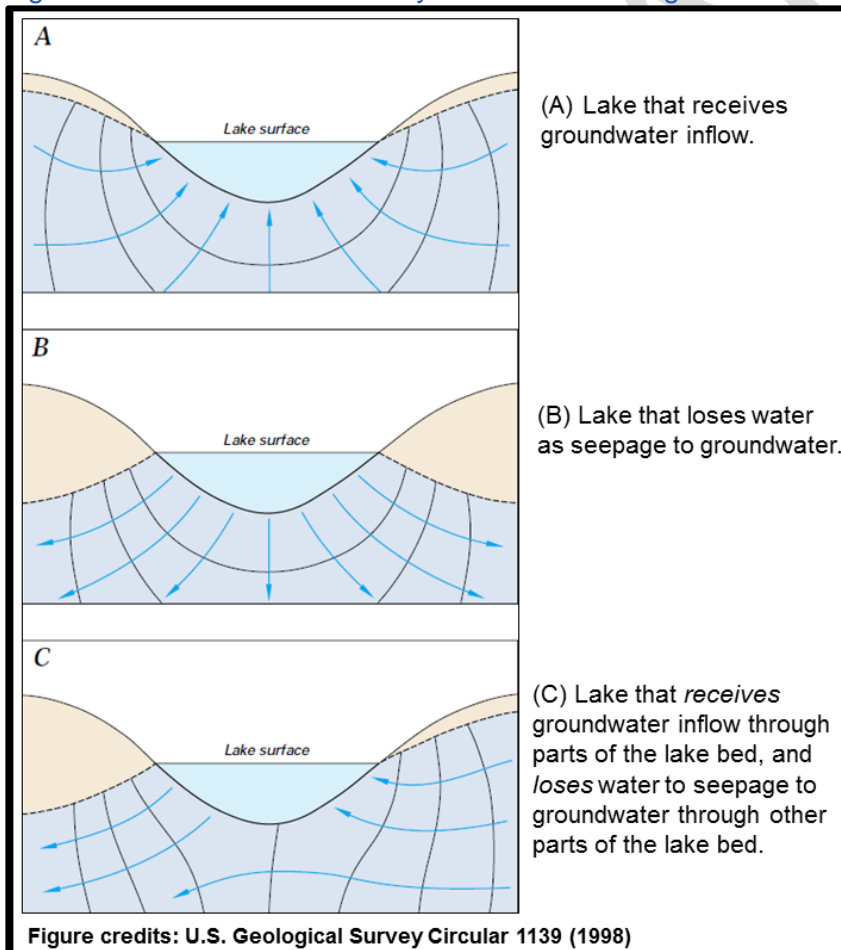
Figure 2-28. Lakes are intimately connected to the groundwater system.
