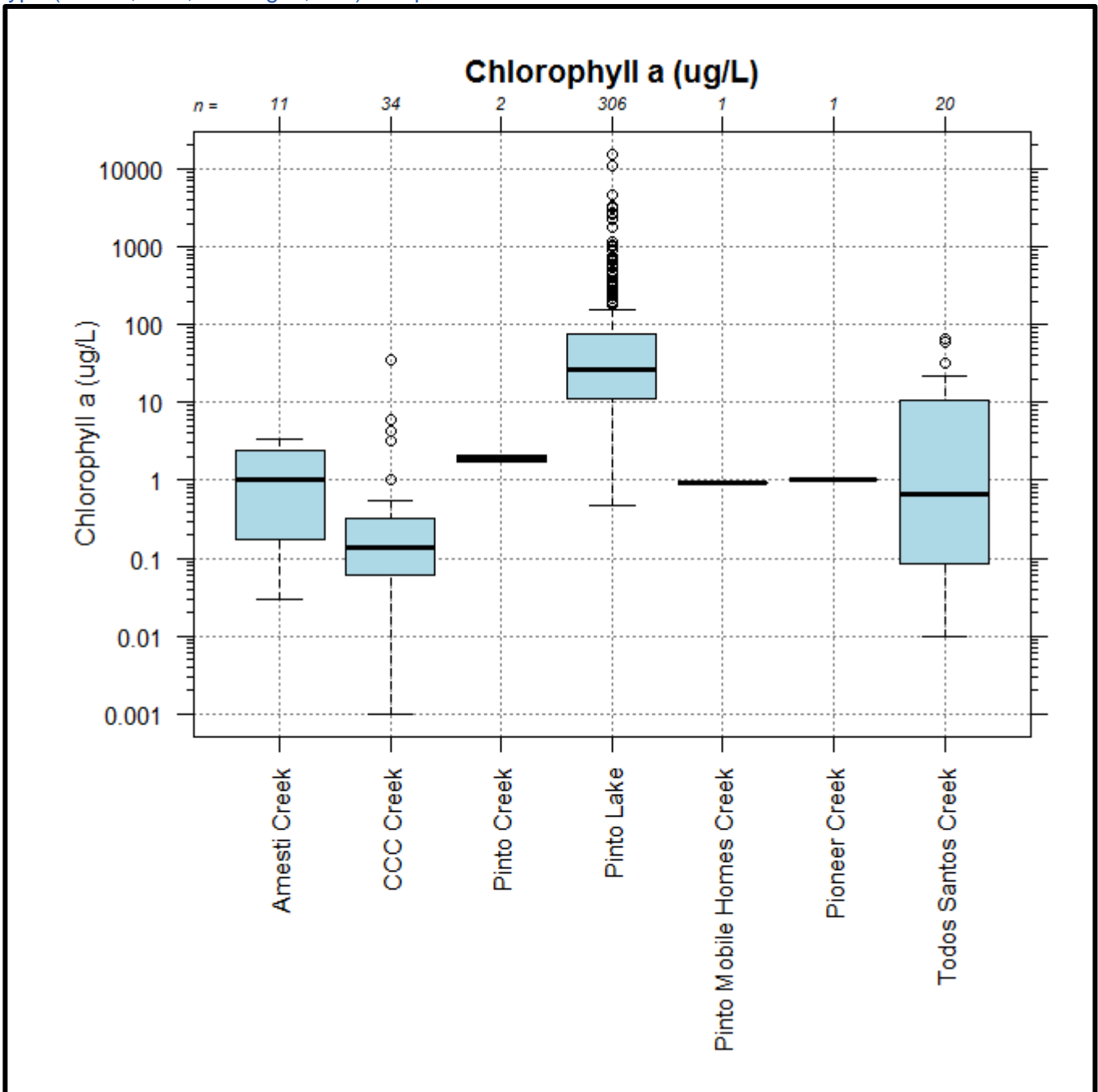
Figure 4-20. Box and whiskers plot, chlorophyll a water quality data for each waterbody/surface water type (creeks, lake, drainages, etc.) sampled.
