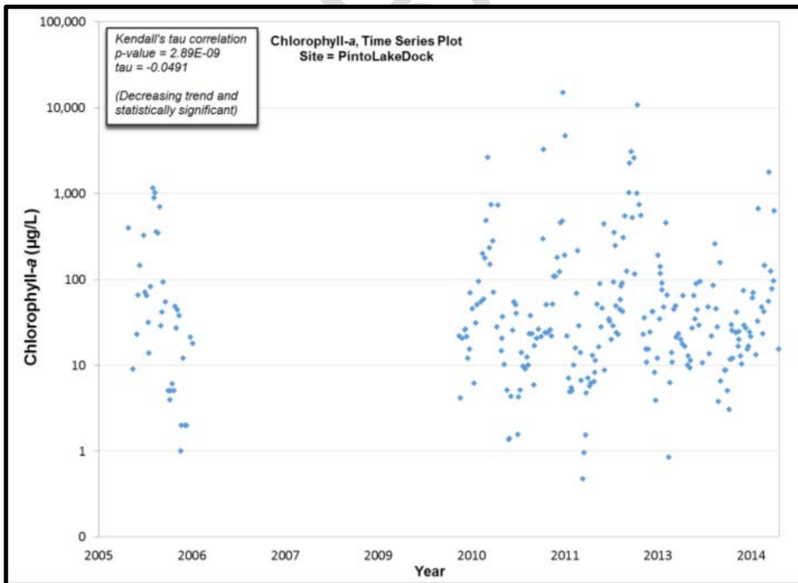
Figure 4-14. Temporal variations in total chlorophyll a concentrations at the Pinto Lake dock, April 2010 to October 2016.
