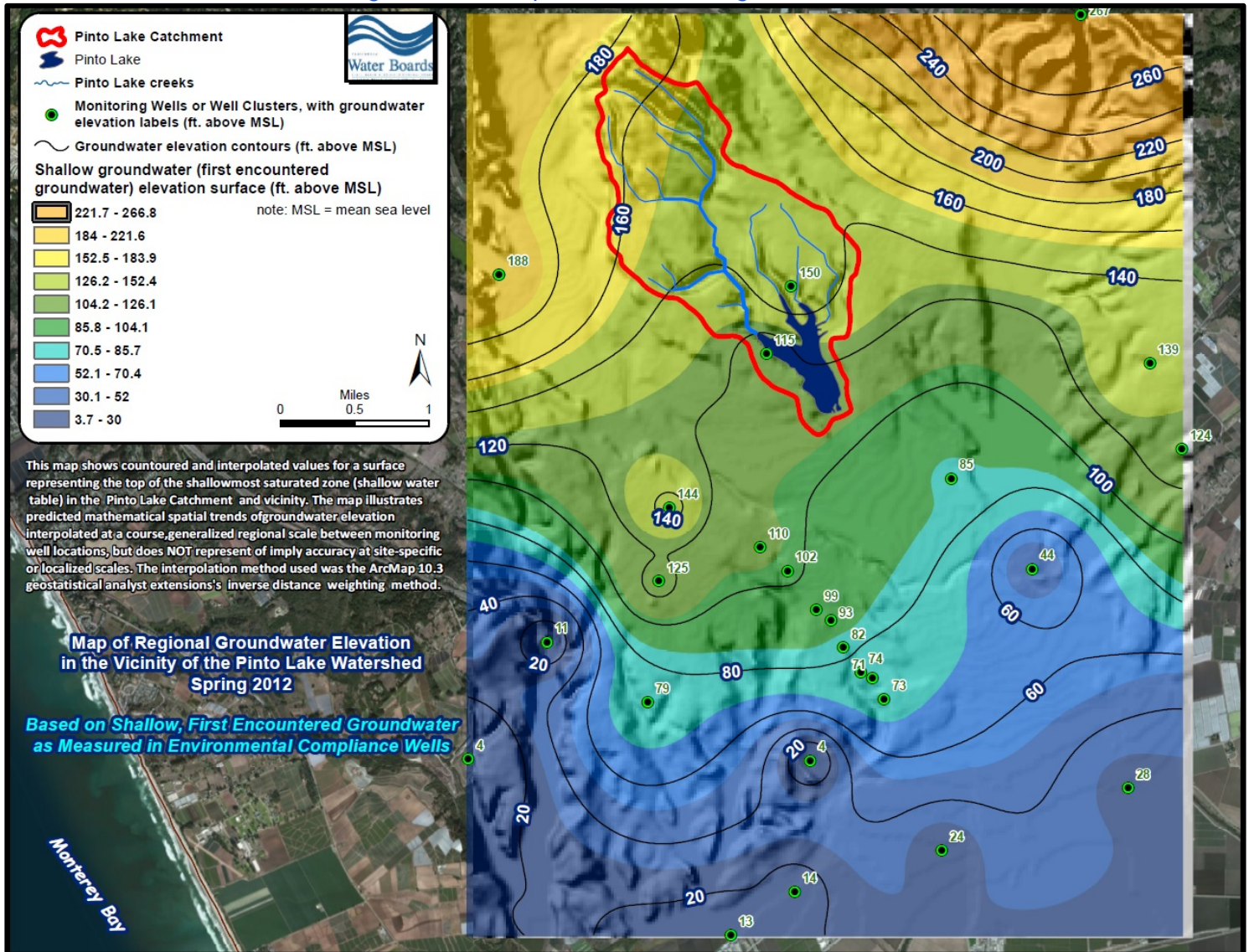
Figure 2-29. Map of groundwater elevation Spring 2012, Pinto Lake catchment and vicinity, on the basis of shallow, first-encountered groundwater reported in monitoring well data.
