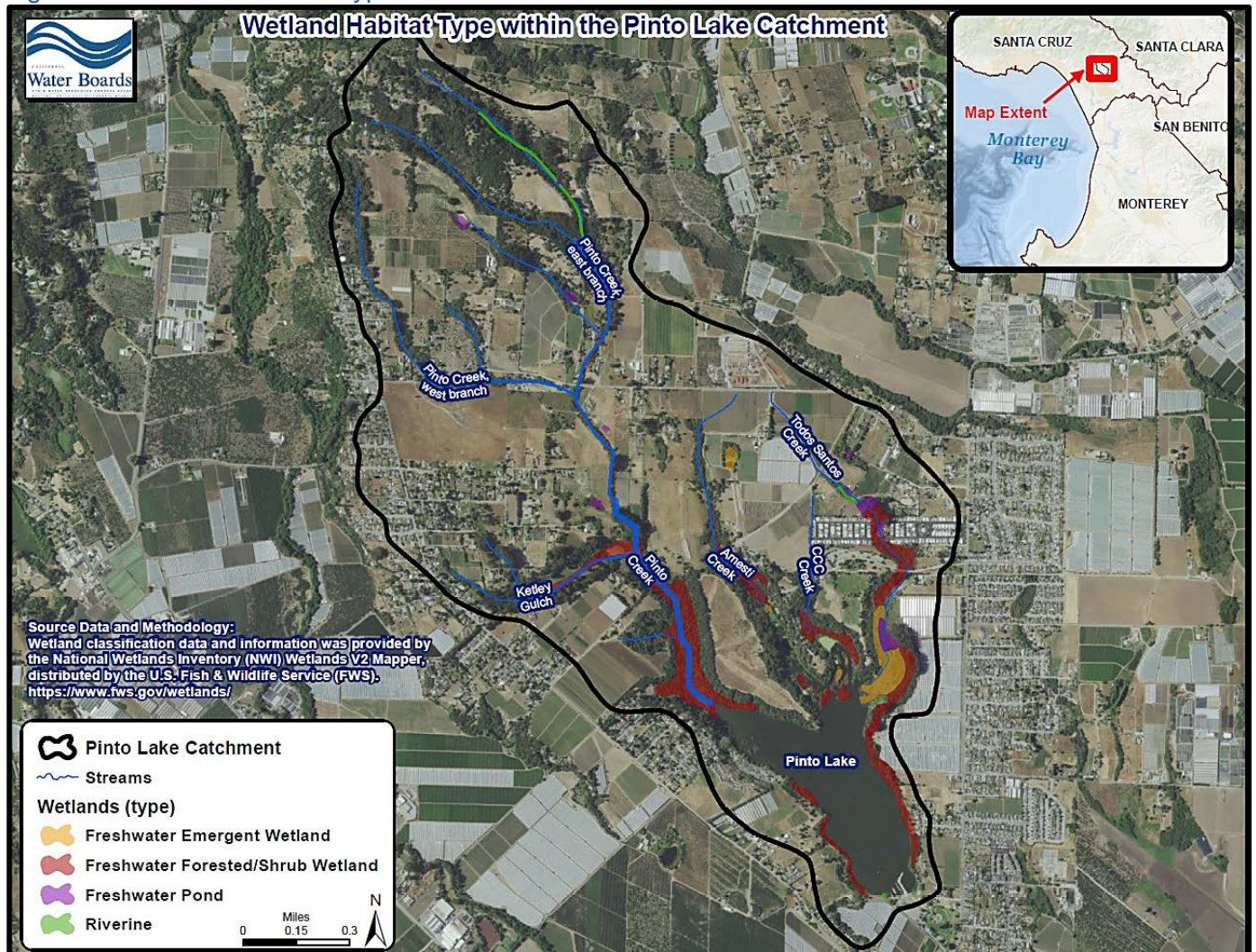
Figure 2-13. Wetland habitat types in the Pinto Lake catchment.
