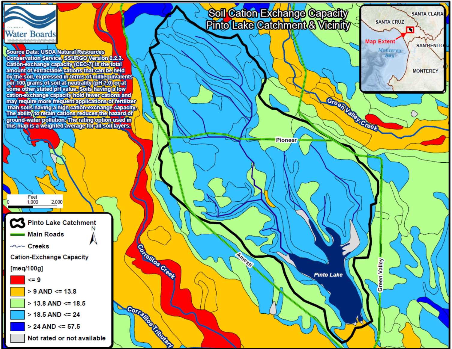
Figure 2-44. Map of soil cation exchange capacity, Pinto Lake catchment and vicinity.
