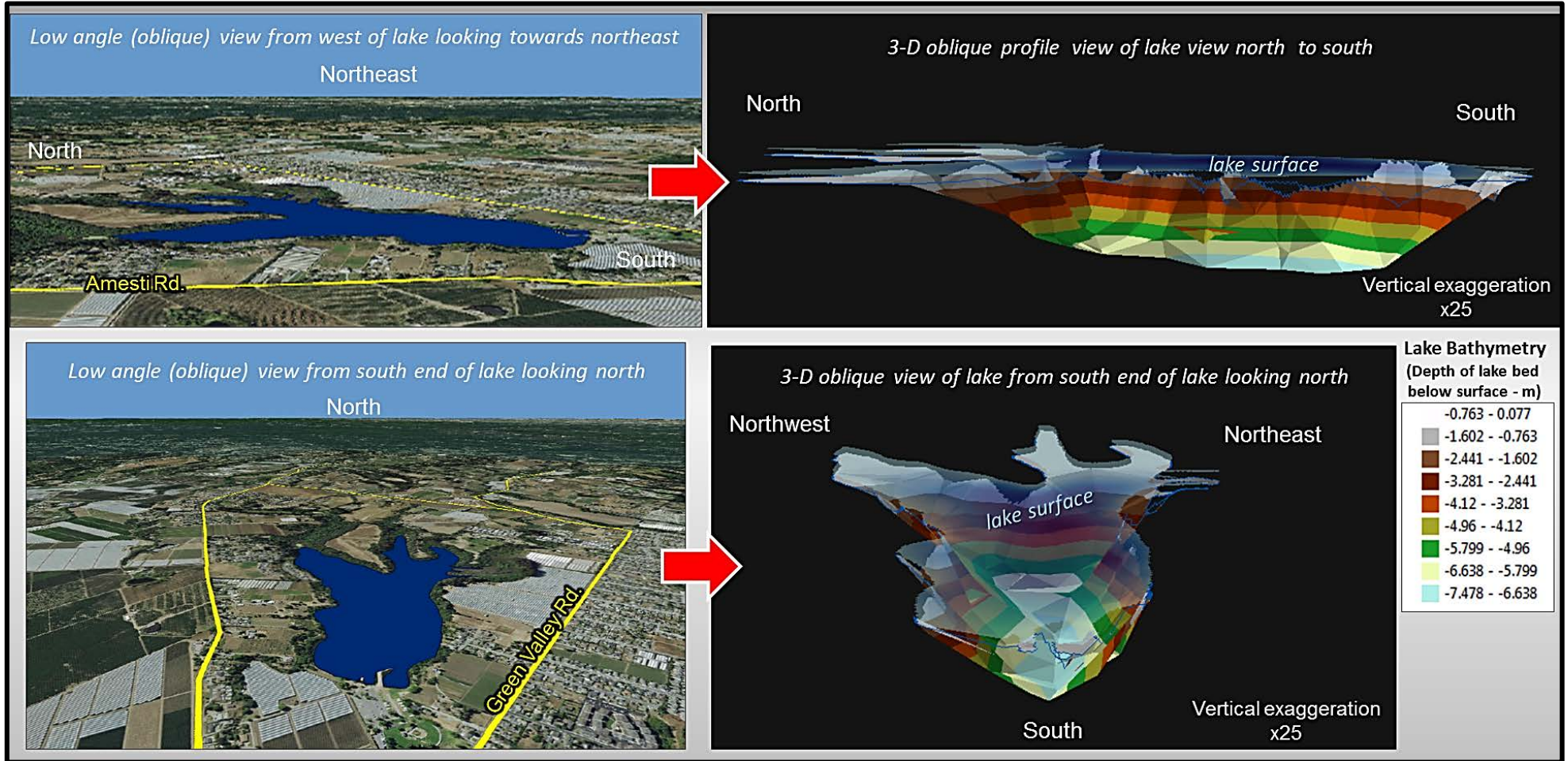
Figure 2-16. Low angle (oblique) aerial views and corresponding 3-dimensional bathymetric models of Pinto Lake.
