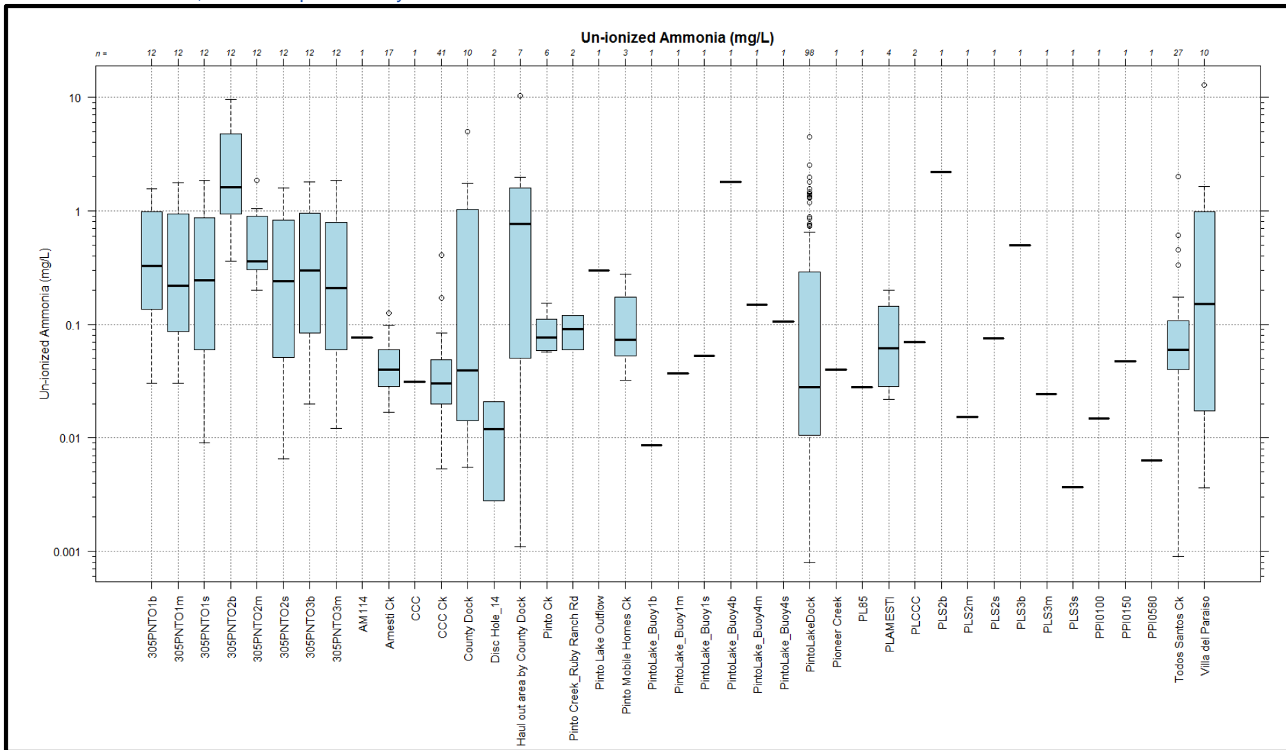
Figure 4-15. Box and whiskers plot, un-ionized ammonia water quality data for all surface water quality monitoring sampling sites within the Pinto Lake catchment, ordered alphabetically.
