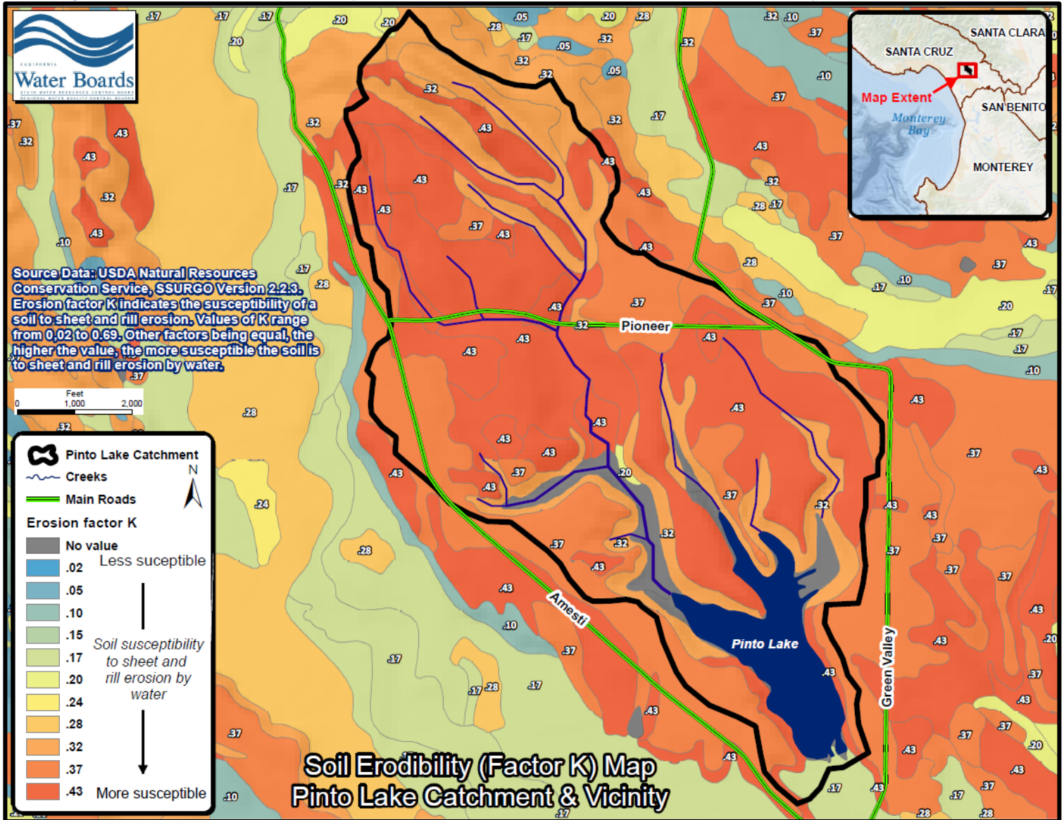
Figure 2-43. Map of soil erodibility (K factor) in the Pinto Lake catchment and vicinity.
