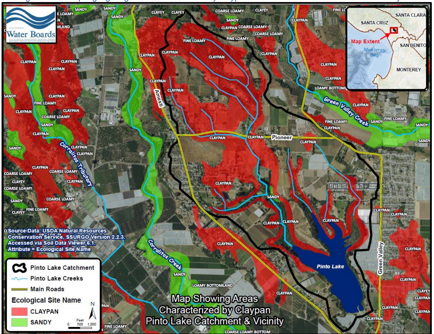
Figure 2-45. Map highlighting areas characterized by claypan in the Pinto Lake catchment and vicinity.
