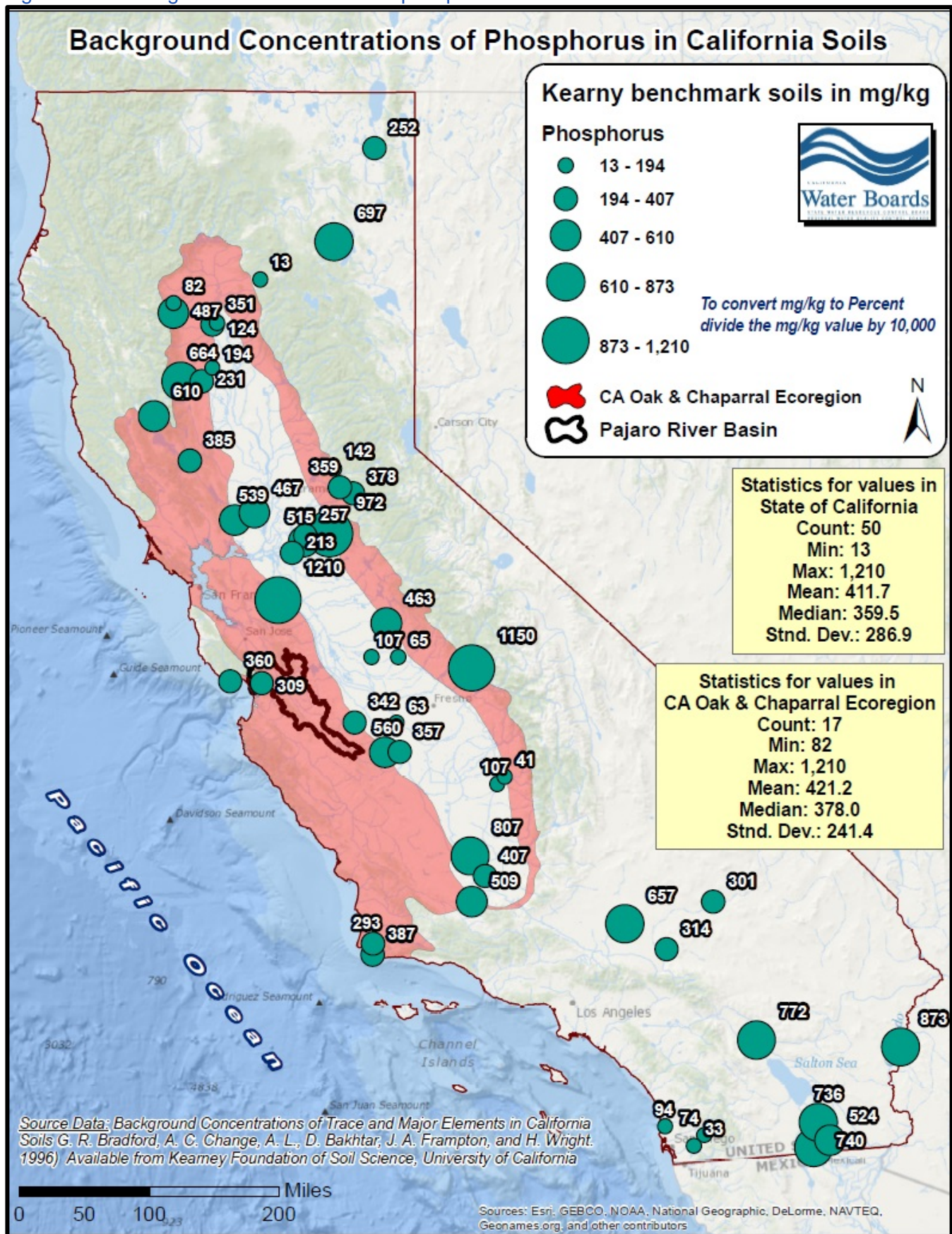
Figure 2-47. Background concentrations of phosphorus in California soils.
