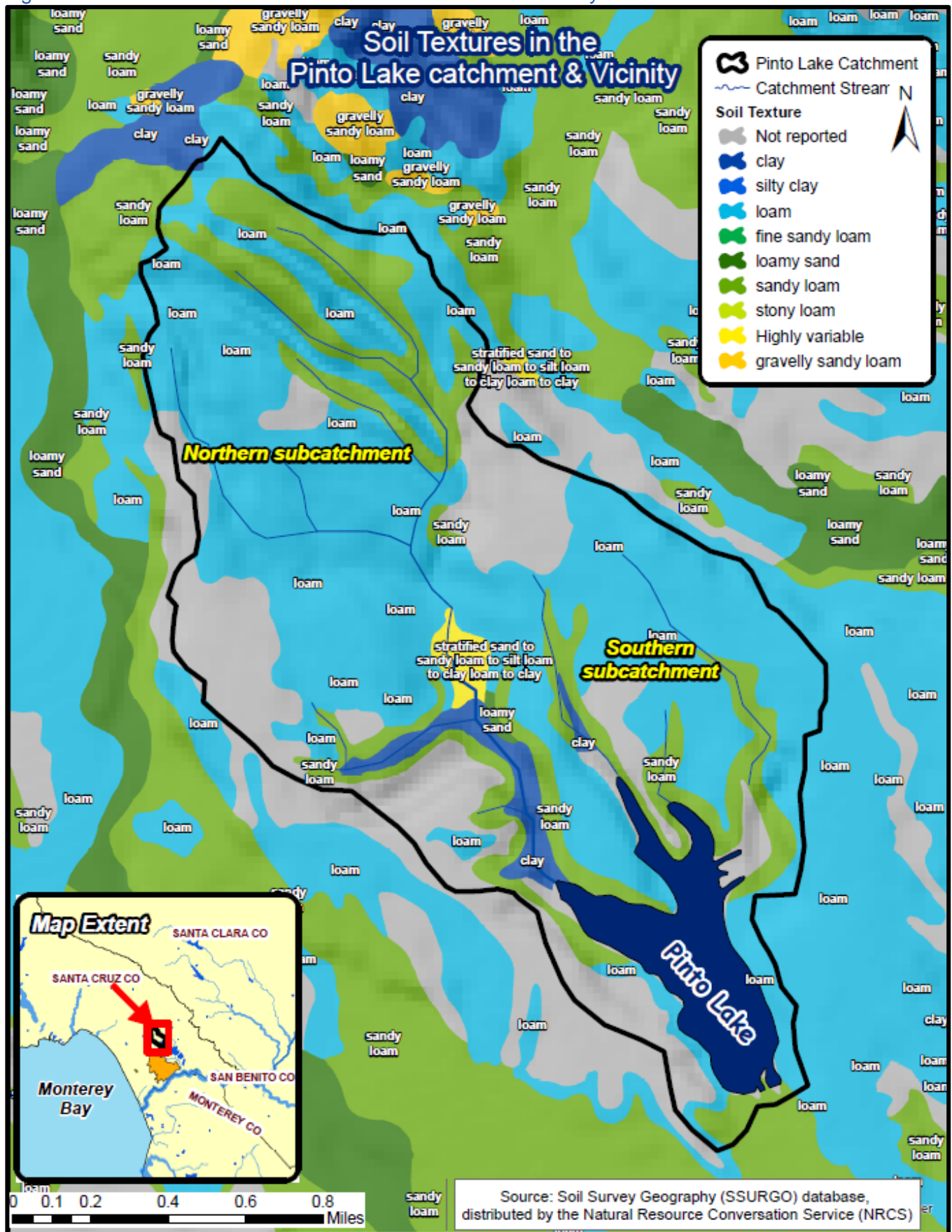
Figure 2-40. Soil textures in the Pinto Lake catchment and vicinity.
