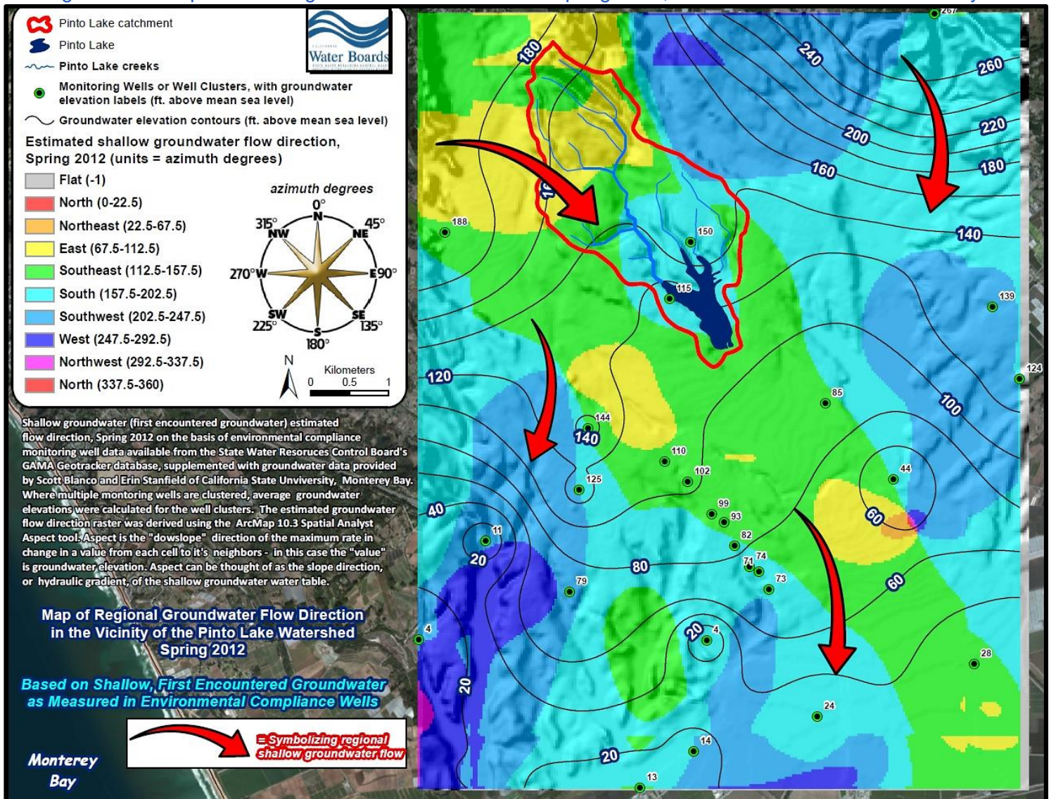
Figure 2-30. Map of shallow groundwater flow direction Spring 2012, Pinto Lake catchment and vicinity.
