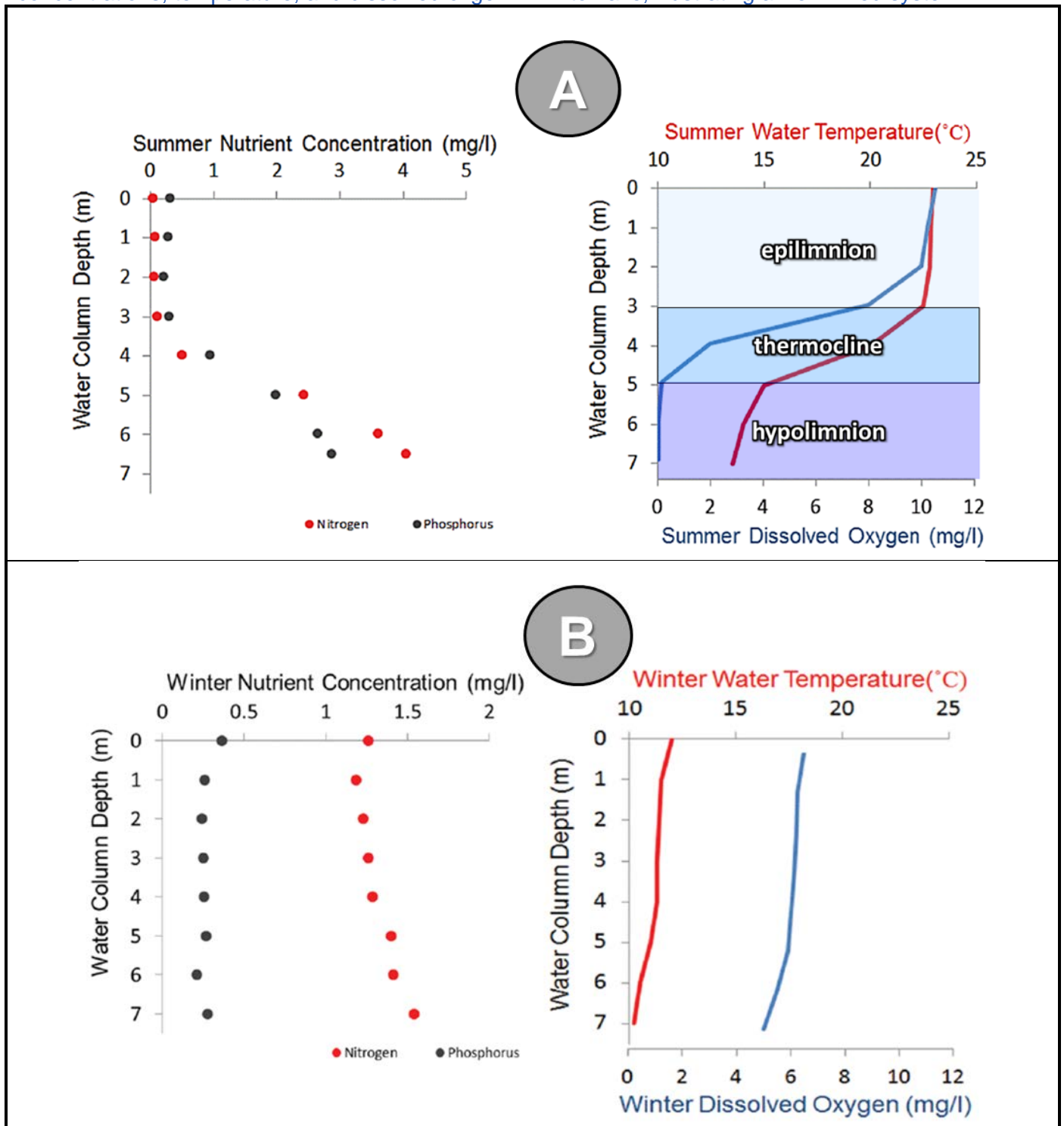
Figure 4-21. Figure from CSUMB and Resource Conservation District of Santa Cruz County, 2013. (A) Summer nutrient concentrations, temperature, and dissolved oxygen illustrating thermal stratification of lake waters and nutrient-enrichment of deep waters (hypolimnion); and (B) Winter nutrient concentrations, temperature, and dissolved oxygen in Pinto Lake, illustrating a well mixed system.
