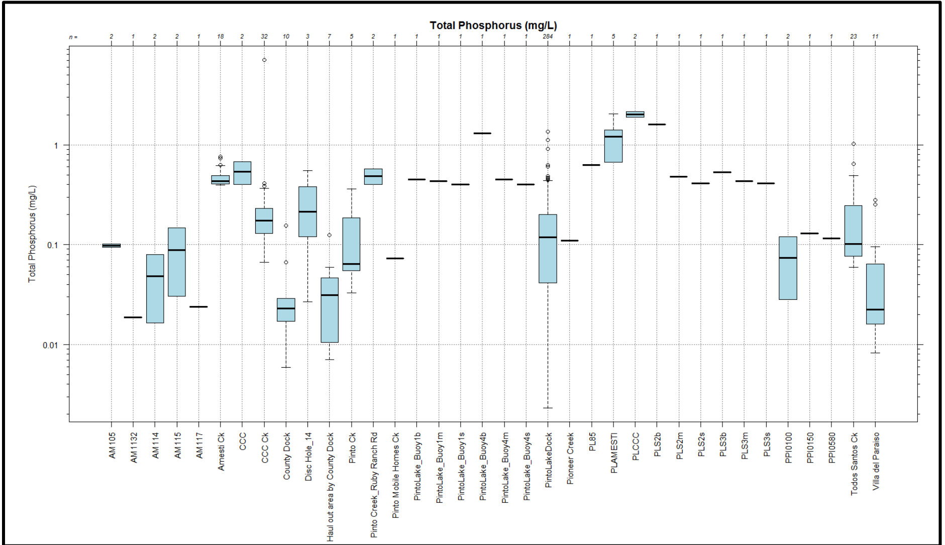
Figure 4-10. Box and whiskers plots, total phosphorus water quality data for all surface water quality monitoring sampling sites within the Pinto Lake catchment, ordered alphabetically. Some of the highest measured concentrations were recorded for tributary monitoring sites located in Amesti Creek (e.g. PLAMESTI), and CCC Creek (e.g. PLCCC). The maximum concentration recorded was 7.045 mg/L at CCC Ck.
