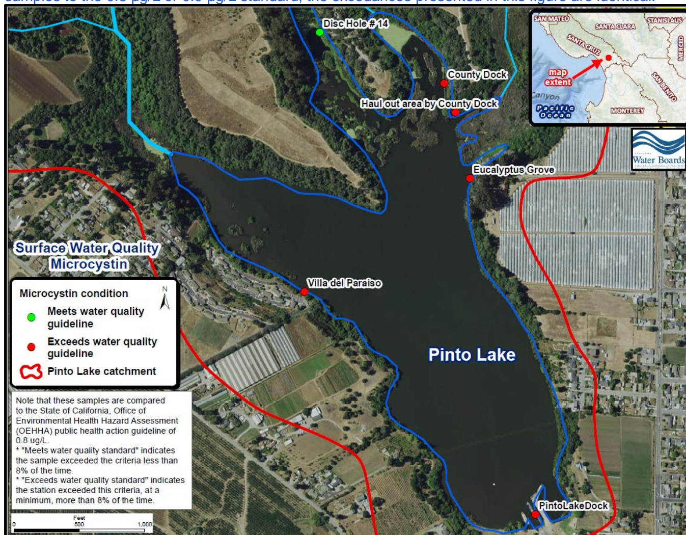
Figure 4-38. Microcystin water quality standards attainment assessment of the water contact recreation (REC-1) and wildlife habitat (WILD) beneficial uses. Note that we compared the WILD beneficial use to a microcystin concentration of 0.9 µg/L (REC-1 is using 0.8 µg/L microcystin). Whether we compared the samples to the 0.8 µg/L or 0.9 µg/L standard, the exceedances presented in this figure are identical.
