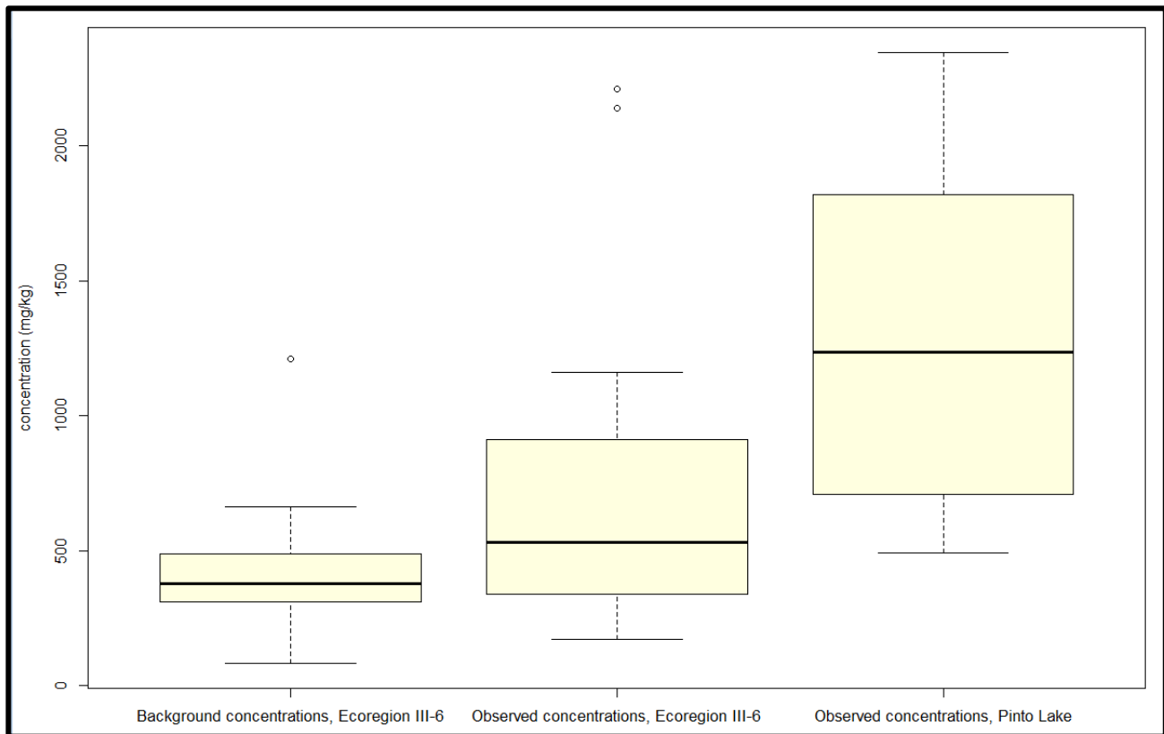
Figure 2-38. Box plot illustrating phosphorus concentration variation in soils of USEPA Ecoregion III-6 (central California oak and chaparral ecoregion) as compared to phosphorus concentrations in the Pinto Lake catchment sediments. Summary statistics for information in this boxplot were previously presented in Table 2-18.
