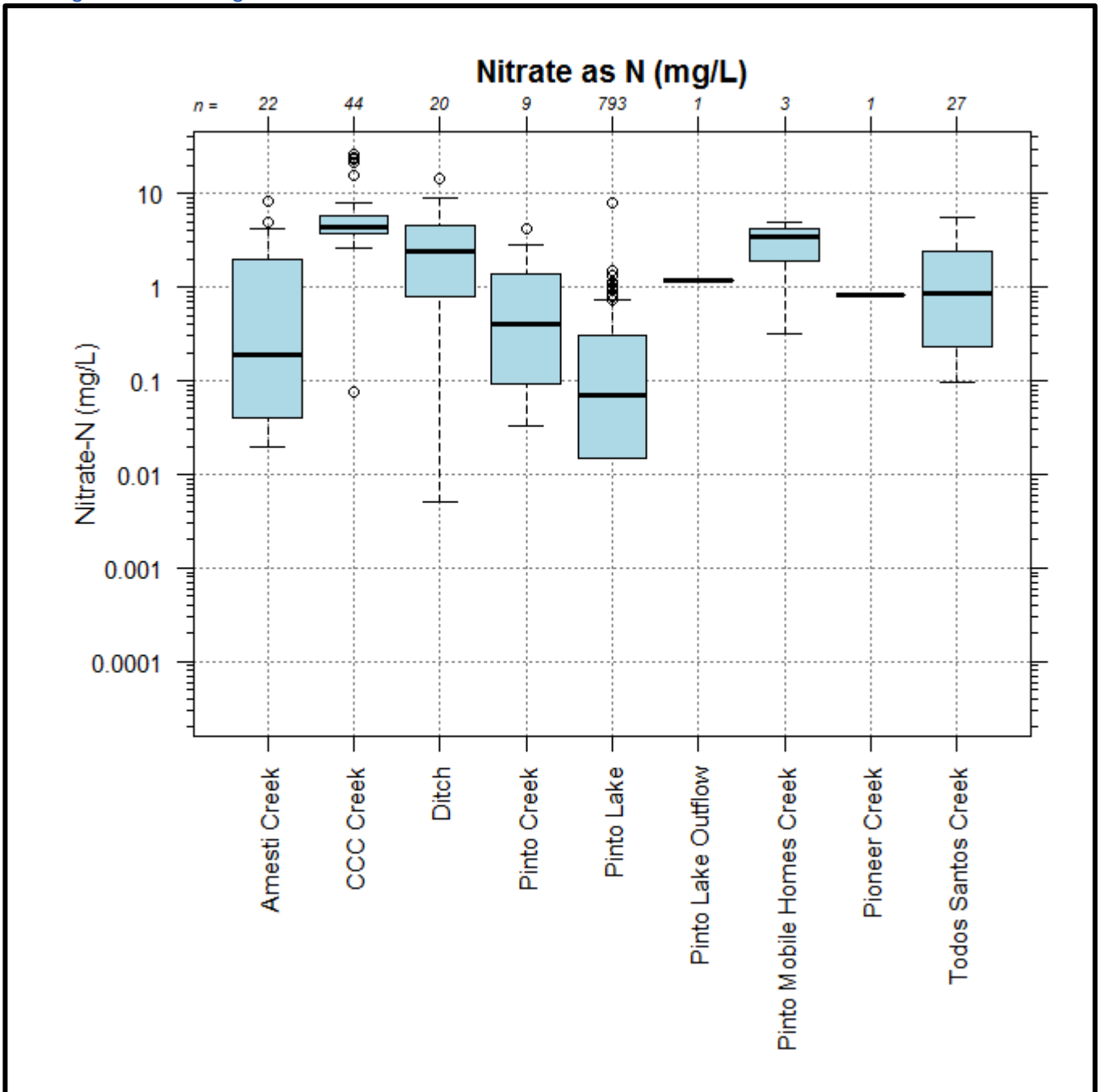
Figure 4-14. Box and whiskers plot, nitrate as N water quality data, for each waterbody/surface water type (creeks, lake, drainages, etc.) sampled. For reference, the nitrate as N water quality standard for drinking water is 10 mg/L.
