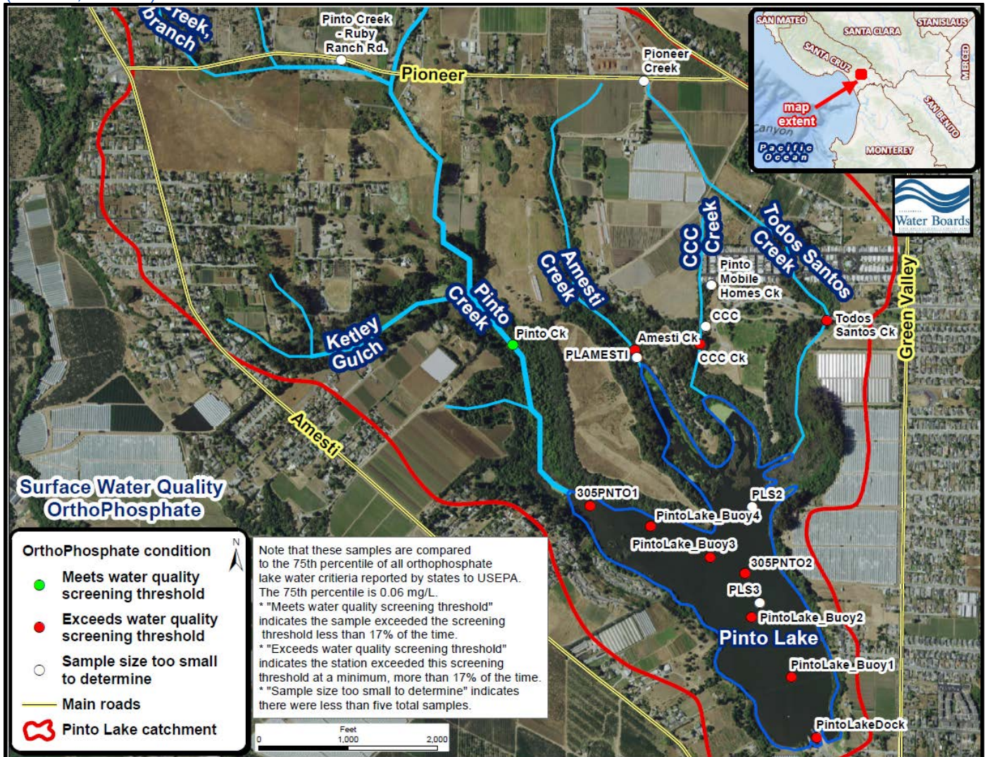
Figure 4-35. OrthoPhosphate water quality standards attainment assessment of the aquatic habitat (WARM, SPWN) beneficial uses.
