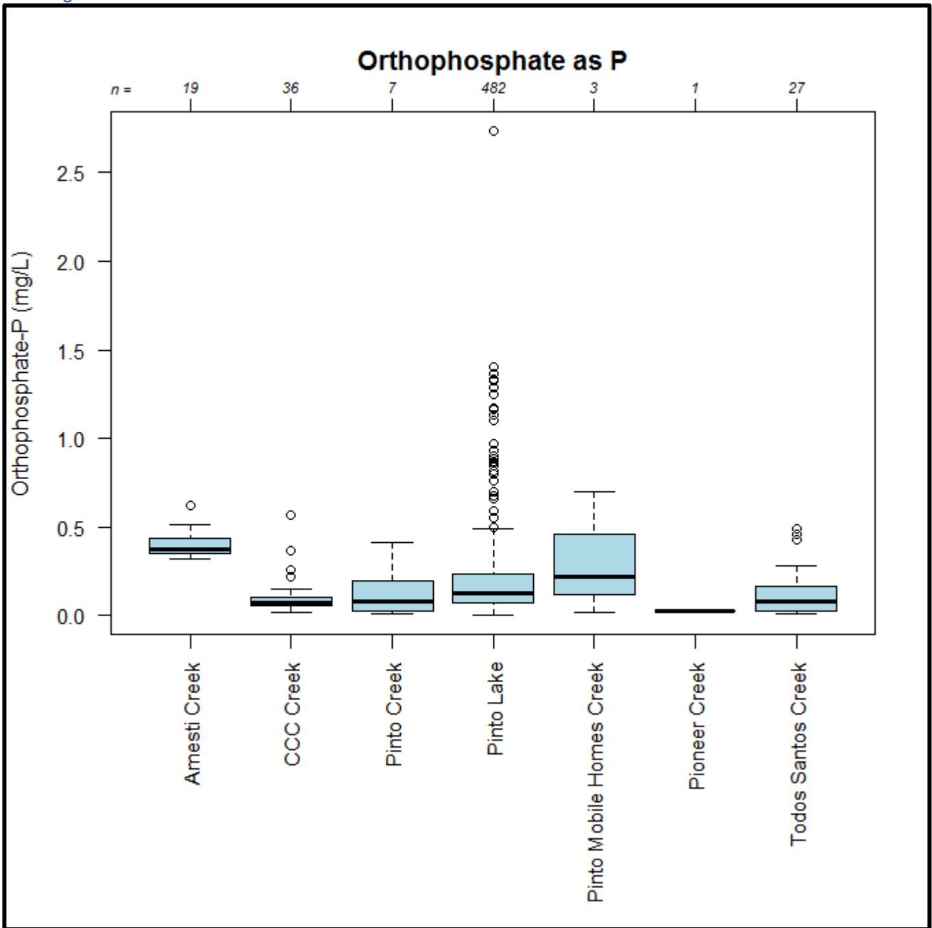
Figure 4-18. Box and whiskers plot, orthophosphate as P water quality data for each waterbody/surface water type (creeks, lake, drainages, etc.) sampled. For reference, the orthophosphate as P guideline is 0.06 mg/L.
