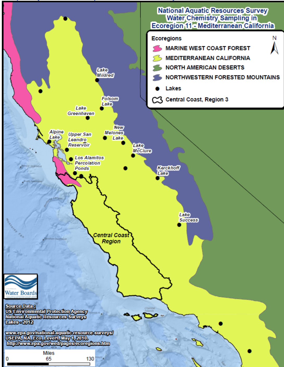
Figure 4-25. Map of USEPA nutrient Ecoregion level 1, sublevel 11 (Mediterranean California) and lakes sampled by the National Aquatic Resources Survey in 2012.
