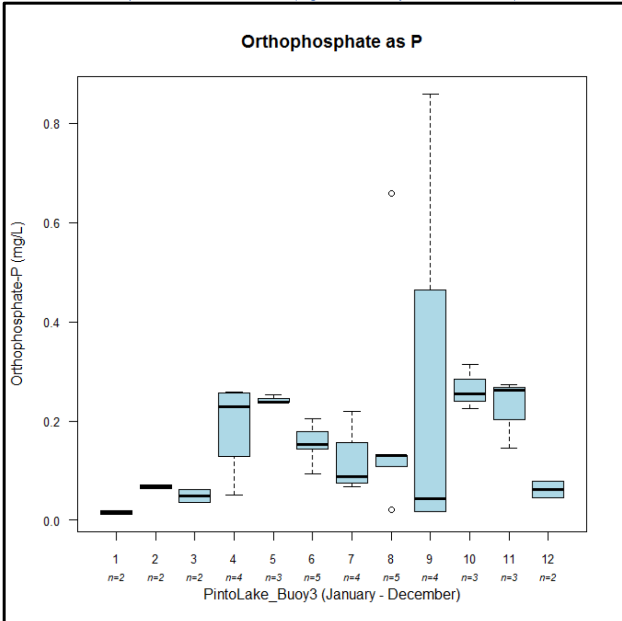
Figure 4-40. Box and whisker plot of orthophosphate as P (mg/L) values from Pinto Lake catchment site, PintoLake_Buoy3. Values plotted per month to show seasonal difference in phosphate values. Numbers on the x-axis correspond to calendar months (e.g., 1 = January, 12 = December).
