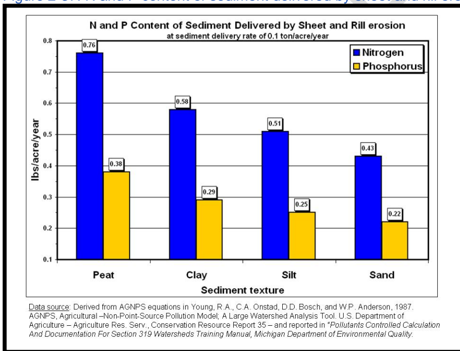
Figure 2-37. N and P content of sediment delivered by sheet and rill erosion.
