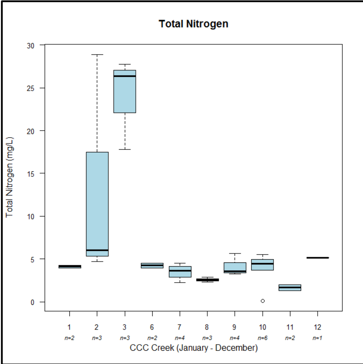
Figure 4-17. Box and whisker plot of total nitrogen (mg/L) values from Pinto Lake catchment site, CCC Creek. Values plotted per month to show seasonal difference in nitrate values. Numbers on the x-axis correspond to calendar months (e.g., 1 = January, 12 = December).
