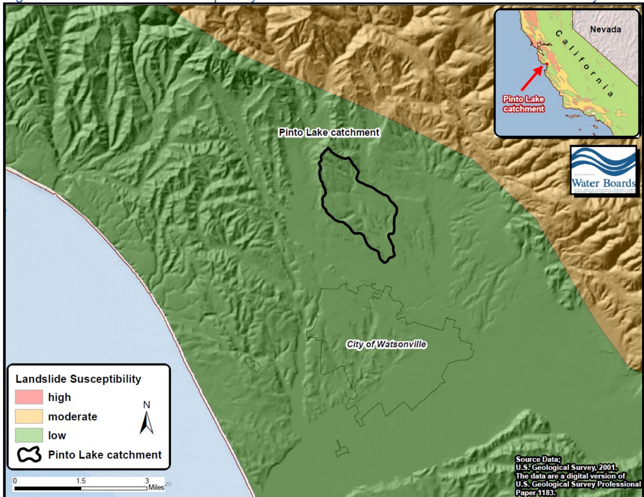
Figure 6. Landslide risks – susceptibility to landslides in the Pinto Lake catchment and vicinity.
