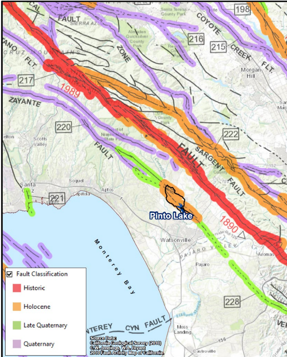
Figure 8. Alquist-Priolo earthquake fault zone map, Pinto Lake and vicinity.
