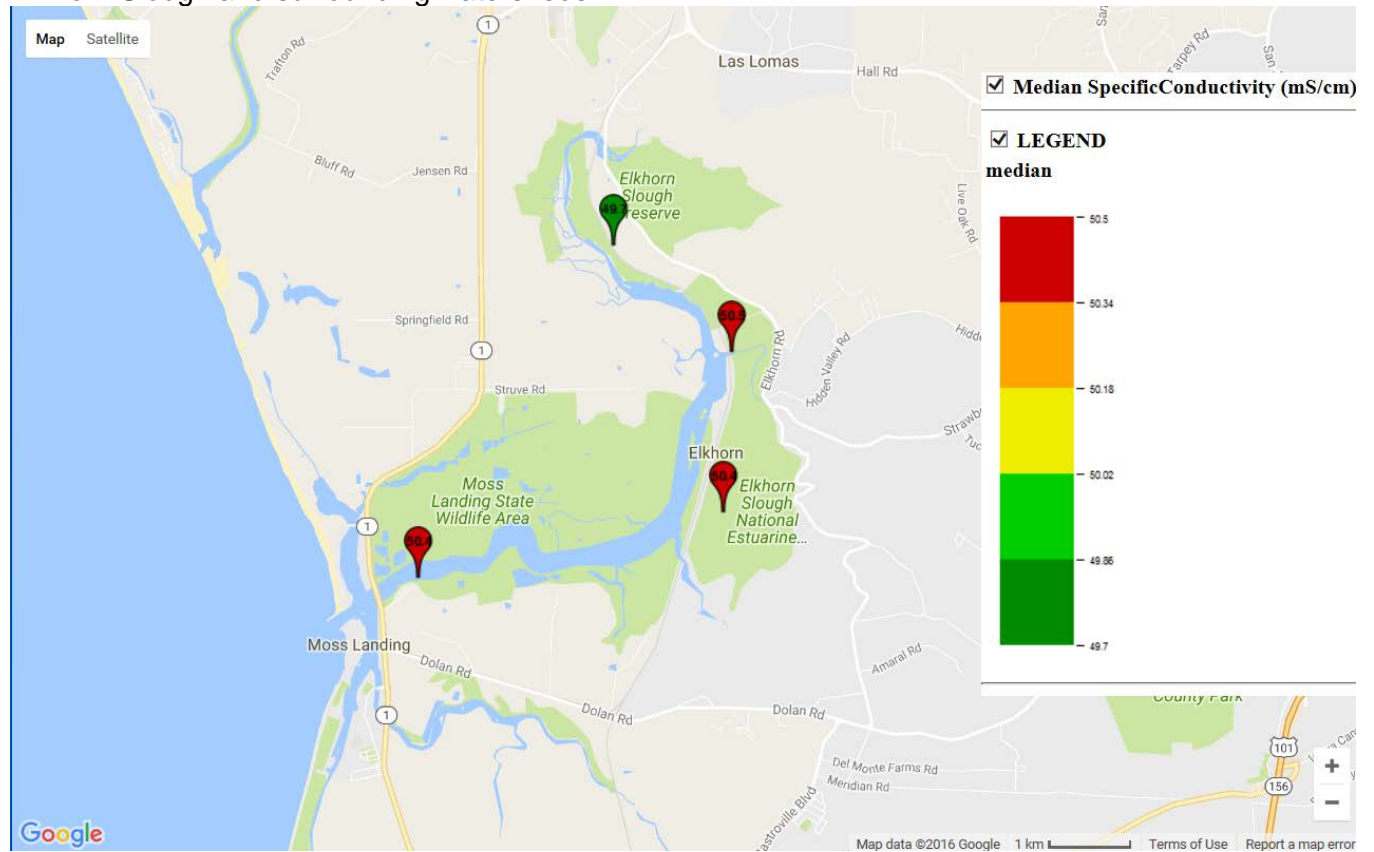
Figure 5-37. Median surface water concentration map of specific conductivity (mS/cm) in the Elkhorn Slough and surrounding watersheds.
