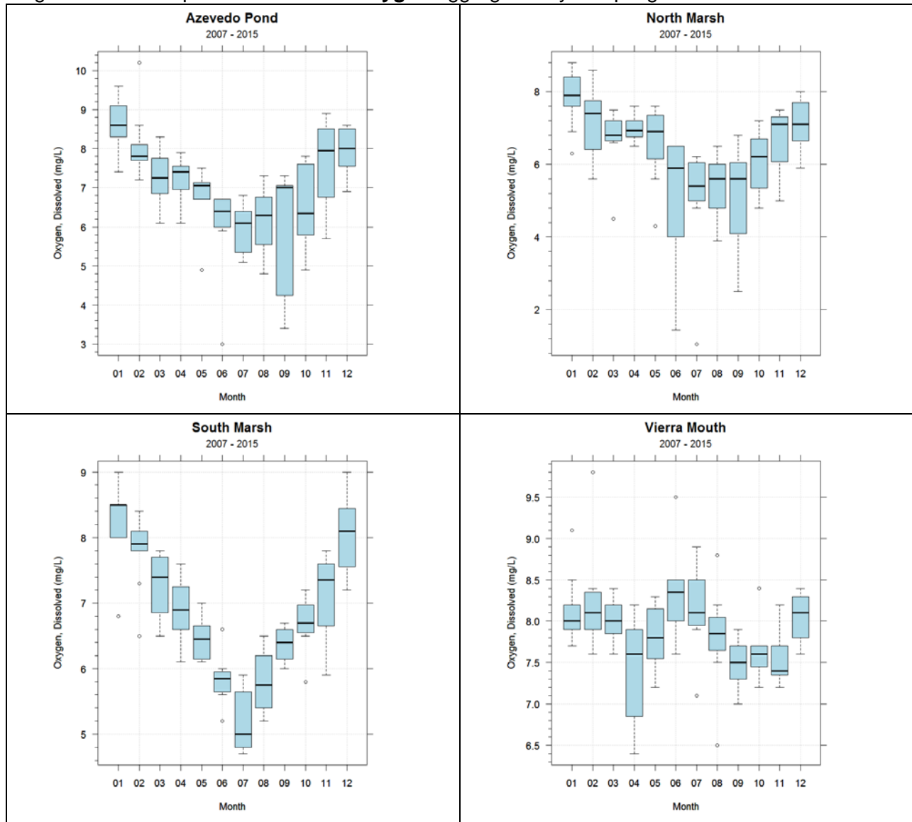
Figure 5-46. Box plots of dissolved oxygen aggregated by sampling month.
