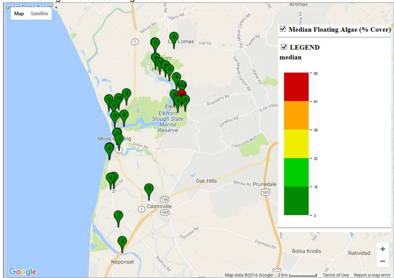
Figure 5-35. Median surface water concentration map of floating algae (% cover) in the Elkhorn Slough and surrounding watersheds.
