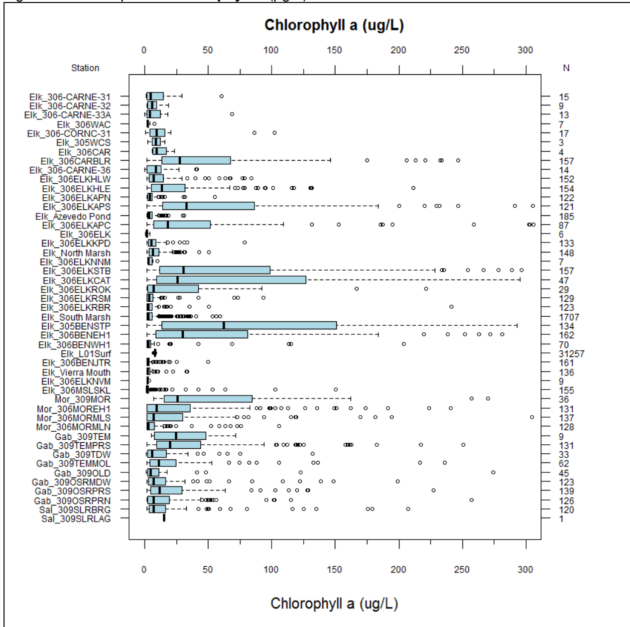
Figure 5-10. Box plots of chlorophyll-a (µg/L) concentrations.
