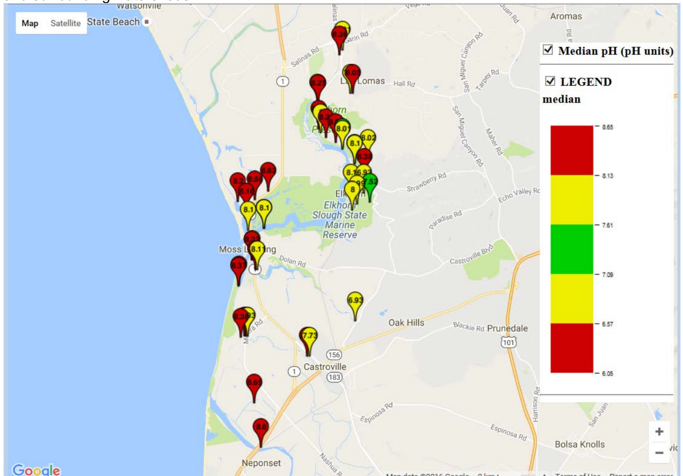
Figure 5-26. Median surface water concentration map of pH (pH units) in the Elkhorn Slough and surrounding watersheds.
