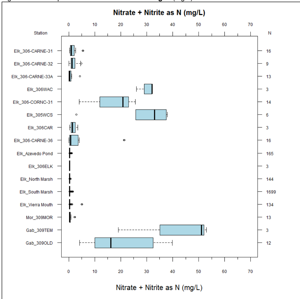
Figure 5-14. Box plots of nitrate + nitrite as nitrogen (mg/L) concentrations.
