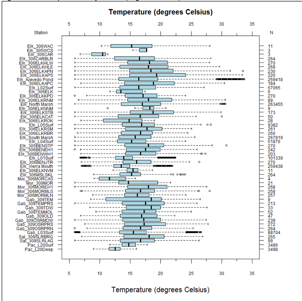
Figure 5-22. Box plots of temperature (degrees Celsius).
