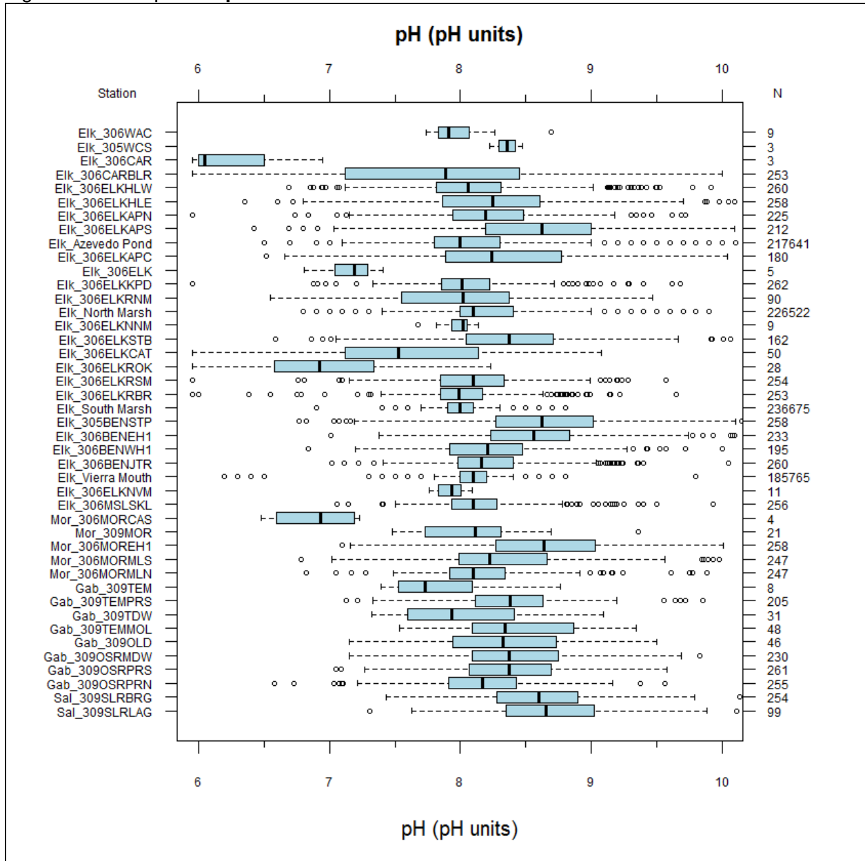
Figure 5-9. Box plots of pH concentrations.
