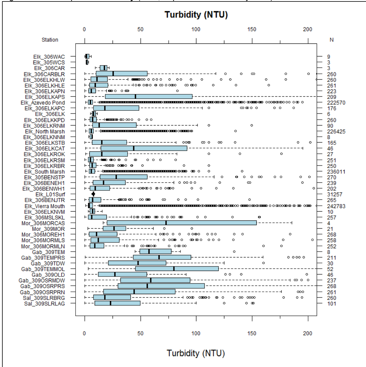
Figure 5-23. Box plots of turbidity (NTU, nephelometric turbidity units) concentrations.
