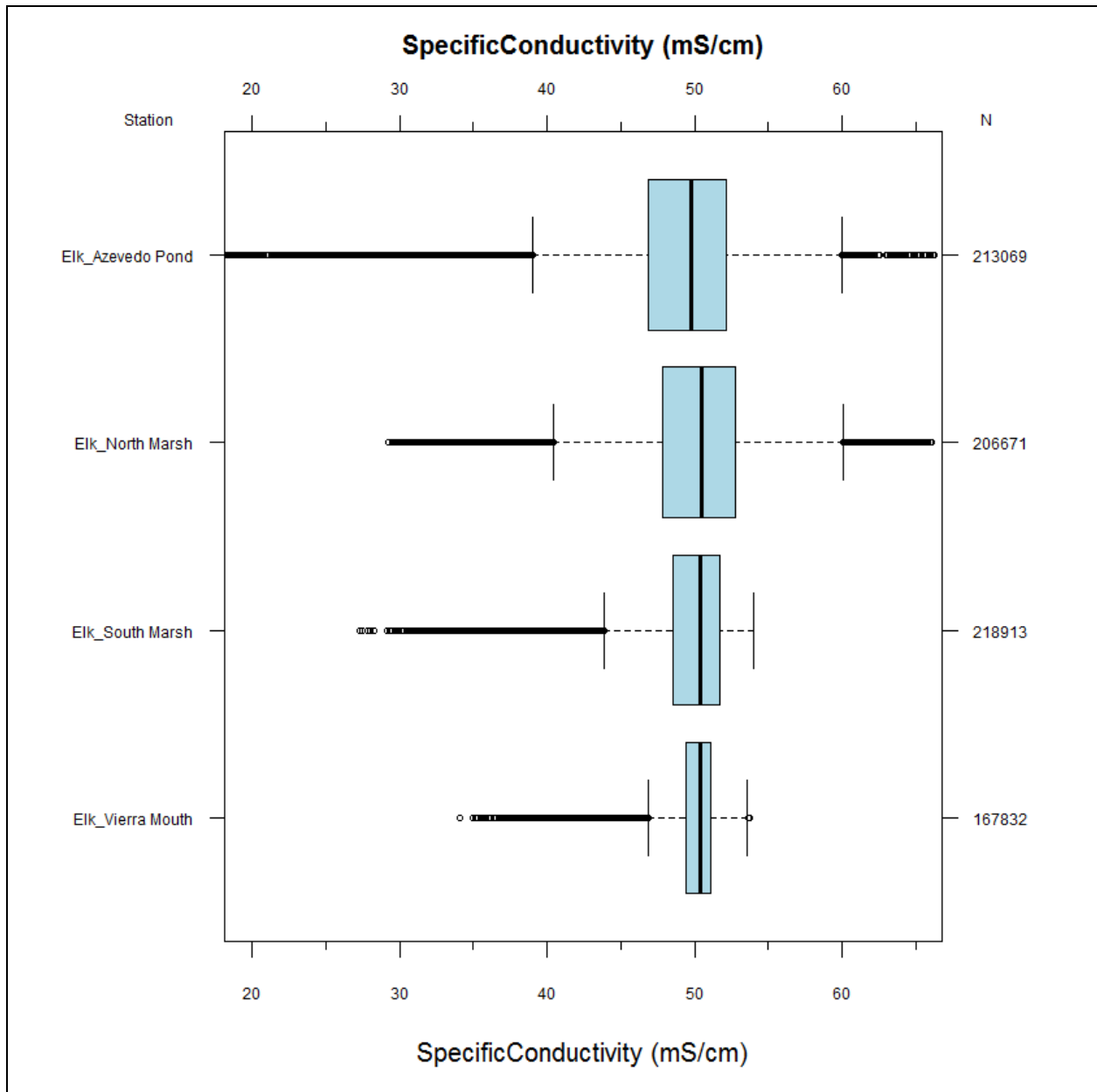
Figure 5-21. Box plots of specific conductivity (mS/cm, milli-Siemens per centimeter) concentrations.
