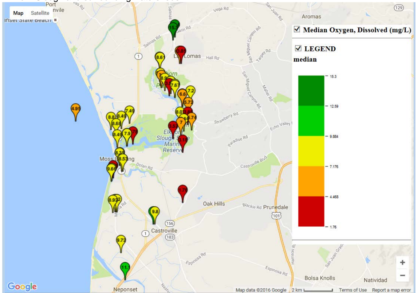
Figure 5-24. Median surface water concentration map of dissolved oxygen (mg/L) in the Elkhorn Slough and surrounding watersheds.
