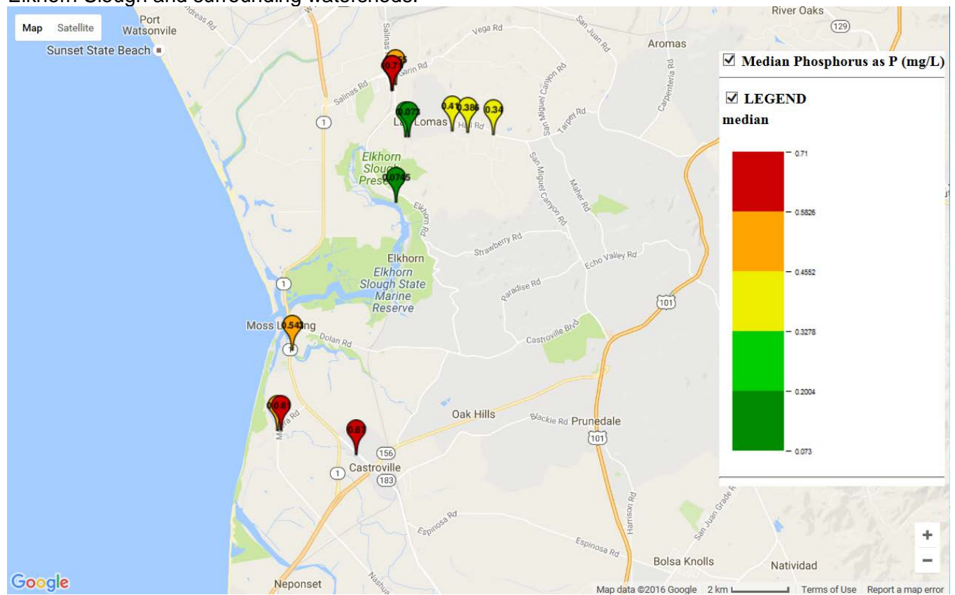
Figure 5-34. Median surface water concentration map of total phosphorous (mg/L) in the Elkhorn Slough and surrounding watersheds.
