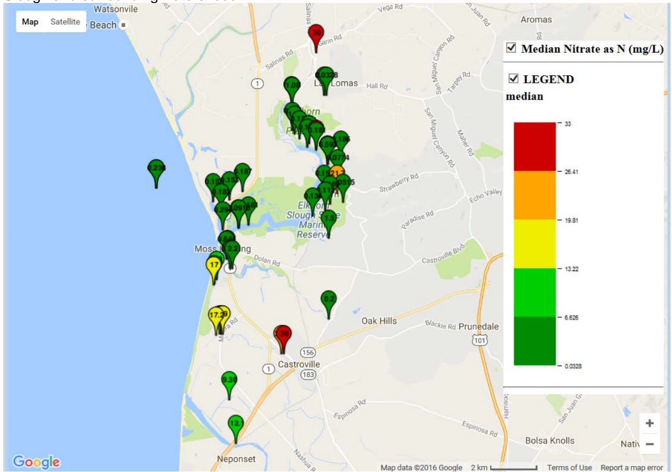
Figure 5-31. Median surface water concentration map of nitrate as N (mg/L) in the Elkhorn Slough and surrounding watersheds.
