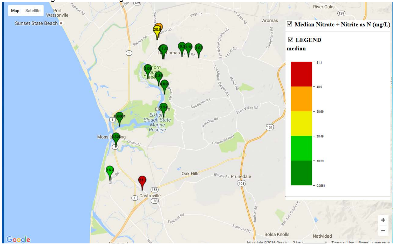
Figure 5-32. Median surface water concentration map of nitrate + nitrite as N (mg/L) in the Elkhorn Slough and surrounding watersheds.
