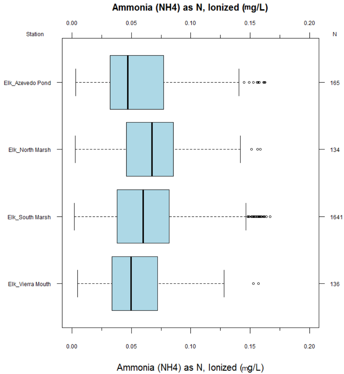
Figure 5-7. Box plots of ionized ammonia (NH 4 ) as nitrogen (mg/L) concentrations.
