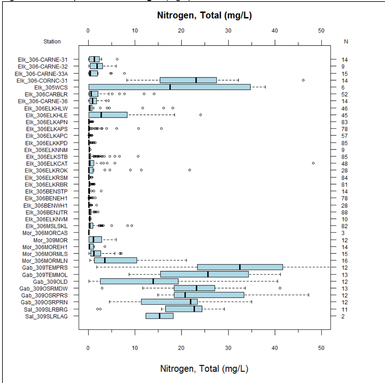
Figure 5-16. Box plots of total nitrogen (mg/L) concentrations.
