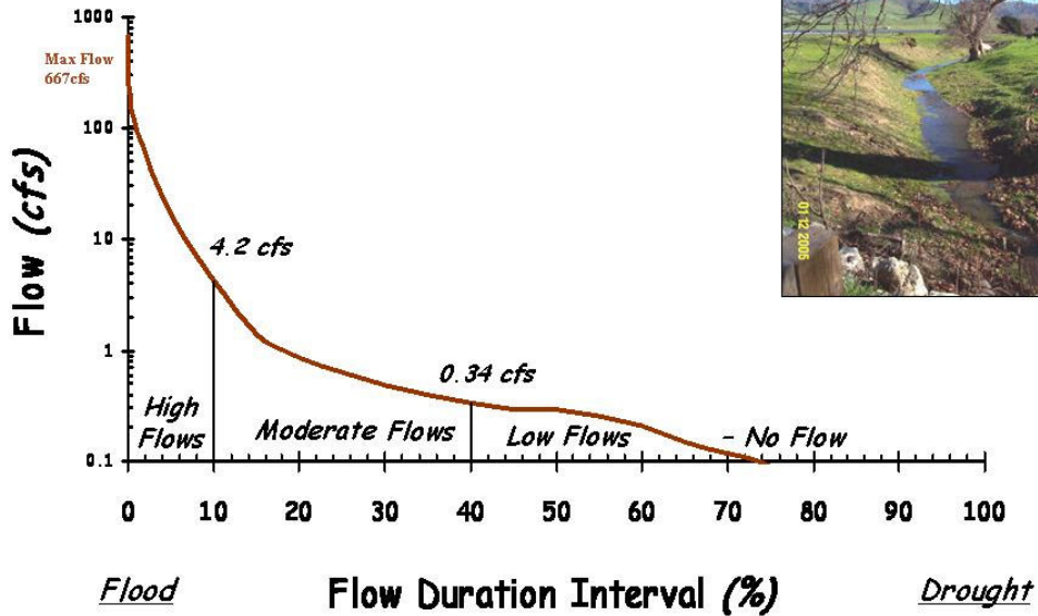
Alisal Creek, CA Flow Duration Curve for Site ALI-AIR
