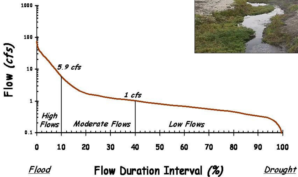
Blanco Drain, CA Flow Duration Curve for Site BLA-COO
