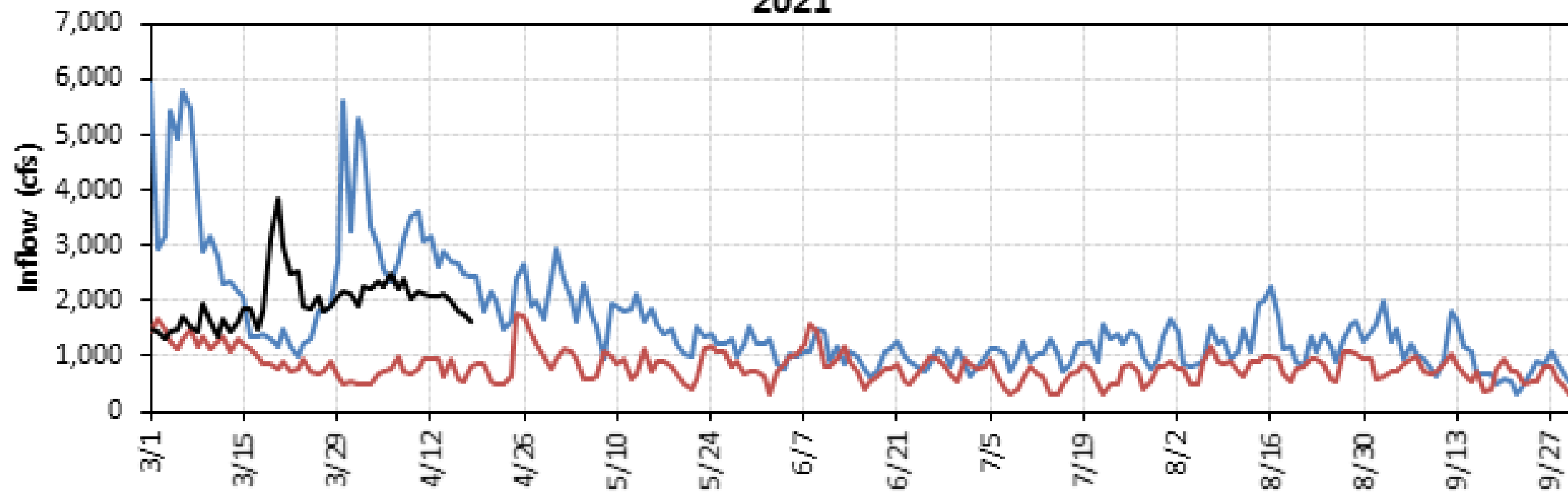
Comparison of Historical Daily Folsom Reservoir Inflow for 2014, 2015, and 2021
