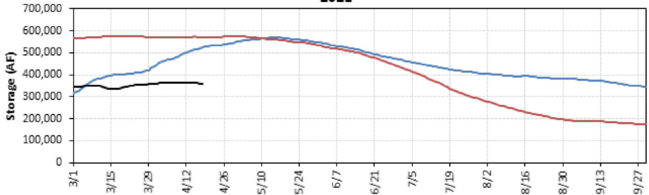
Comparison of Historical Daily Folsom Reservoir Storage for 2014, 2015, and 2021
