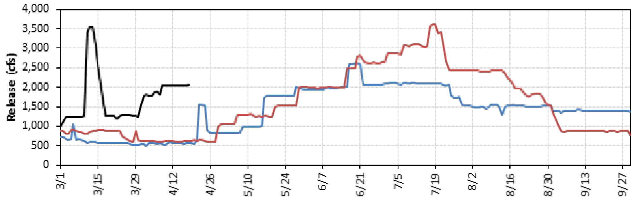
Comparison of Historical Daily Nimbus Dam Releases for 2014, 2015, and 2021
