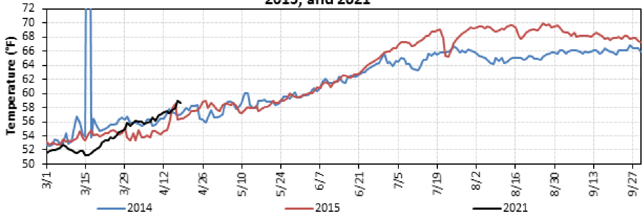
Comparison of Historical Daily Nimbus Dam Release Temperatures for 2014, 2015, and 2021
