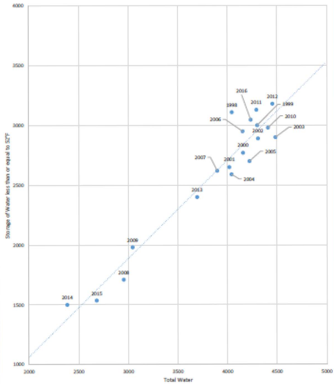
Shasta Lake end of April Water Volumes
