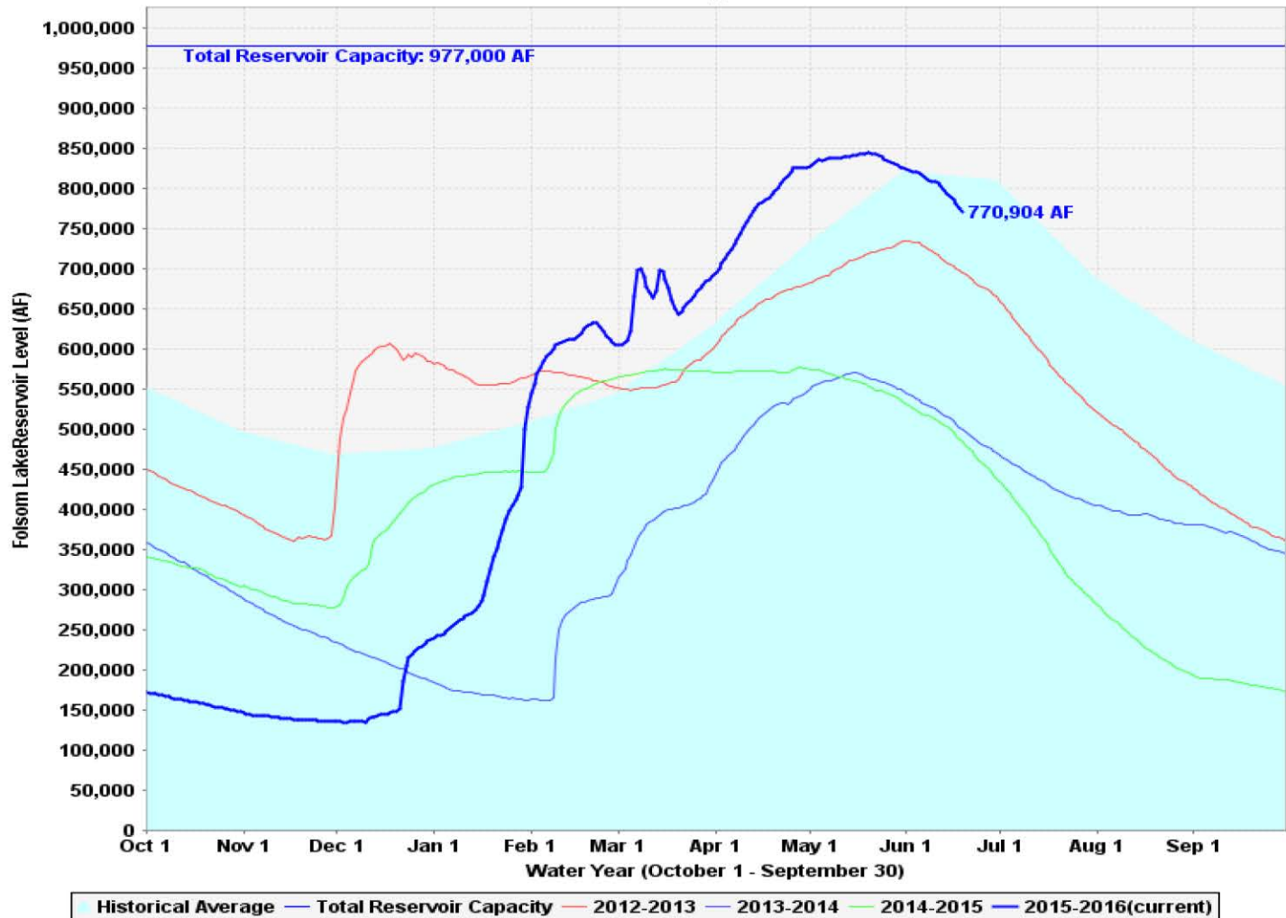
Folsom Lake Storage Levels
