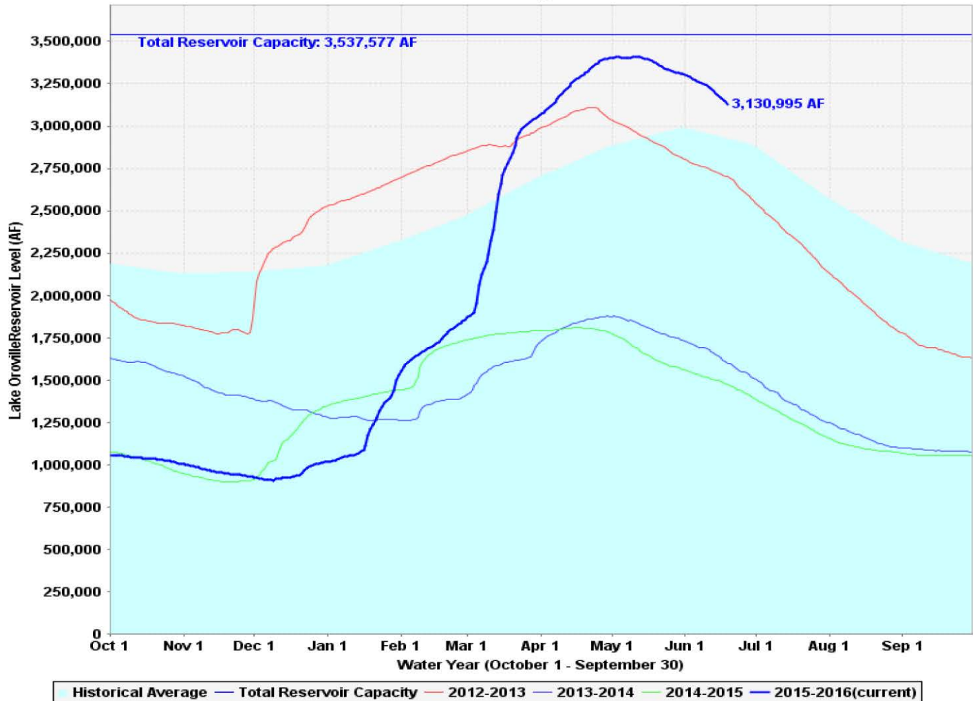
Lake Oroville Storage Levels
